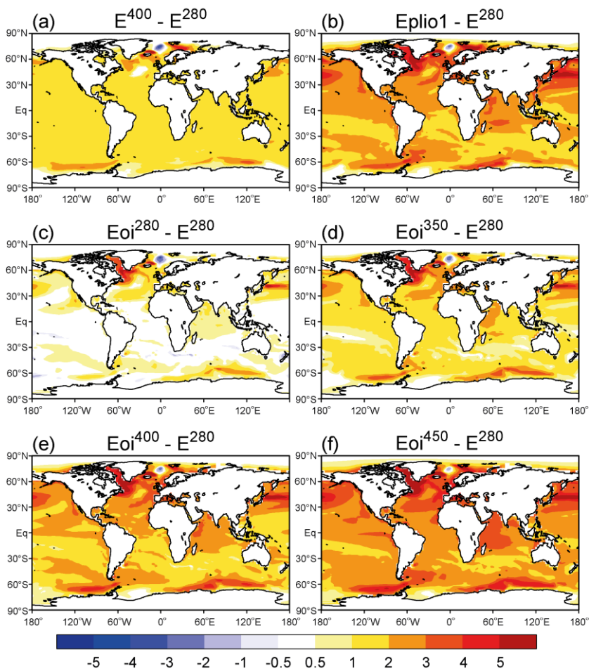
Figure 6: Annual mean sea surface temperature anomaly between six experiments and E 280 , the Pre-Industrial. For a comparison of PlioMIP1 and PlioMIP2, see (b) and (e). For the individual effects of CO 2 and Pliocene boundary conditions, see (a) and (c), respectively.
