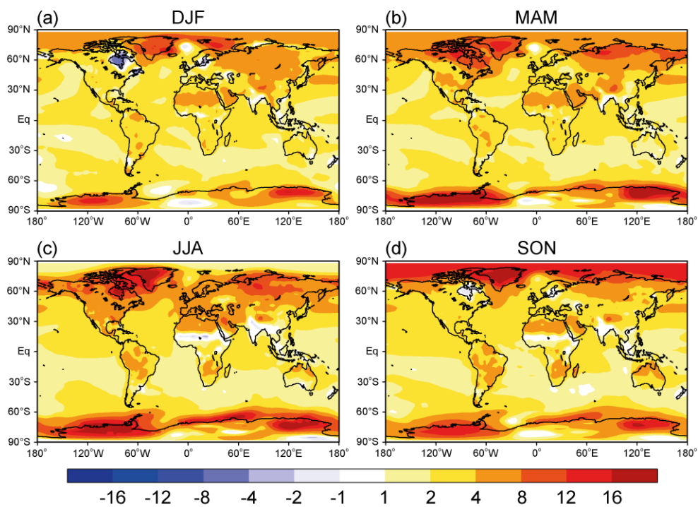
Figure 5: Seasonal surface air temperature anomaly between E_{oi}^{400} and E^{280} for December-February (DJF), March-May (MAM), June-August (JJA) and September-November (SON).
