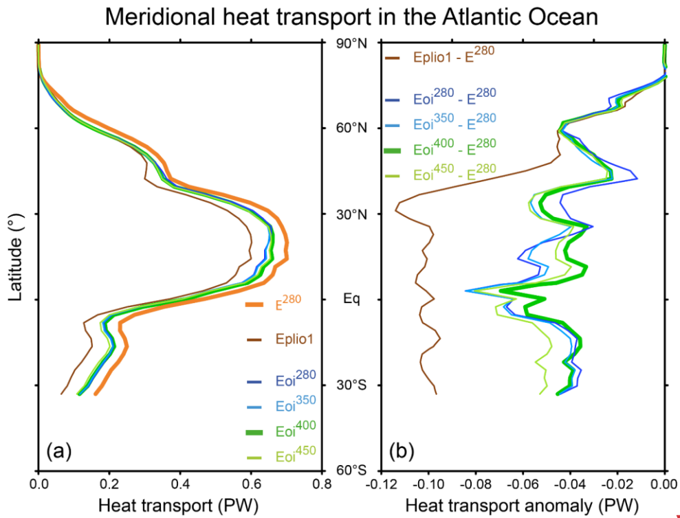
815 Figure 12: (a) The Atlantic Ocean meridional heat transport in the Pliocene experiments and in E 280 and (b) the anomaly between the Pliocene experiments and E 280 . The core experiment, Eoi 400 , is shown in bold green.
