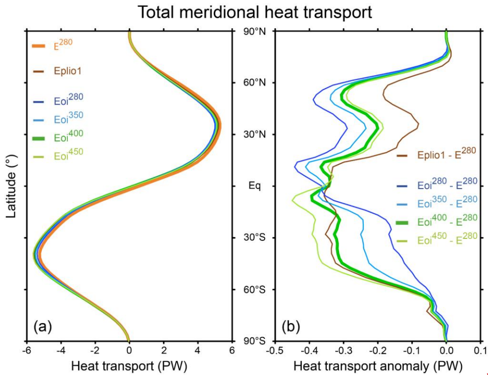
Figure 13: (a) The total meridional heat transport in the Pliocene experiments and in E^{280} , as calculated from the top-of-atmosphere radiative transport, and (b) the anomaly between the Pliocene experiments and E^{280} . The core experiment, Eoi^{400} , is shown in bold green.
