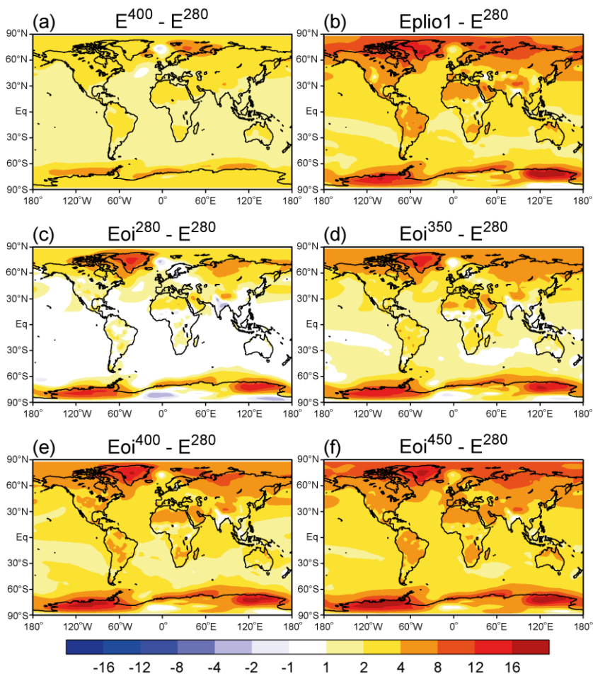
Figure 3: Annual mean surface air temperature anomaly between six experiments and E 280 , the Pre-Industrial. For a comparison of PlioMIP1 and PlioMIP2, see (b) and (e). For the individual effects of CO 2 and Pliocene boundary conditions, see (a) and (c), respectively.
