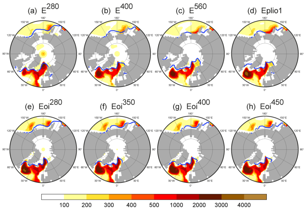
Figure 9: Oceanic mixed layer depth in the northern hemisphere during March. The blue lines indicate the extent of 15% sea ice concentration. For a comparison of PlioMIP1 and PlioMIP2, see (d) and (g). For the individual effects of CO 2 and Pliocene boundary conditions, see (b) and (e), respectively.
