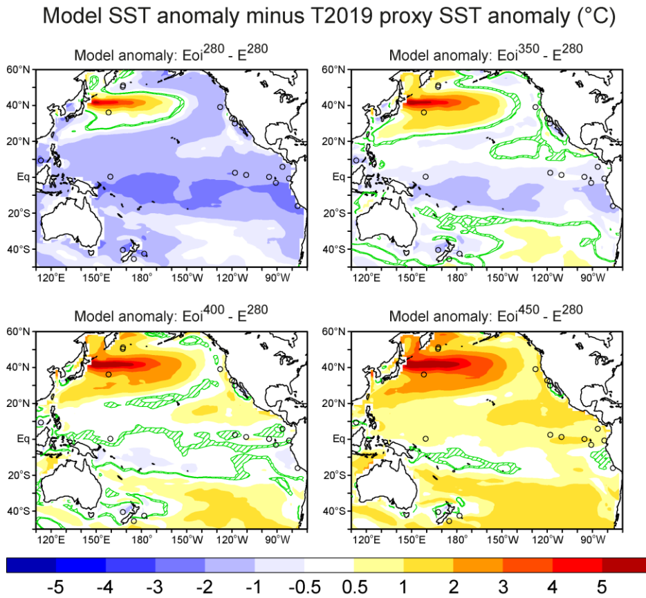
Figure 18: Comparison of annual mean model SST anomalies and T2019 (Tierney et al, 2019) proxy data SST anomalies. Model anomalies refer to the Pliocene experiments, a) Eoi280, b) Eoi350, c) Eoi400 and d) Eoi450. For reference, the location of T2019 core sites are shown as black circles. 95% confidence levels are shown by the green striped area.
