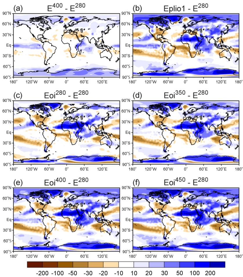
Figure 7: Annual mean precipitation anomaly between six experiments and E^{280} , the Pre-Industrial, as a percentage of E^{280} , eg. 100 \times (E_{oi}^{400} - E^{280}) / E^{280} . For a comparison of PlioMIP1 and PlioMIP2, see (b) and (e). For the individual effects of CO 2 and Pliocene boundary conditions, see (a) and (c), respectively.
