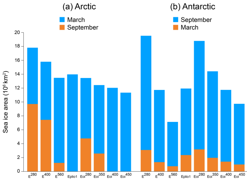
800 Figure 8: Total surface area of sea ice in each polar region during March and September.
