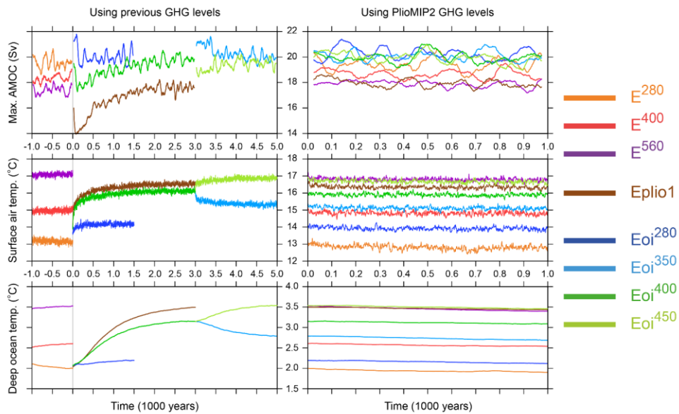
Figure 2: Time series of the AMOC index (top), globally averaged surface air temperature (middle) and global ocean temperature below depths of 1900m (bottom). A 51-year moving average has been applied to the AMOC index time series. The subfigures on the left depict the initial stages of the experiments during which greenhouse gas levels are set to previous, PlioMIP1 values, while the subfigures on the right depict the final 1000 years of the integration during which greenhouse gas levels are consistent with those specified in PlioMIP2.
