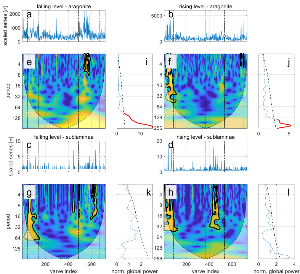
465 Figure 8 – Wavelet and global-wavelet spectrogram of aragonite thickness and flood frequency during falling (left) and rising (right) episodes. Patches with significance level above 0.95 ( \alpha=0.05 ) detected using the cumulative area-wise significance test are depicted by a bold black line (Schulte et al., 2018; Schulte, 2016). Each triplot section shows the normalized data (a-d), the wavelet spectra (e-h) and the global wavelet spectra (blue) compared against the significance test of the global wavelet power spectra (dashed black, i-l). Significant peaks of arcs are marked in red (Schulte, 2019). Dashed vertical lines in (e-h) depict clusters identified as episodes of increased flood frequency. Note that the short-term cyclical component in the global wavelet spectra, which fail the significance test using the original series, are found to be significant in the analysis of the detrended series (Fig. S14).
