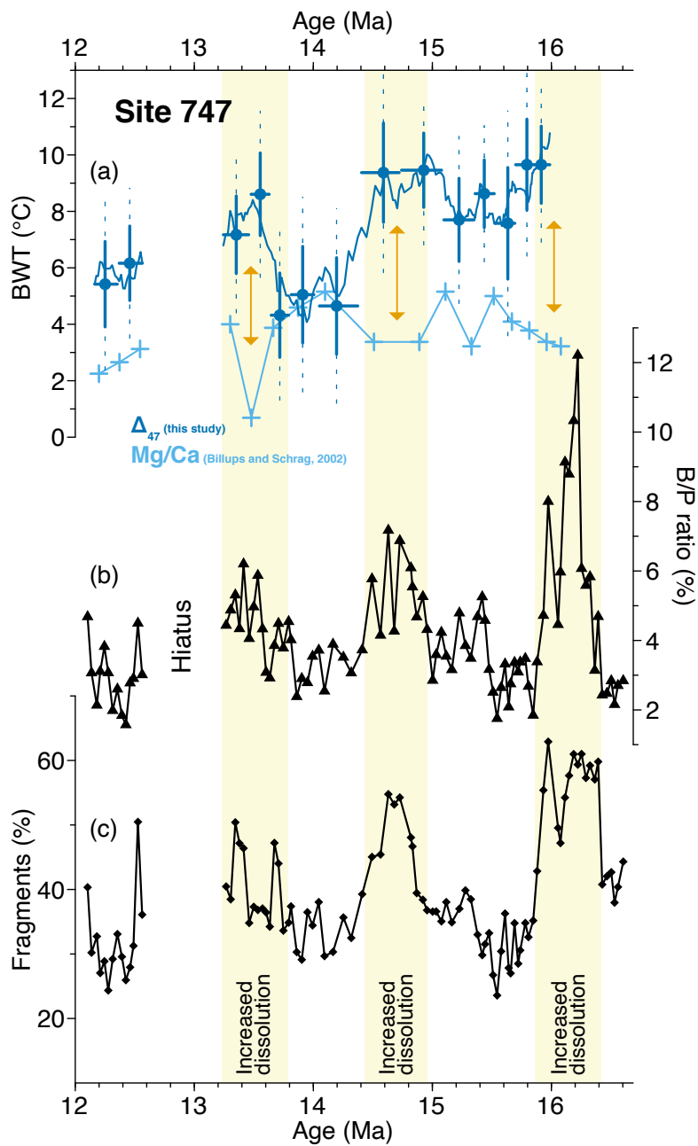
320 Fig. 4: Bottom water temperature (BWT) and dissolution at Site 747. (a) \Delta_{47} - and Mg/Ca-based BWT estimates (this study; Billups and Schrag, 2002) are shown versus (b) percent benthic to planktic (B/P) foraminiferal test ratios (Diester-Haass et al., 2013) and (c) percent fragments in a sample (Diester-Haass et al., 2013). Percent fragments and B/P foraminiferal test ratios have been previously used to monitor dissolution at Site 747 (Diester-Haass et al., 2013). Intervals interpreted as affected by increased dissolution of planktic
