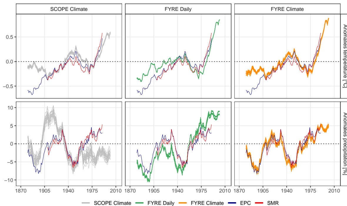
Figure 8. Anomalies of annual temperature (top panels) and precipitation (bottom panels) averaged over France, and smoothed with a 20-year rolling mean. See text for details.
