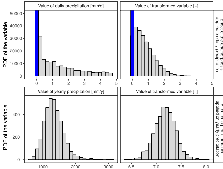
Figure 3. Schematic view of the transformations applied to SCOPE Climate daily (upper panels) and yearly (lower panels) precipitation for the case study cell during the 1958–2008 period. The blue line represents zero values. For daily precipitation the x-axis of left panels is truncated at 5 mm/d for readability.
