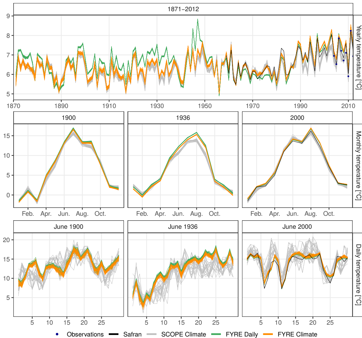
Figure 9. Temperature time series of SCOPE Climate, FYRE Climate, FYRE Daily and Safran over the case study cell for different periods and different time steps.
