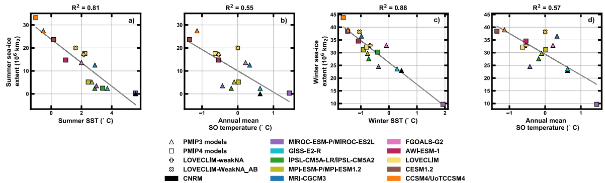
Figure 5. Scatter plot showing the relationship between sea ice, SO SST (averaged over 50-75°S) and SO temperature (averaged over 50-75°S and 0-5500m depth) in all experiments. Panels a, b show the relationship for austral summer and panels c, d show the relationship for austral winter.
