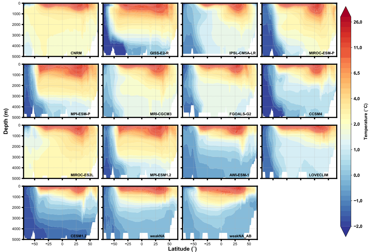
Figure 6. Zonally averaged oceanic potential temperatures ( ^{\circ}\text{C} ) in the Atlantic basin for PMIP3, PMIP4 and LOVECLIM simulations.
