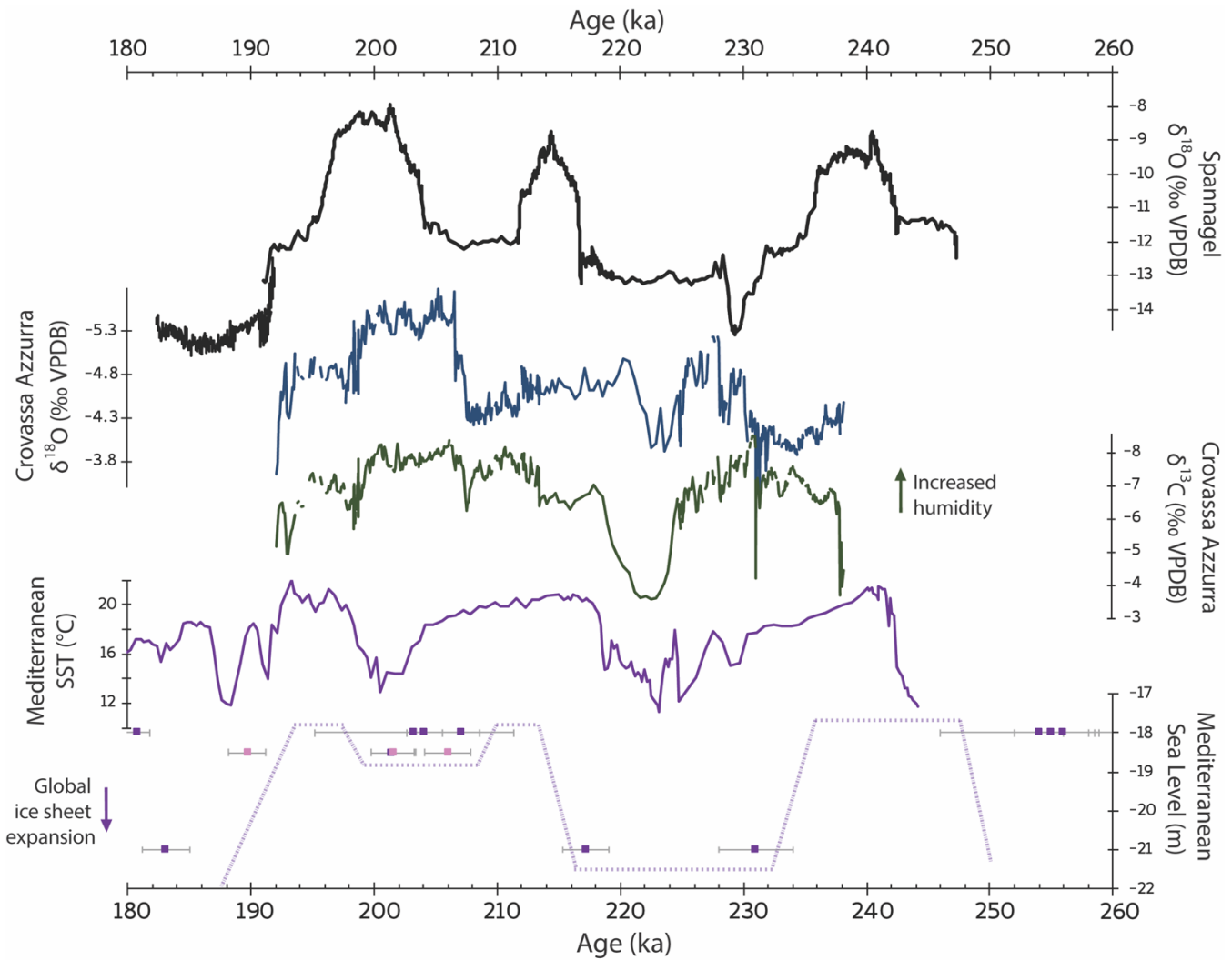
615 Figure 5: MIS 7 records from the circum-Mediterranean region. Spannagel Cave \delta^{18}\text{O} (black; this study), Crovassa Azzurra (Sardinia, Italy) \delta^{18}\text{O} (blue) and \delta^{13}\text{C} (green) (Columbu et al., 2019), Western Mediterranean SST (Martrat et al., 2004), and Mediterranean sea-level reconstructions (purple; Dutton et al., 2009) and (pink; Bard et al., 2002). Purple dashed lines are for visual aid only; absolute sea levels are unknown. Spannagel \delta^{18}\text{O} events that are decoupled from Mediterranean temperatures and humidity records represent evidence for temperature-driven \delta^{18}\text{O} excursions in the Austrian Alps, as opposed to changes in the proportion of Mediterranean-sourced moisture arriving at our study site.
