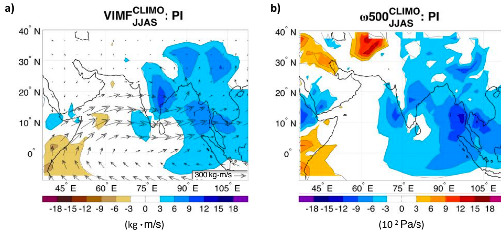
Figure A10. Climatological summer (JJAS, June to September) (a) vertical integrated horizontal moisture flux (VIMF, \text{kg} \cdot \text{m/s} ) with the arrows representing the zonal and meridional component of the moisture flux; (b) vertical pressure velocity at 500 hPa ( \omega_{500} , 10^{-2} \text{ Pa/s} ), in the pre-industrial (PI) simulation.
