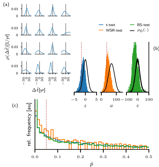
Figure 6. Exemplary application of the analysis to the proxy pair ( \text{Ca}^{2+}, \text{Na}^+ ) from the NGRIP ice core. Panel (a) shows 16 uncertain time lags \Delta\hat{T}_i derived from the proxy data around DO events. The continuous densities have been obtained via a Gaussian kernel density estimate from the corresponding MCMC samples (see Sec. 3.1). In panel (b) the uncertain test statistics induced by the uncertain sample are shown for the t -test (blue), the WSR-test (orange) and a bootstrap test (green). The values that comprise the histograms are immediately derived from the MCMC samples. Panel (c) shows the empirical uncertainty distribution for the p -values of the three tests, following from the uncertain test statistics in panel (b). Dotted red lines separate rejection from acceptance regions in panels (b) and (c). In case of the bootstrap test, the rejection regions cannot be defined consistently on the level of the test statistic, since each possible value \Delta\hat{t} for the uncertain \Delta\hat{T} induces its individual null distribution. The null distribution shown here is in fact the pooled distribution of resampled \tilde{v}_j obtained from all MCMC-sampled values for \Delta\hat{T} . For the other proxy pairs investigated in this study, corresponding plots would appear structurally similar.
