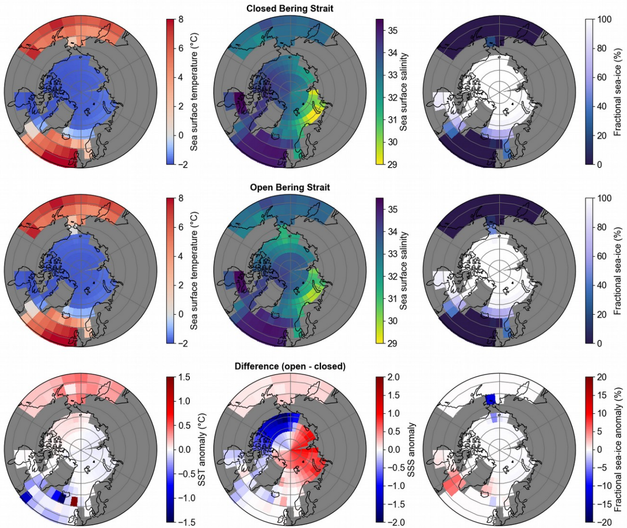
Figure B7. Annual mean sea surface temperature (SST), sea surface salinity (SSS), and fractional sea-ice north of 50° N under LGM boundary conditions. (top) Closed Bering Strait (simulation LGM_BS+wind+tidal), (middle) new steady-state after transiently opening the Bering Strait but all other boundary conditions as in top panel, and (bottom) difference between open and closed Bering Strait.
