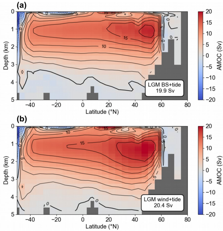
Figure B6. Atlantic stream functions for LGM boundary conditions with (a) closed Bering Strait and consideration of increased tidal dissipation after Wilmes et al. (2019) and (b) added LGM wind stress anomalies from PMIP3 models (Muglia and Schmittner, 2015) and increased tidal dissipation.
