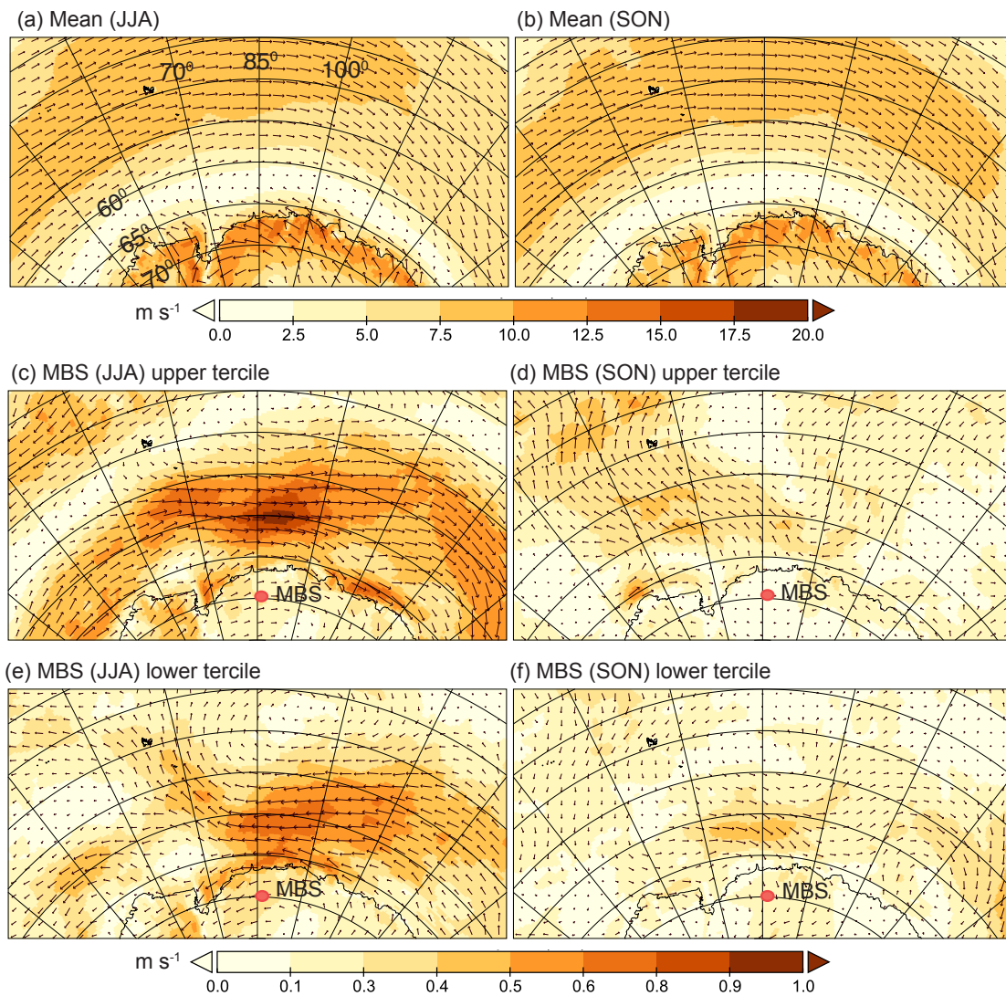
65 Figure 9. Near-surface (10 m) wind vector composite maps of the mean state during austral winter (a, June-August) and spring (b, September-November), and anomaly composite maps during upper (c) and lower (e) tercile in June-August of the detrended, log-transformed annual sea salt concentrations from the Mount Brown South (MBS) site average, over the period 1979-2016. (d, f) same as (c, e) except in September-November. The red dot indicates the MBS site location. Latitudinal lines are in increments of 5^\circ and longitudinal lines are in increments of 15^\circ .
