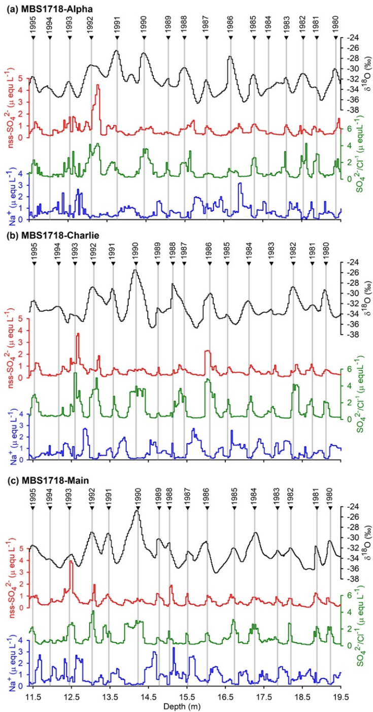
95 Figure 2. An 8 m long section from the Mount Brown South (MBS1718-Alpha (a), MBS1718-Charlie (b) and MBS1718- Main (c)) ice cores. These sections cover the period 1980-1995 (which contains some ambiguous annual horizons, see section 3.1), with annual layers (year boundaries) shown as triangles with vertical grey lines. Annual horizons are identified from summer-peaking glaciochemical species (i.e., oxygen isotopes ( \delta^{18}\text{O} ), non-sea salt sulphate ( \text{nssSO}_4^{2-} ) and the ratio between sulphate and chloride ( \text{SO}_4^{2-}/\text{Cl}^- )). Winter-peaking sea salts ( \text{Na}^+ ) are used as a confirmatory 00 species. Panels (a) and (b) are on the same depth scale as shown in (c).
