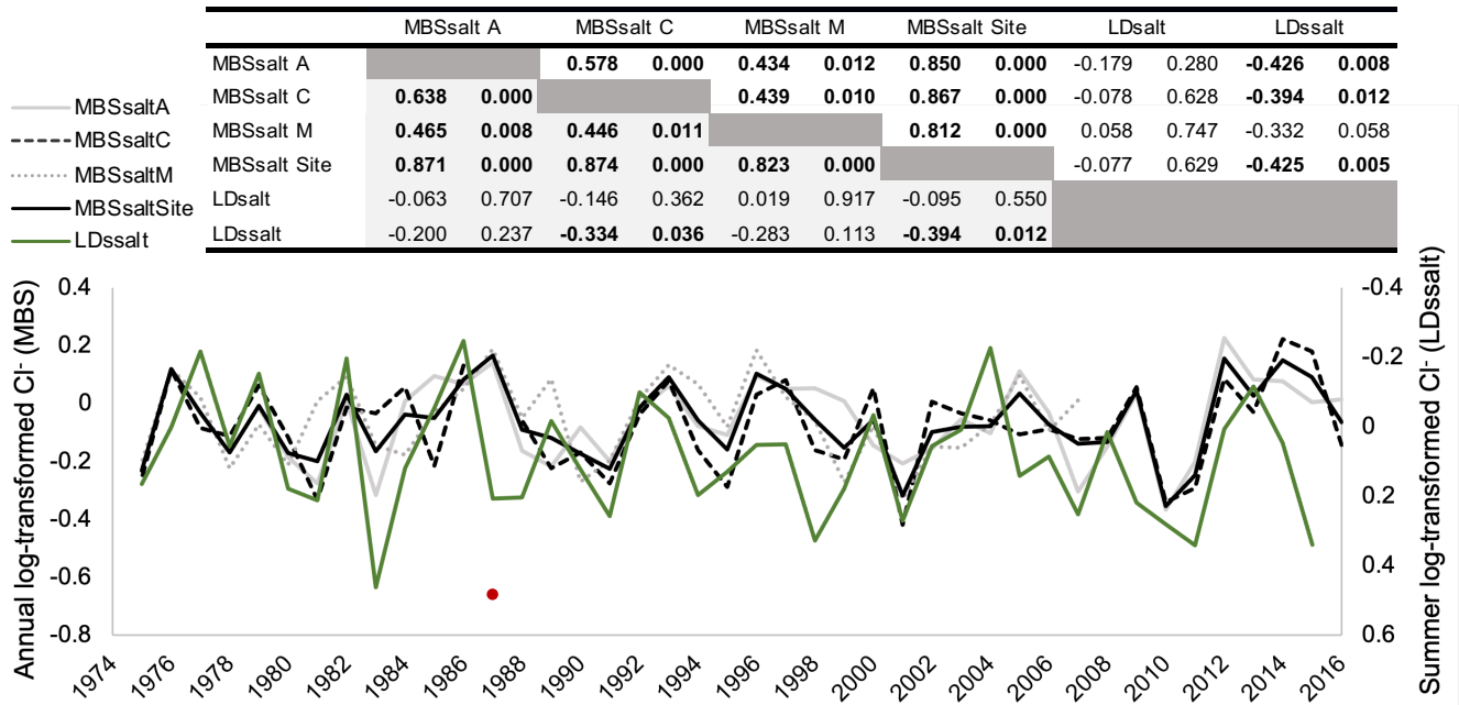
25 Figure 5. Timeseries of log-transformed annual sea salt concentrations for the Mount Brown South site average (MBSsalt Site), the Alpha (MBSsaltA), Charlie (MBSsaltC) and Main (MBSsaltM) ice cores, including the Charlie 1987 (red dot) outlier, and the log-transformed summer sea salt concentrations for the Law Dome (Dome Summit South site; LDssalt) record (on inverted secondary axis). Embedded table shows Pearson's correlation coefficient ( r -left column, p -right column) for the log-transformed sea salt concentrations for MBSsaltSite, MBSsaltA, MBSsaltC, MBSsaltM, LDssalt, and the log-transformed annual sea salt concentrations for the Law Dome (LDsalt) record. Correlations for normalised Gaussian smoothed (kernel = 3 yearly points, sigma = 0.6) sea salt concentrations are shaded and presented in the lower-left of the table. Correlations significant at 95% are bold, and the dates range between 1975-2016. 30
