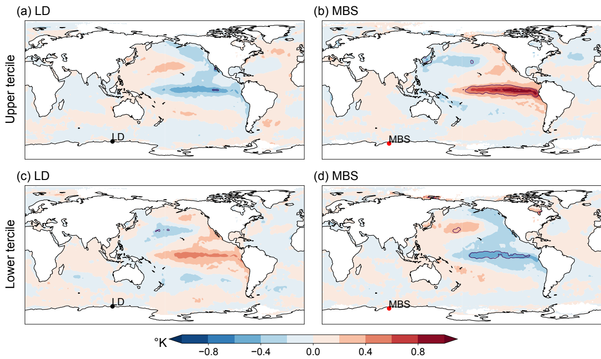
50 Figure 7. SST anomalies composite maps during upper (a) and lower (c) tercile (November-February) of the detrended, log-transformed summer sea salt concentrations from the Law Dome (LD, Dome Summit South site) record over 1975-2015, and upper (b) and (d) lower tercile (June-November) detrended, log-transformed sea salt concentrations from the annual Mount Brown South (MBS) site average over 1975-2016. The red dot indicates MBS and the black dot indicates LD. Significant anomalies are within the upper and lower purple contour lines, where p < 0.1 .
