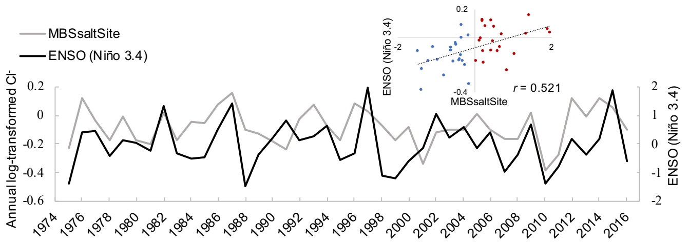
640 Figure 6. Timeseries of the annual detrended, log-transformed sea salt concentrations for the Mount Brown South site average (MBSsaltSite) and the detrended (June-November) El Niño Southern Oscillation region SST anomalies (ENSO (Niño 3.4 Index)). Embedded scatterplot shows the relationship between the two time series differentiated by positive (red dots) and negative (blue dots) Niño 3.4 region SST anomalies based on the period 1975-2016.
