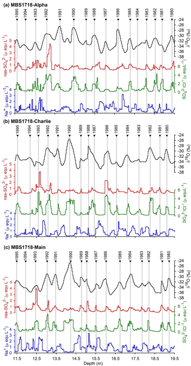
Figure 2. An 8 m long section from the Mount Brown South (MBS1718-Alpha (a), MBS1718-Charlie (b) and MBS1718-Main (c)) ice cores. These sections cover the period 1980-1995 (which contains some ambiguous annual horizons, see section 3.1), with annual layers (year boundaries) shown as triangles with vertical grey lines. Annual horizons are identified from summer-peaking glaciochemical species (i.e., oxygen isotopes ( \delta^{18}\text{O} ), non-sea salt sulphate ( \text{nssSO}_4^{2-} ) and the ratio between sulphate and chloride ( \text{SO}_4^{2-}/\text{Cl}^- )). Winter-peaking sea salts ( \text{Na}^+ ) are used as a confirmatory species. Panels (a) and (b) are on the same depth scale as shown in (c).
