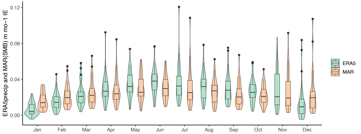
Figure 4. Climatology of surface mass balance and precipitation estimates at Mount Brown South from the Model Atmospherique Regional (MAR(SMB)) and ERA5 (ERA5precip), respectively, over the period 1975-2016.
