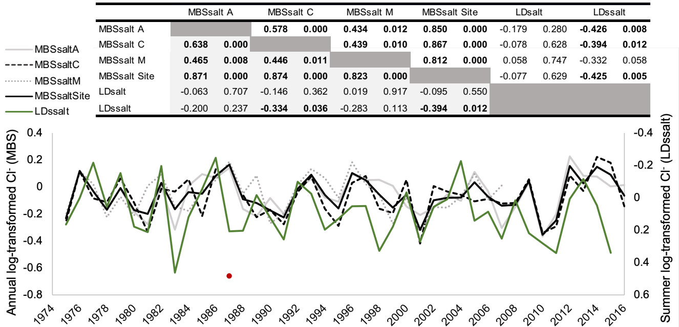
620 Figure 5. Timeseries of log-transformed annual sea salt concentrations for the Mount Brown South site average (MBSsalt Site), the Alpha (MBSsaltA), Charlie (MBSsaltC) and Main (MBSsaltM) ice cores, including the Charlie 1987 (red dot) outlier, and the log-transformed summer sea salt concentrations for the Law Dome (Dome Summit South site; LDssalt) record (on inverted secondary axis). Embedded table shows Pearson’s correlation coefficient ( r -left column, p -right column) for the log-transformed sea salt concentrations for MBSsaltSite, MBSsaltA, MBSsaltC, MBSsaltM, LDssalt, and the log-transformed annual sea salt concentrations for the Law Dome (LDsalt) record. Correlations for normalised Gaussian smoothed (kernel = 3 yearly points, sigma = 0.6) sea salt concentrations are shaded and presented in the lower-left of the table. Correlations significant at 95% are bold, and the dates range between 1975-2016. 625
