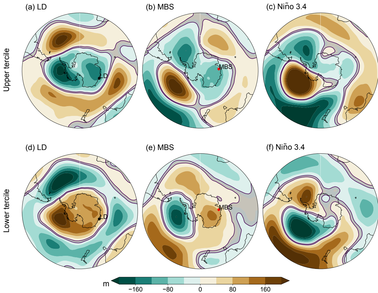
655 Figure 8. Geopotential height composite anomaly maps (m at Z500) during upper (a) and lower (d) tercile (November-February) of the detrended, log-transformed summer sea salt concentrations from the Law Dome (LD, Dome Summit South site) record over 1979-2015. (b, e) same as (a, d) except using the detrended, log-transformed annual sea salt concentrations from the Mount Brown South (MBS) site average (June-November) over the period 1979-2016. (c, f) same as (b, e) except using the detrended Niño 3.4 index (June-November). The red dot indicates MBS and the black dot indicates LD. Significant anomalies are within the upper and lower purple contour lines, where p < 0.1 .
