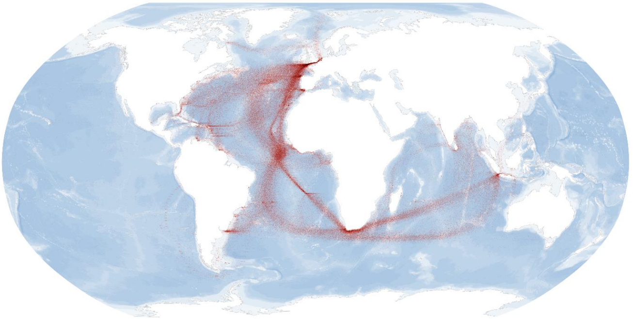
Figure 10: Plot of the position of all ships' logbook entries in the CLIWOC database (Degroot and Ottens, 2020). The map is derived from the open source variant of the CLIWOC database (García-Herrera et al., 2005b) held at https://www.historicalclimatology.com .
