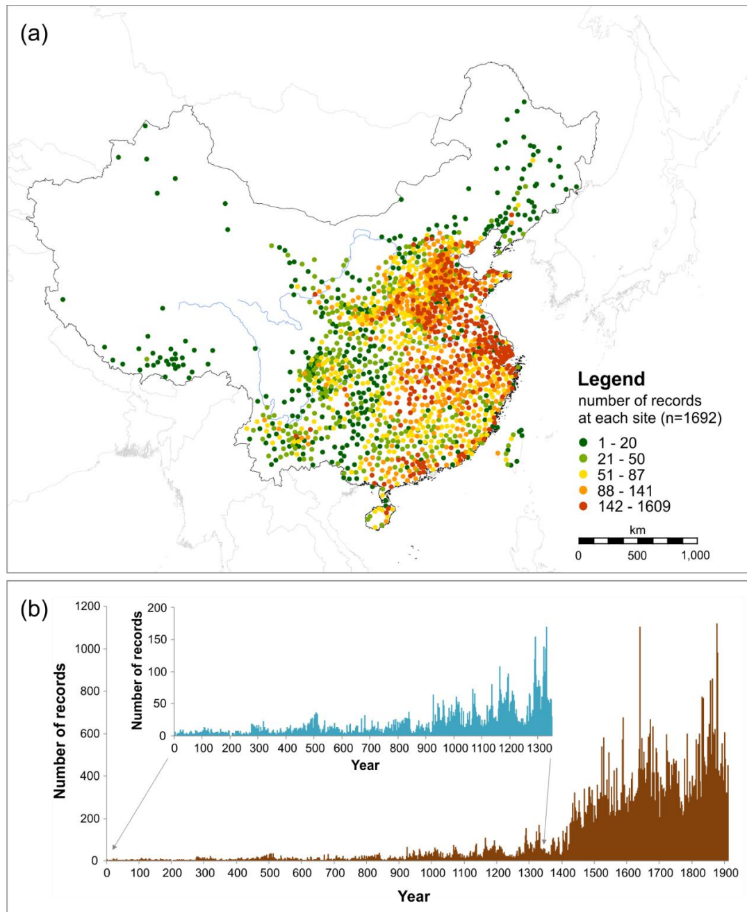
369 Figure 3: Numbers of historical documentary records in the REACHES database for China. (a) Spatial distribution of 370 records at 1,692 geographical sites across China. (b) Temporal evolution of the records in the database from 1 to 1911 CE 371 (brown series); inset (blue series) shows the same data for 1 to 1350 CE but with an expanded vertical axis.
