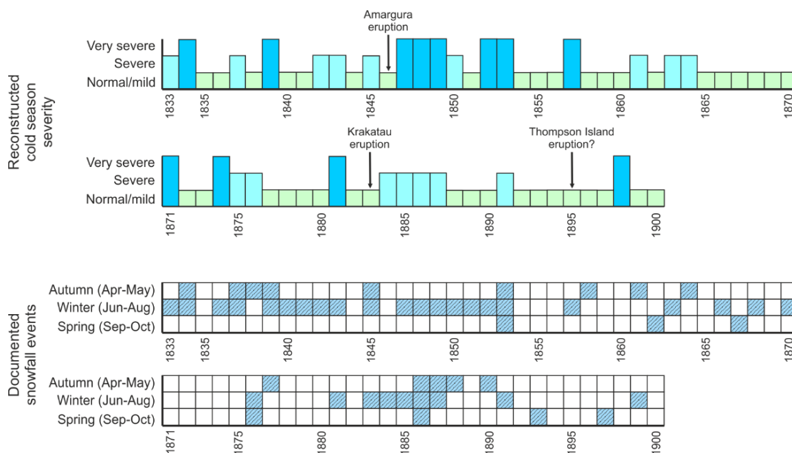
499 500 Figure 7: Three-point “cold season severity” index for Lesotho and surrounding areas during the 19th century (top), with 501 major volcanic eruptions indicated. The occurrence of snowfall events (bottom) during the same period is also shown 502 (modified after Grab and Nash, 2010).
