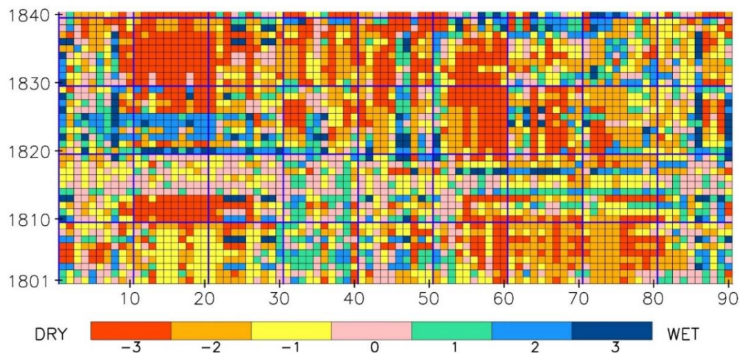
482 483 Figure 5: Seven-point "wetness" index series for 1801 to 1840 for the 90 homogenous rainfall regions of Africa indicated 484 across the x-axis. This series is reconstructed using documentary and instrumental data, with data gaps infilled using 485 substitution and statistical inference (see section 8.3 and Nicholson et al., 2012a). From left to right, the regions 486 approximately extend by latitude from the northern (region 1 – Northern Algeria/Tunisia) to southern (region 84 – western 487 Cape, South Africa) extremes of the continent. Anomalies in the numbering sequence are regions 85, 86, 90 (all equatorial 488 Africa), 87 (eastern Africa) and 88, 89 (Horn of Africa).
