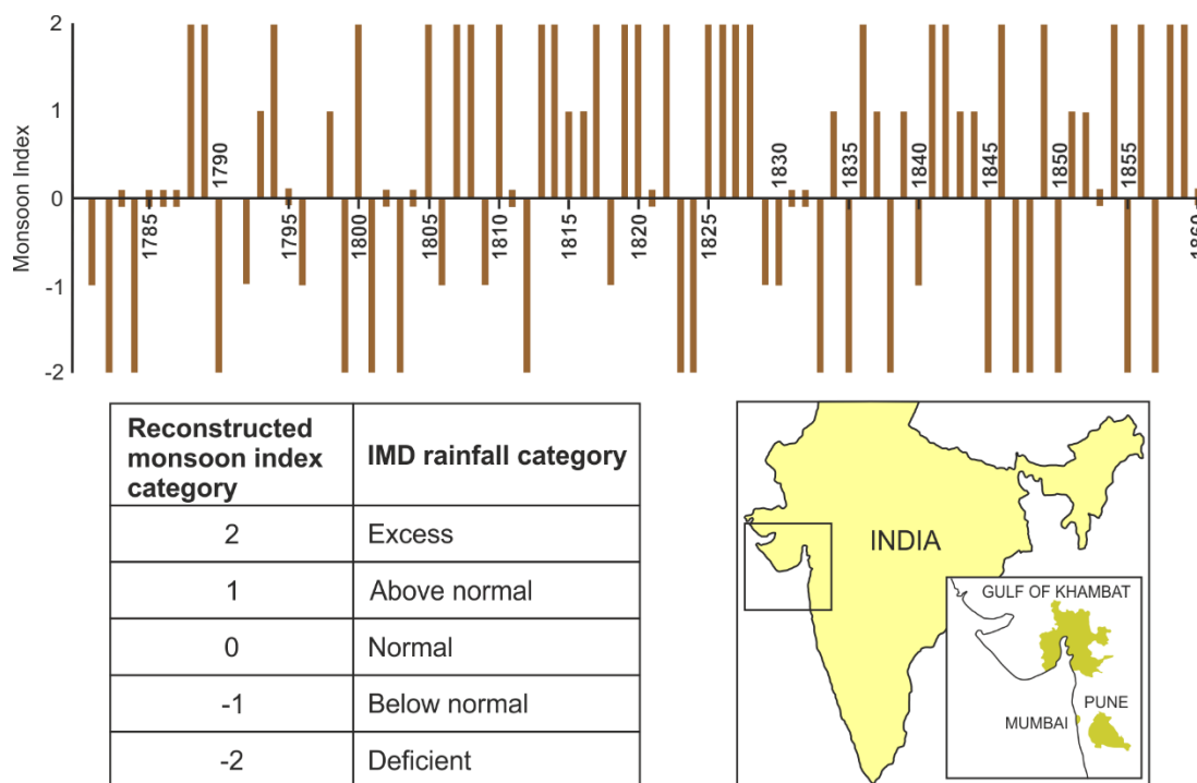
415 Figure 4: Five-point Western India Monsoon Rainfall reconstruction for 1780-1860. The reconstruction is a combination of 416 separate series for Mumbai, Pune and the Gulf of Khambhat (see inset). Monsoon index categories map broadly onto Indian 417 Meteorological Department (IMD) descriptors of seasonal monsoon rainfall (data for reconstruction from Adamson and 418 Nash, 2014). Zero values are shown as small bars; years with insufficient data to generate an index value are left blank.
