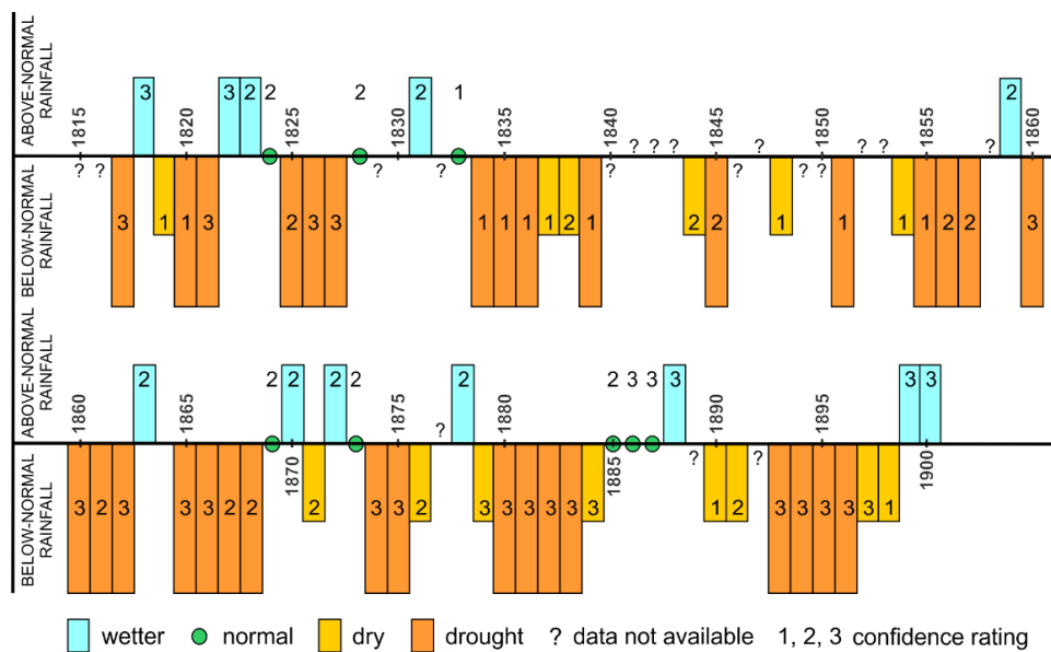
1043 Figure 13: Five-point index of rainfall variability in Namaqualand (South Africa) during the 1800s, including the first use of 1044 confidence ratings in relation to annual classifications in a documentary-derived index series (1 = low confidence, 3 = high 1045 confidence). Data from Kelso and Vogel (2007).
