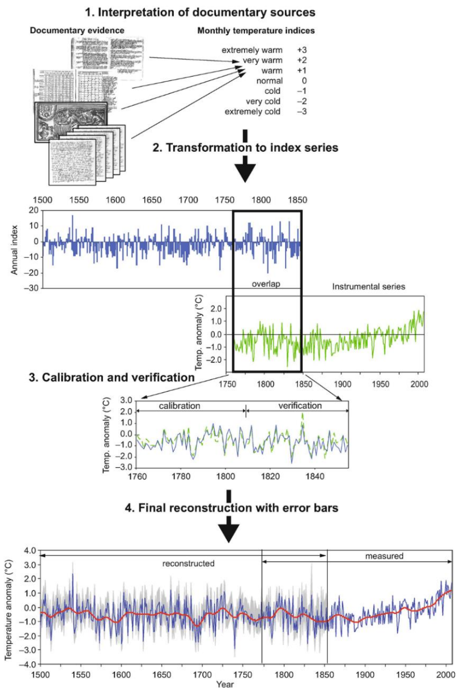
941 Figure 11: The main steps in quantitative climate reconstruction based on temperature or precipitation indices derived from 942 documentary evidence. Historical documentary sources are analysed to generate seven-point monthly indices (step 1), which 943 are then summed to produce annual index series (step 2). Calibration and verification are carried out on periods of 944 overlapping instrumental data (step 3), with statistical results from verification used to define error bars for the final
