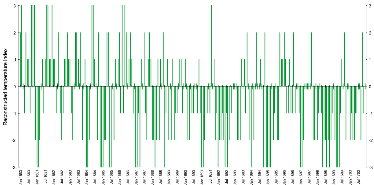
124 Figure 1: Monthly seven-point temperature indices for the Swiss Plateau (1680-1700), reconstructed using the Pfister index 125 approach (data from Pfister, 1998). Zero values for specific months are indicated by a small green bar.
