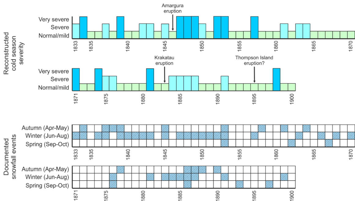
489 Figure 7: Three-point “cold season severity” index for Lesotho and surrounding areas during the 19th century (top), with 490 major volcanic eruptions indicated. The occurrence of snowfall events (bottom) during the same period is also shown 491 (modified after Grab and Nash, 2010).
