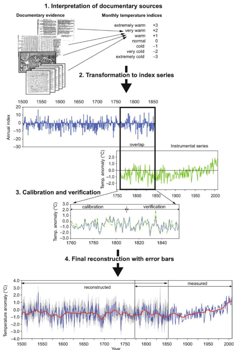
942 Figure 11: The main steps in quantitative climate reconstruction based on temperature or precipitation indices derived from 943 documentary evidence. Historical documentary sources are analysed to generate seven-point monthly indices (step 1), which 944 are then summed to produce annual index series (step 2). Calibration and verification are carried out on periods of
