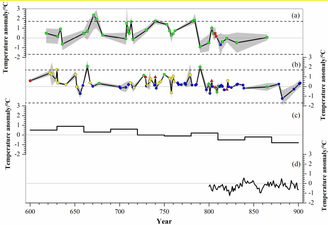
Figure 3 Comparison of reconstructed temperature anomalies for 600-900 AD (with respect to the mean climatology between 1961 and 1990). (a): The annual mean temperature anomalies
