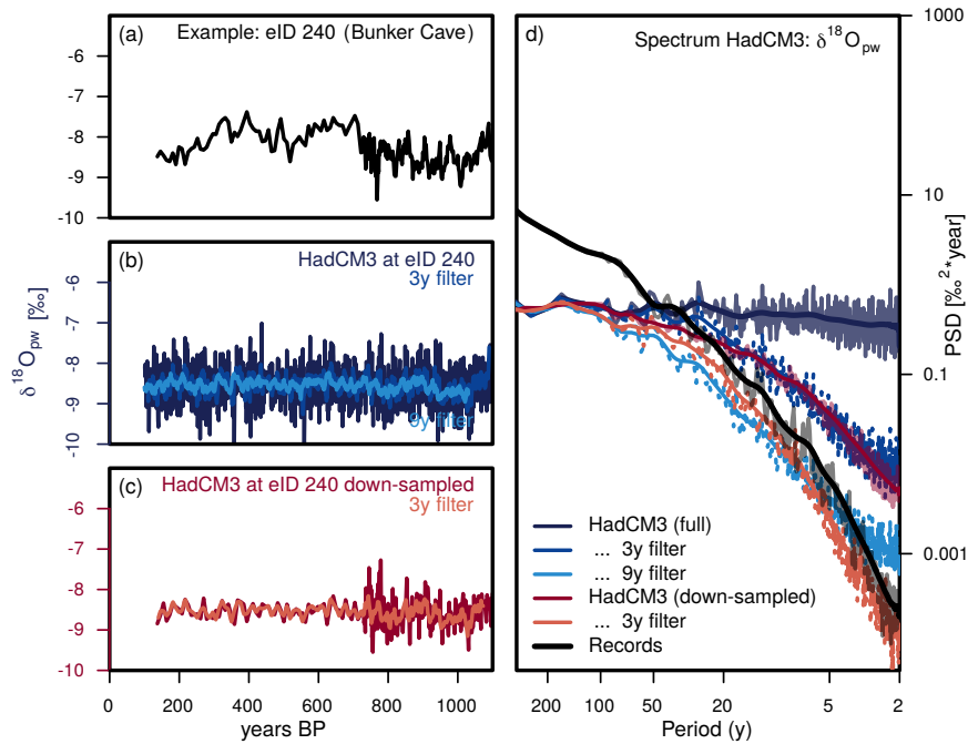
Figure 6. Variability on different time scales through comparison of measured \delta^{18}\text{O}_{dw.eq} and simulated \delta^{18}\text{O}_{pw} time series as well as of their spectra. (a-c) Example time series of eID 240 in Bunker cave (Germany) (Fohlmeister et al., 2012). (a) The measured \delta^{18}\text{O}_{dw.eq} in the speleothem, (b) the iHadCM3 simulated \delta^{18}\text{O}_{pw} at the cave location with two filters (3 and 9 years) and (c) the simulated \delta^{18}\text{O}_{pw} but down-sampled to the same temporal resolution as in (a) with 3 year filter. (d) Power spectral density (PSD) of mean spectra of simulated \delta^{18}\text{O}_{pw} at the cave site in yearly resolution (blue), down-sampled to the caves resolution (red) and mean spectrum of the \delta^{18}\text{O}_{dw.eq} of the records (black), including the karst-filters as shown in (a-c). The spectra are area-weighted and averaged over the three simulations (LM1, LM2 and LM3). The colors for the example eID in (a-c) correspond to the colors of the mean spectra over all entities in (d).
