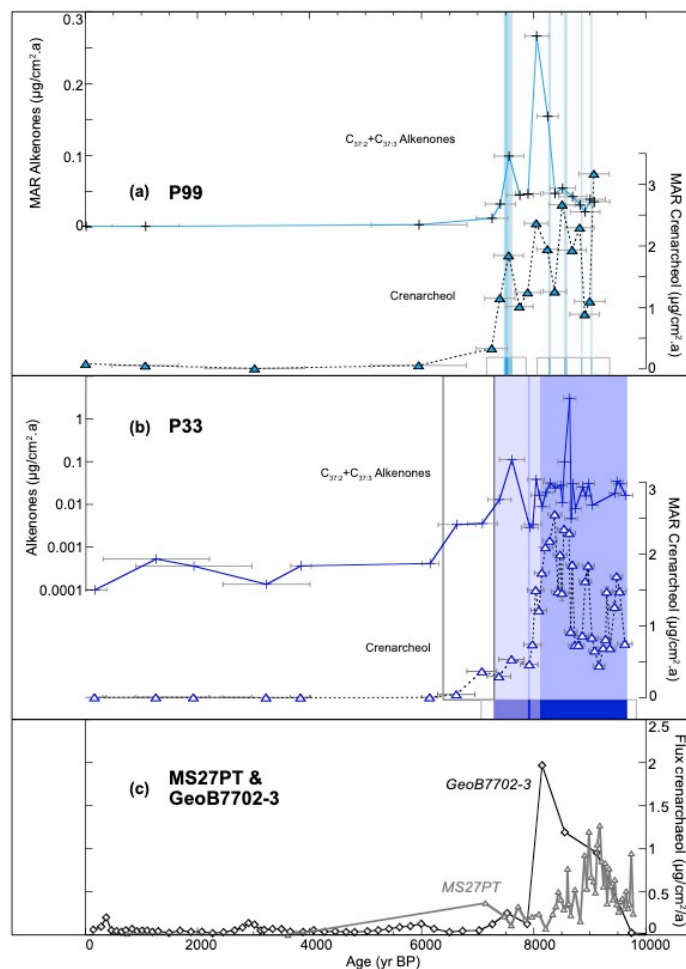
349 350 Figure 7. Proxies of primary productivity in cores (a) P99 (turquoise), (b) P33 (blue), (c) GeoB7702-3 (black) and MS27PT (grey) on 351 age scale (0-10 ka BP). MAR of alkenones (crosses and continuous lines) and MAR of crenarchaeol for cores P33 and P99 (triangles 352 and dashed lines), as well as for cores GeoB7702-3 (black diamonds) (Castañeda et al., 2010) and MS27PT (grey triangles) (Ménot 353 et al., 2020). Lamination pattern (similar colour coding as in Fig. 6). Grey bars show the age uncertainty.
