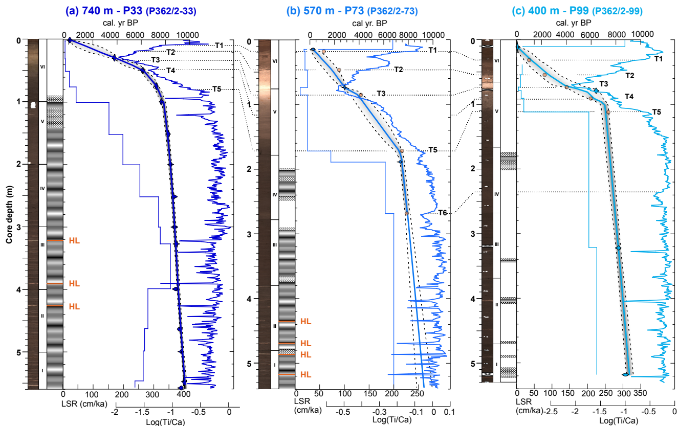
180 Figure 2. Age models. (a) core P33, (b) core P73 and (c) core P99. For all cores, from left to right: core depth (m), half-core surface 181 images (for core P99, realised after sampling with empty sections shown as crosses), section number (roman numbers), schematic 182 lithological log (white: bioturbated, dashed: faint laminations, hatched: laminations, orange: hard layers labelled HL), linear 183 sedimentation rates (cm/ka, step curves), age-depth relationships as computed by Bacon V2.3 (Blauw and Christen, 2011) with 184 radiocarbon ages (blue violin distributions) and tie points (orange dots), Log(Ti/Ca) records with tie-points T1-T6 (dashed lines) 185 (Tab. 2).
