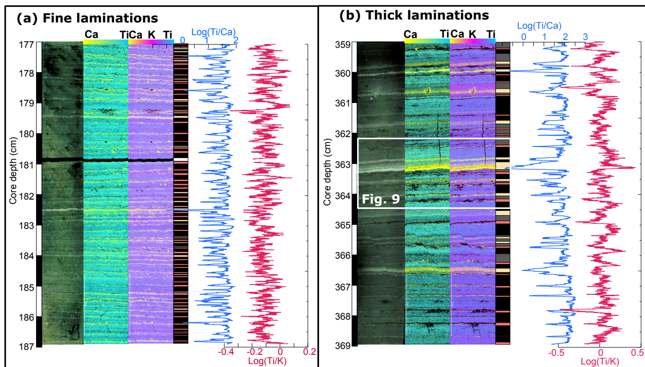
272 273 Figure 4. Laminations in core P33. (a) Fine laminations and (b) thick laminations from sections located at ca. 180 and 360 cm core 274 depth, respectively. From left to right: core depth (cm), cross-polarized scan of the thin section, elemental mapping showing relative 275 amounts of calcium (Ca, yellow) versus titanium (Ti, turquoise), elemental mapping showing relative amounts of calcium (Ca, 276 yellow), potassium (K, pink) and titanium (Ti, blue), schematic lithological log with color-coded sublayer type following Fig. 3a (LL1: 277 pink, DL1, grey, LL2: yellow and DL2: black), down-section profile of \log(\text{Ti}/\text{Ca}) (blue) and \log(\text{Ti}/\text{K}) (red).
