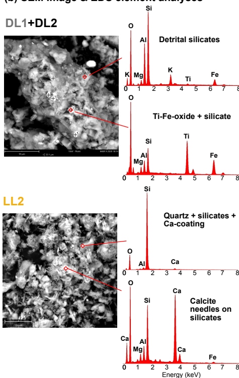
(b) SEM image &amp; EDS element analyses
