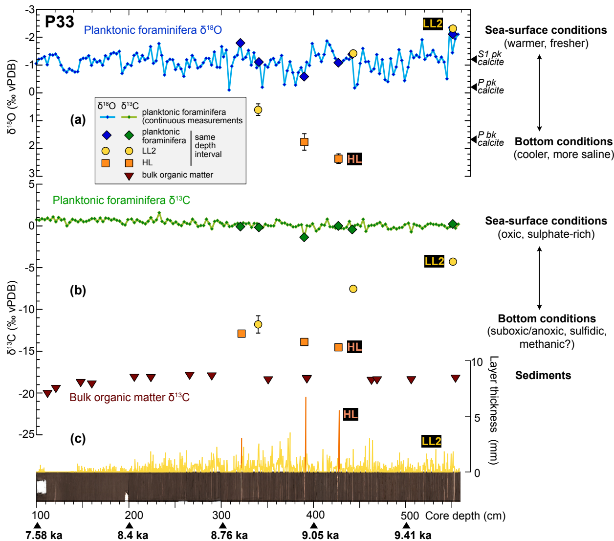
495 496 Figure 10. Changes in water-column stratification and chemistry as provided by isotopic composition of authigenic calcite in 497 individual LL2 and HL of core P33. (a) \delta^{18}\text{O} of planktonic foraminifera (blue curve and diamonds), LL2 (yellow dots) and HL 498 (orange squares), as compared to biogenic and inorganic calcite formed in equilibrium with seawater providing information on the 499 water-column stratification as indicated on the right-hand side. (b) \delta^{13}\text{C} of planktonic foraminifera (green curve and diamonds), 500 LL2 (yellow dots) and HL (orange squares) and bulk organic matter (brown triangles) showing the changes in water-mass 501 oxygenation state. (c) Thickness of LL2 and HL, picture of the core surface, depth scale and indications of age.
