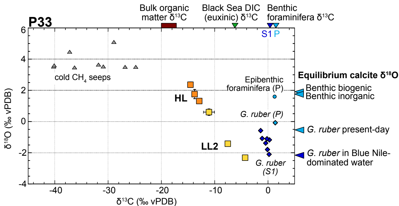
290 291 Figure 5. Isotopic signature of LL2 and HL from core P33. Scatter plot of \delta^{18}\text{O} vs \delta^{13}\text{C} values of three LL2 (yellow) and three 292 cemented HL (orange), as compared to isotopic signatures of methane-derived carbonates from the Nile DSF (grey triangles) (Aloisi 293 et al., 2000; Bayon et al., 2013); P33 top-core and S1 planktonic foraminifera (light and dark blue diamonds, resp.); present and S1 294 epibenthic foraminifera (light blue circle and blue triangles; Grimm et al., 2015); P33 bulk organic matter \delta^{13}\text{C} (brown rectangle); 295 Black Sea \delta^{13}\text{C} of dissolved inorganic carbon (DIC) (green triangle) (Fry et al., 1991); \delta^{18}\text{O} value of biogenic and inorganic benthic 296 and planktonic calcite formed in equilibrium with seawater (blue triangles) (Table S4, see calculation details in Supplementary 297 Information).
