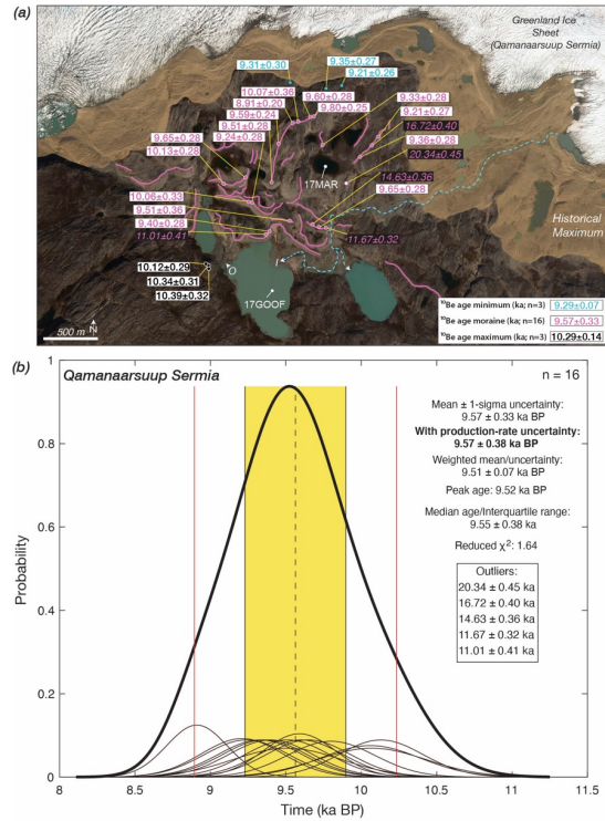
290 Figure 3: (a) Qamanaarsuup Sermia region depicting the Kapisigdlit stage moraines (pink) and retreat since from the historical maximum extent (brown shading); moraines were mapped in the field. 10 Be ages (ka BP ± 1 S.D.) are from three morphostratigraphic groups: 1) erratic boulders perched on bedrock outboard the Kapisigdlit stage moraines (black symbols and text), 2) Kapisigdlit stage moraine boulders (pink symbols and text), and 3) erratic boulders perched on bedrock inside the Kapisigdlit stage moraines (blue symbols and text). 10 Be ages influenced by isotopic inheritance are in italics with black boxes. Also shown are the sediment coring locations in Goose Feather Lake (17GOOF) and Marshall Lake (17MAR). Dashed blue line marks the route of meltwater from the GrIS to the Goose Feather Lake inflow (I). The outflow (O) for Goose Feather Lake routes meltwater back towards the GrIS. Map data: Google, Maxar Technologies. (b) Normal density estimates for the Kapisigdlit stage moraines from panel (a). Age in bold includes the production-rate uncertainty.
