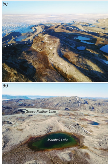
300 Figure 4: (a) View to the northeast in the Qamanaarsuup Sermia region (Fig. 3). In the foreground is a Kapisigdlit stade moraine crest resting directly adjacent to the historical maximum extent of this sector of the GrIS (dashed line). The GrIS is in the background and, here, there has been minimal retreat from the historical maximum extent. (b) View to the southwest in the Qamanaarsuup Sermia region showing Marshall Lake and Goose Feather Lake. Note the color contrast between the two lakes. 305 Marshall Lake currently does not receive meltwater from the GrIS. Goose Feather Lake is currently a proglacial lake that receives silt-laden GrIS meltwater; the lake catchment currently extends beneath the modern GrIS footprint (Fig. 3a; Fig. 6).
