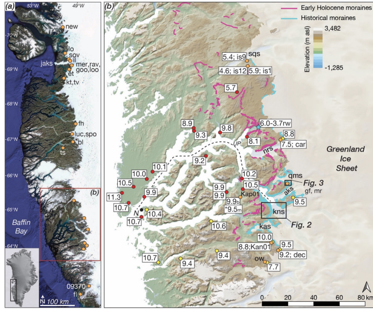
Figure 1: (a) Southwestern Greenland with the locations of proglacial-threshold lakes discussed in the text. Map data: Google, Landsat, U.S. Geological Survey. jaks = Jakobshavn Isbræ ( Sermeq Kujalleq ); new = Newspaper Lake (Cronauer et al., 2015); lo = Lake Lo (Håkansson et al., 2014); sov = South Oval Lake, il = Ice Boom Lake, mer = Merganser Lake, rav = Raven Lake, goo = Goose Lake, loo = Loon Lake, et = Eqauiut taserssuat (Briner et al., 2010); kt = Kuussuup Tasia, tv = Tininnillik Valley (Kelley et al., 2012); fh = Four Hare Lake (Lesnek et al., 2020); luc = Lake Lucy, spo = Sports Lake (Young and Briner, 2015; Lesnek et al., 2020 ); bl = Baby Loon Lake, ts = Tasersuaq (Lesnek et al., 2020); 09379, fl = Frederikshåb Isblink (Larsen et al., 2015). (b) Nuuk (N) region with existing radiocarbon ages (red dots) and ^{10}\text{Be} ages (yellow dots) in ka BP (CE 1950) that constrain the timing of regional deglaciation. The Kapisigdlit stade moraines are shown in pink and historical moraines are in blue (modified from Pearce et al., 2018). For figure clarity we only show the mean deglaciation age at each location without uncertainties; see Table S1 (radiocarbon) and Table S2 ( ^{10}\text{Be} ) for details. Also shown are the locations of proglacial-threshold lakes discussed in the text (orange dots) and location of marine bivalves reworked into the historical maximum ( blue star ) near Ujarassuit Paavat (up; Weidick et al., 2012; rw = reworked ). The dotted line marks the flowline used to assess model-data fit in Fig. 17. is1, is9, is12, (Levy et al., 2017); car = Caribou Lake, gf = Goose Feather Lake (Lesnek et al., 2020); mr = Marshall Lake (this study); dec = Deception Lake, ow = One-way Lake (Lesnek et al., 2020); Kan01 (Larsen et al., 2015); Kap01 (Larsen et al., 2014 and this study); b = bulk sediments; m = macrofossils. Glaciers: kns = Kangiata Nunaata Sermia; kas = Kangasarsuup Sermia; aks = Akullersuup Sermia; qms = Qamamaarsuup Sermia; nrs = Narsap Sermia; sqs = Saqqap Sermia.
