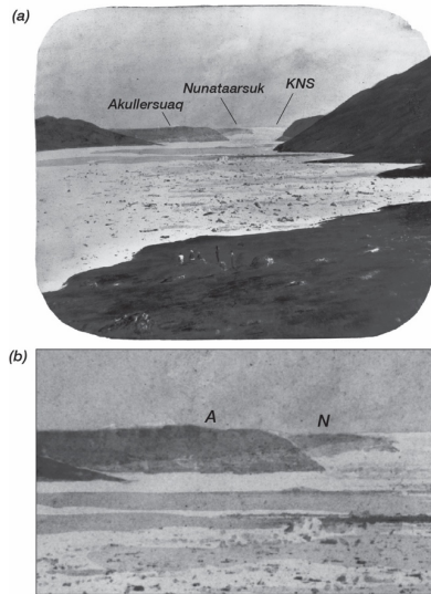
Figure 10: (a) Photograph looking upfjord towards KNS taken some time in the 1850s by Danish geologist Hinrich Rink (Weidick et al., 2012). Our northeastern KNS field site (Fig. 9) is located on the distal side of Nunataarsuk. (b) Close up of Akullersuaq (A) and Nunataarsuk (N) that captures the trim-line marking the historical maximum extent of KNS. Photograph is housed in the archives of the National Museum in Copenhagen. Digital copy was graciously provided by O. Bennike.
