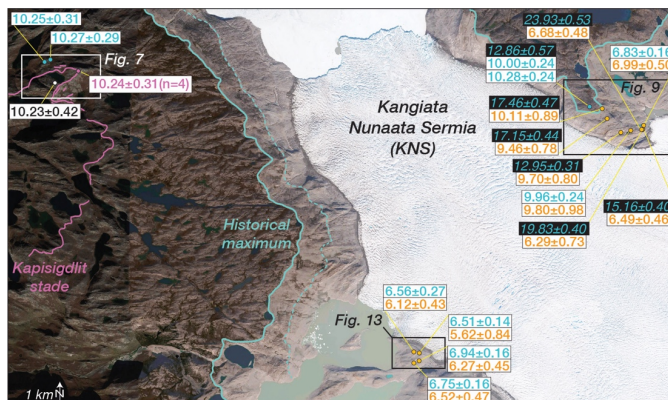
Figure 2: Kangiata Nunaata Sermia with the Kapisigdlit stade moraines (pink) and the historical maximum extent (blue), which is marked by prominent moraines and trim_lines. The dashed line marks the CE 1920 stade. For figure clarity, we only show ^{10}\text{Be} ages (ka BP \pm 1 S.D.) that constrain deposition of the Kapisigdlit stade moraine and do not include outliers; see Fig. 7 and Table S3 for a detailed view and the complete ^{10}\text{Be} dataset. For bedrock samples located inside the historical maximum extent, ^{10}\text{Be} ages (ka BP \pm 1 S.D.) are shown in blue text, and the corresponding in situ ^{14}\text{C} age from the same sample is in orange text (ka BP \pm 1 S.D.). ^{10}\text{Be} ages influenced by isotopic inheritance are in italics with black boxes. More detailed views of the bedrock sampling locations and the corresponding ^{26}\text{Al}/^{10}\text{Be} ratios are shown in Fig. 9 and Fig. 13. Map data: Google, Maxar Technologies.
