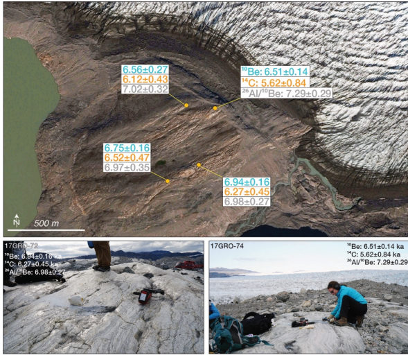
Figure 13: ^{10}\text{Be} ages and in situ ^{14}\text{C} ages (ka BP \pm 1 S.D.), and measured ^{26}\text{Al}/^{10}\text{Be} ratios at each bedrock sample site on the southwestern side of KNS. Also shown are representative bedrock sample sites 17GRO-72 and -74. Map data: Google, Maxar Technologies.
