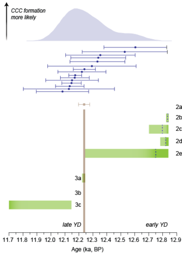
620 Figure 5: ^{230}\text{Th} ages of CCC and their 2\sigma uncertainties from Cioccherloch (blue bars) and CCC formation “windows” as suggested by model scenarios for the early and late YD. Calculated Kernel density function of the ^{230}\text{Th} ages shows the likelihood of CCC formation (blue shaded area). The green bars mark the -1 to 0^\circ\text{C} window of possible CCC formation at the depth of the CCC site. The blue dashed vertical lines mark the -0.5^\circ\text{C} isotherm at 50 m depth (2c-2e). The brown vertical line and age with the 2\sigma error bar mark the timing of the mid-YD transition at Meerfelder Maar (Lane et al., 2013).
