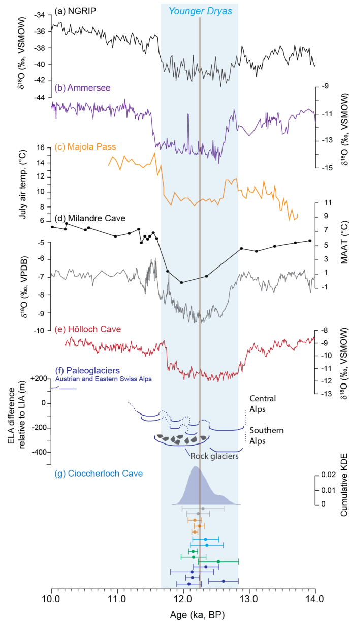
630 Figure 6: CCC ages from Ciochcherloch (g) compared to YD proxy records in Europe and Greenland plotted on their published 635 chronology. (a) NGRIP \delta^{18}\text{O} data (Rasmussen et al., 2014), (b) lacustrine benthic ostracod \delta^{18}\text{O} data from Ammersee (von Grafenstein et al., 1999). YD paleotemperature reconstructions are shown by (c) chironomid-inferred July air temperatures from the Majola Pass (Ilyashuk et al., 2009) and by (d) MAAT inferred from fluid inclusion stable isotope data of stalagmites and speleothem \delta^{18}\text{O} data from Milandre Cave (Affolter et al., 2019). CCC ages are compared to speleothem \delta^{18}\text{O} data from Hölloch Cave and (f) extent of Central and Southern Alpine paleoglaciers (Heiri et al., 2014b). Calculated Kernel density function of all ^{230}\text{Th} ages is shown by the blue shaded area (g). Dark blue and green refer to ^{230}\text{Th} ages of CCCs from heap A and B, respectively (f). Data from heaps C, D and E are shown in light blue, orange, and grey, respectively (g). The brown vertical line mark the mid-YD transition recorded at Meerfelder Maar (Lane et al., 2013).
