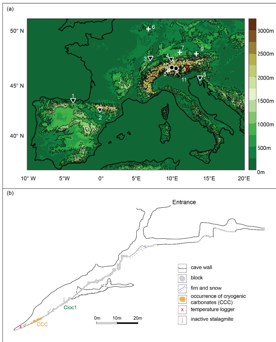
Figure 1: Relief map of Europe showing the location of Cioccherloch (red triangle) and other European YD speleothem (black triangle), lacustrine (white cross) and palaeoglacier (black circle) records (a) mentioned in the text (1 –La Garma cave, 2 – Seso cave, 3 – Milandre Cave, 4 –Bärenhöhle, 5 –Savi Cave, 6 –Meerfelder Maar, 7 – Lake Ammersee, 8 –Majola Pass, 9 – Mondsee 10 –Err-Julier and Julier Pass, 11 –Ortles). Vertical cross section of Cioccherloch Cave showing the CCC findings in the terminal chamber (b).
