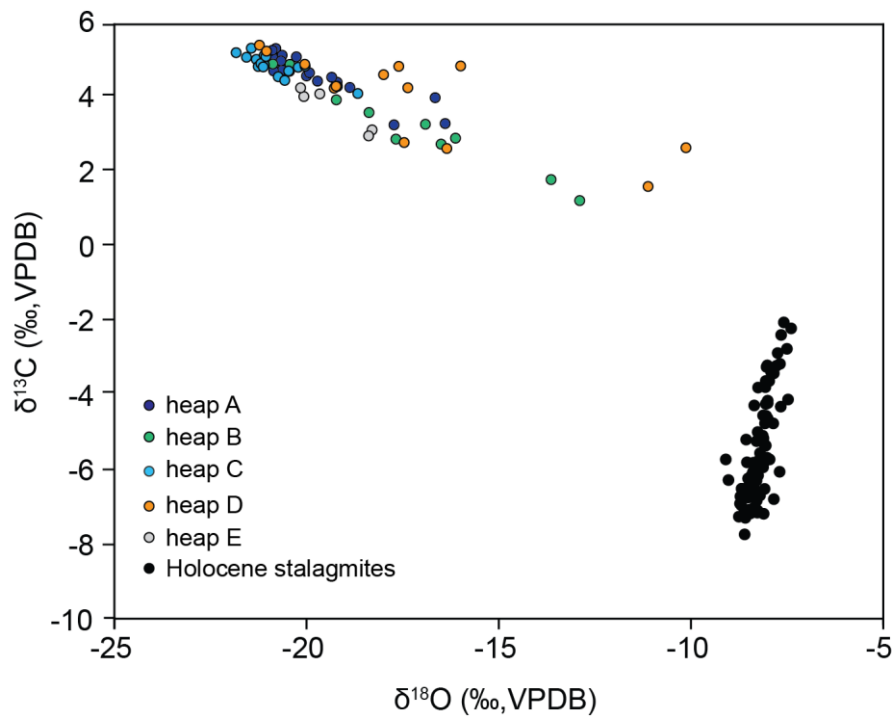
Figure 2: Stable isotope composition of CCCs from Ciocherloch Cave. Samples from different CCC heaps are color-coded. Values of two Holocene stalagmites from the same cave gallery are shown for comparison (unpublished data by the authors).
