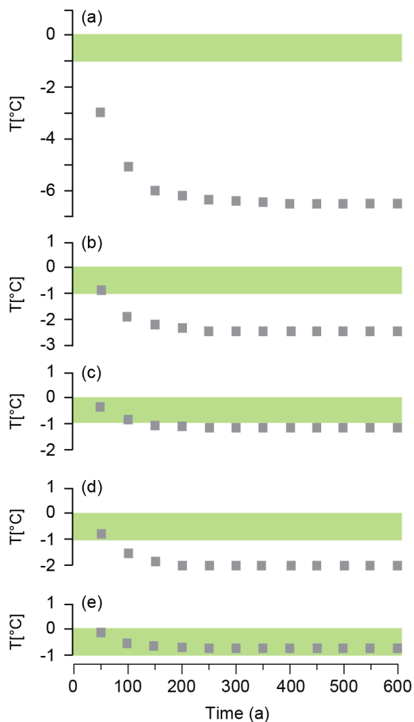
605 Figure 3: Thermal models 2a to 2e simulating the development and deepening of the permafrost during the early YD. Modeling results depict the ground temperature at 50 m depth at the depth of the CCC site in Cioccherloch. These models use the temperature profile of scenario 1 as initial condition. Model 2a (a) is forced with a MAAT of -6.5^\circ\text{C} . Models 2b (b) and 2c (c) use a MAAT of -2.5^\circ\text{C} and the latter simulates the impact of a winter snow cover resulting in the attenuation of the winter cold by 5^\circ\text{C} (i.e. snow \Delta T = 5^\circ\text{C} ). Scenarios 2d (d) and 2e (e) model the changes of the thermal profile at the CCC site using a MAAT of -1.5^\circ\text{C} . Scenario 2e considers the presence of a winter snow pack resulting in snow \Delta T of 4.7^\circ\text{C} . The green horizontal bar marks the -1 to 0^\circ\text{C} “window” of possible CCC formation for the depth range of the CCC site in this cave.
