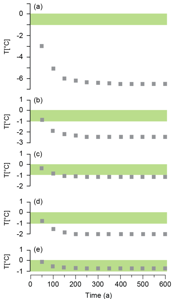
Figure 3: Thermal models 2a to 2e simulating the development and deepening of the permafrost during the early YD. Modeling results depict the ground temperature at 50 m depth at the depth of the CCC site in Cioccherloch. These models use the temperature profile of scenario 1 as initial condition. Model 2a (a) is forced with a MAAT of -6.5^{\circ}\text{C} . Models 2b (b) and 2c (c) use a MAAT of -2.5^{\circ}\text{C} and the latter simulates the impact of a winter snow cover resulting in the attenuation of the winter cold by 5^{\circ}\text{C} (i.e. \text{snow } \Delta T = 5^{\circ}\text{C} ). Scenarios 2d (d) and 2e (e) model the changes of the thermal profile at the CCC site using a MAAT of -1.5^{\circ}\text{C} . Scenario 2e considers the presence of a winter snow pack resulting in \text{snow } \Delta T of 4.57^{\circ}\text{C} . The green horizontal bar marks the -1 to 0^{\circ}\text{C} “window” of possible CCC formation for the depth range of the CCC site in this cave.
