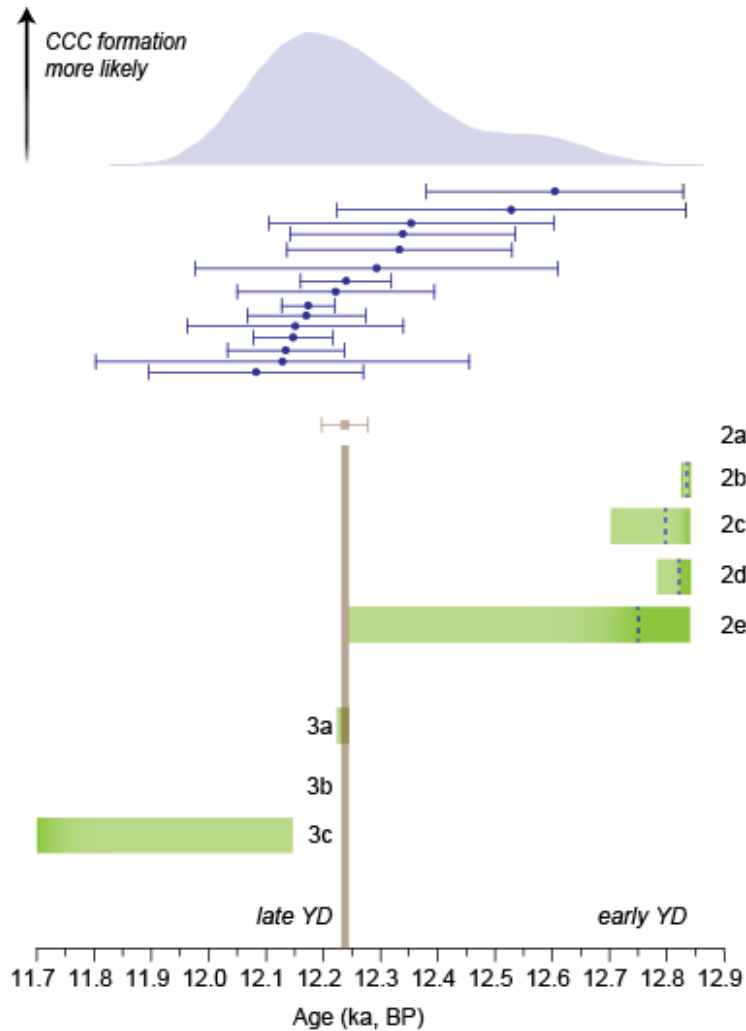
660 Figure 5: ^{230}\text{Th} ages of CCC and their 2\sigma uncertainties from Cioccherloch (blue bars) and CCC formation “windows” as suggested by model scenarios for the early and late YD. Calculated Kernel density function of the ^{230}\text{Th} ages shows the likelihood of CCC formation (blue shaded area). The green bars mark the -1 to 0^\circ\text{C} window of possible CCC formation at the depth of the CCC site. The blue dashed vertical lines mark the -0.5^\circ\text{C} isotherm at 50 m depth (2c-2e). The brown vertical line and age with the 2\sigma error bar mark the timing of the mid-YD transition at Meerfelder Maar (Lane et al., 2013).
