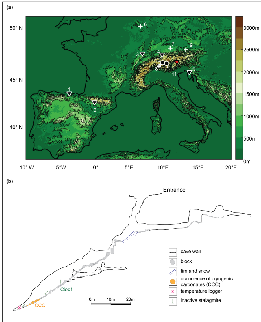
630 Figure 1: Relief map of Europe showing the location of Cioccherloch (red triangle) and other European YD speleothem (black triangle), lacustrine (white cross) and palaeoglacier (black circle) records (a) mentioned in the text (1 –La Garma cave, 2 – Seso cave, 3 – Milandre Cave, 4 –Bärenhöhle, 5 –Savi Cave, 6 –Meerfelder Maar, 7 – Lake Ammersee, 8 –Majola Pass, 9 – Mondsee 10 –Err-Julier and Julier Pass, 11 –Ortles). Vertical cross section of Cioccherloch Cave showing the CCC findings in the terminal chamber (b).
