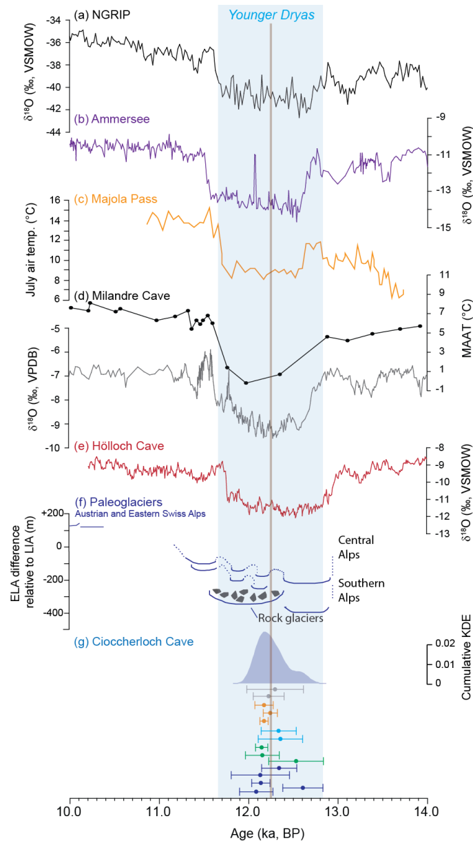
Figure 6: CCC ages from Cioccherloch (fg) compared to YD proxy records in Europe and Greenland plotted on their published chronology. (a) NGRIP \delta^{18}\text{O} data (Rasmussen et al., 2014), (b) lacustrine benthic ostracod \delta^{18}\text{O} data from Ammersee (von Grafenstein et al., 1999). YD paleotemperature reconstructions are shown by (c) chironomid-inferred July air temperatures from the Majola Pass (Ilyashuk et al., 2009) and (e) Mondsee (Lauterbach et al., 2011) and by (d) speleothem \delta^{18}\text{O} data and MAAT inferred from fluid inclusion stable isotope data of stalagmites and speleothem \delta^{18}\text{O} data from Milandre Cave (Affolter et al., 2019). CCC ages are compared to speleothem \delta^{18}\text{O} data from Hölloch Cave and (fe) extent of Central and Southern Alpine paleoglaciers (Heiri et al., 2014b). Calculated Kernel density function of all ^{230}\text{Th} ages is shown by the blue shaded area (g). Dark blue and green refer to ^{230}\text{Th} ages of CCCs from heap A and B, respectively (f). Data from heaps C, D and E are shown in light blue, orange, grey and light blue-grey, respectively (gf). The brown vertical line mark the mid-YD transition recorded at Meerfelder Maar (Lane et al., 2013).
