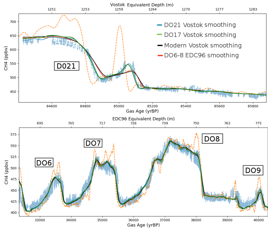
Figure 10. Comparison of smoothing resulting from for the three different glacial age distributions, and the modern Vostok GAD constrained with firm air pumping data. Atmospheric references (dashed lines) have been smoothed by the four different GADs and are displayed overlying the measurements (light blue). The upper panel shows the DO21 event as measured in Vostok, and the lower panel shows the DO-6 to 9 as measured in EDC96.
