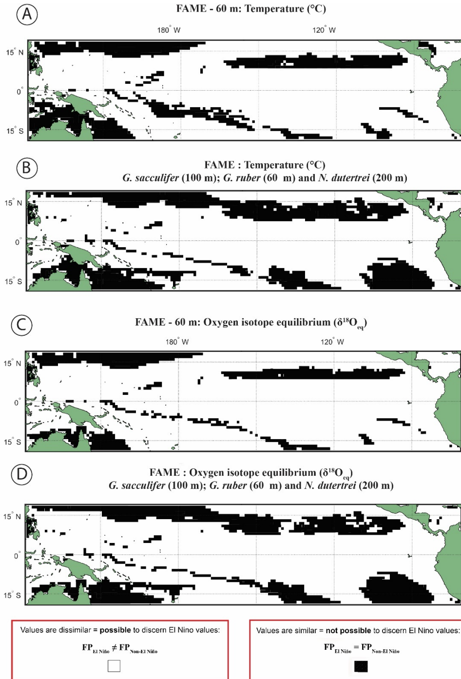
5 Figure 2 Anderson-Darling results plotted regionally in which species-specific results are overlain, for each plot the results represent where at least one species shows that it may not be possible to discern El Niño Values. Panels represent water depth locations where dissimilar and similar values for the two climate states for (a-b) FAME- T_c modelled temperature (c-d) FAME- \delta^{18}\text{O}_c modelled oxygen isotope values recorded in the calcite shells ( T_c ) occur. Each panel represents the Anderson-Darling test
