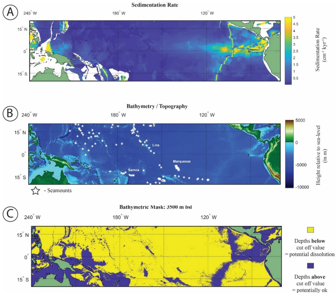
Figure 5 (A) Map of the sedimentation rate and bathymetry of the Tropical Pacific. (A) Inferred sedimentation rate (Olson et al. 2016). White regions represent continental shelf. (B) GEBCO map of height relative to 0 m with location of seamounts plotted (white stars). (C) A binary colour map of the GEBCO data, yellow is values below cut-off depth value (3500 m below sea-level (bsl)) and purple above the cut-off depth value. See Supplementary Figure 8 for variation in cut-off values.
