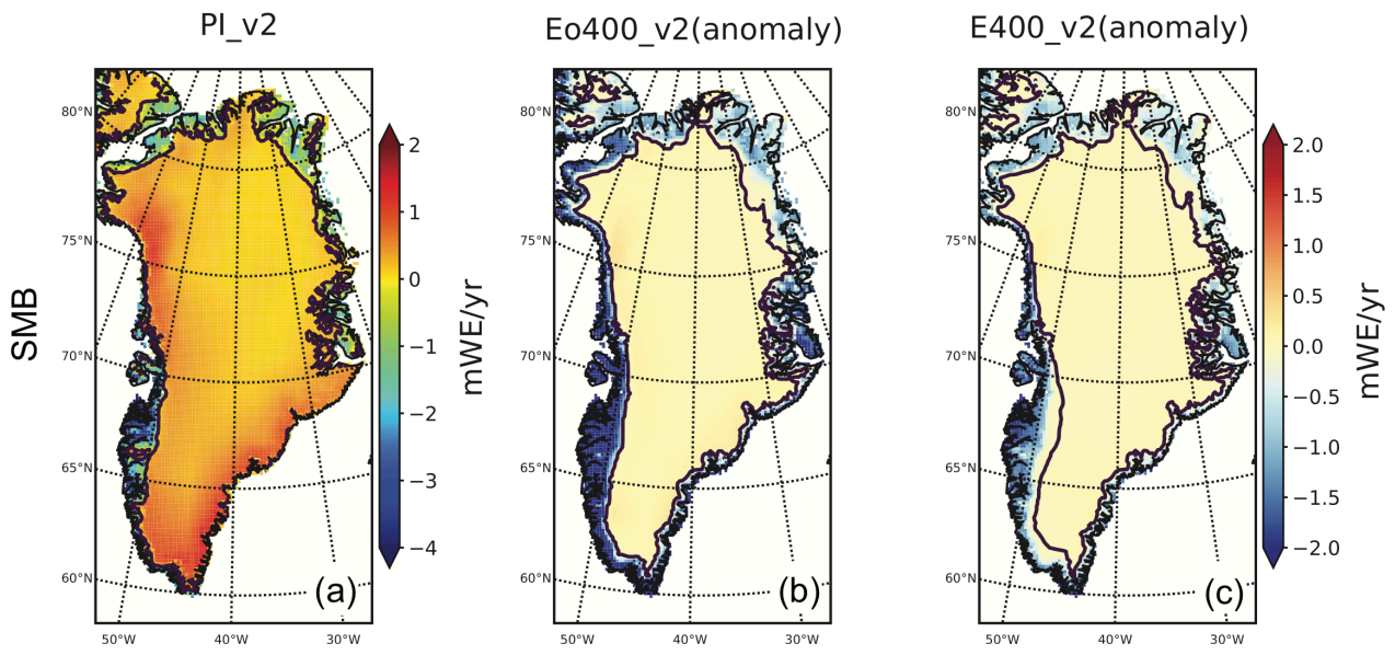
Figure 10: Mean annual surface mass balance (SMB) in Greenland in PI control experiment (a) and the anomalies of SMB in Eo400_v2 (b) and E400_v2 (c) experiments in comparison with PI control (unit: mWE (water equivalent)/yr). Contour line indicates the zero value.
