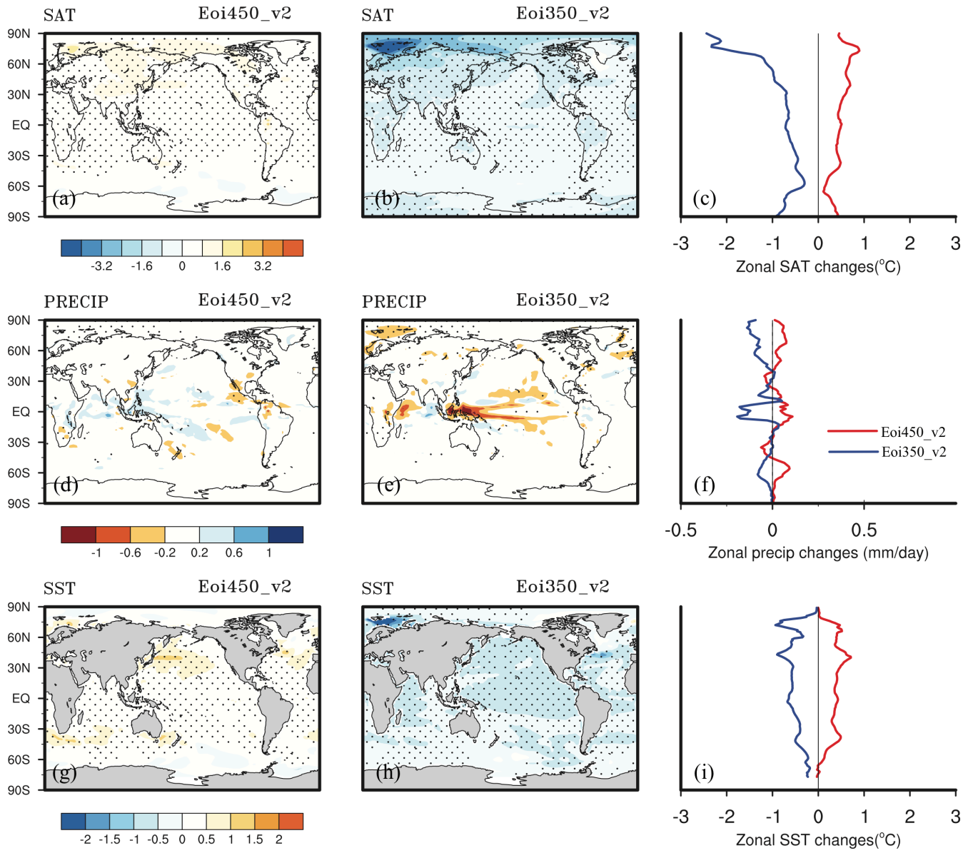
5 Figure 11: Anomalies of mean annual SAT, mean annual precipitation rate and mean annual SST for Eoi450_v2(a, d, g), Eoi350_v2(b, e, h) in comparison with Eoi400_v2. The last column (c, f, i) of this panel shows the zonal mean of related anomalies (red and blue lines represent respectively for the results of Eoi450_v2 and Eoi350_v2). Stippling indicates regions where results are statistically significant at 99% confidence criteria.
