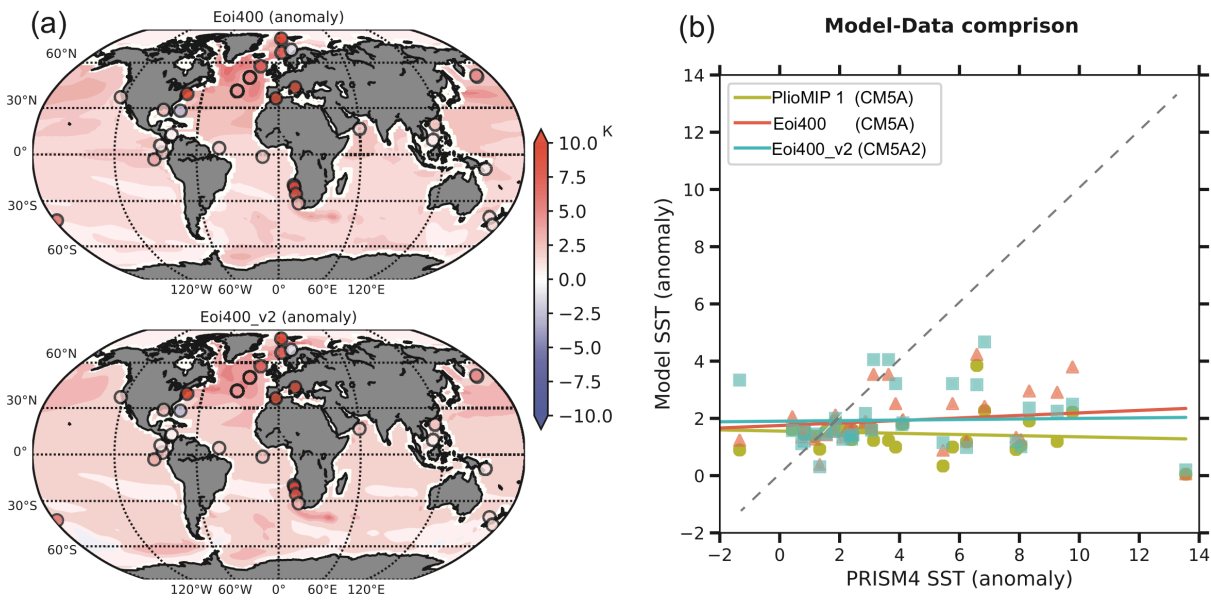
5 Figure 12: SST model data comparison. (a) Modelled mean annual SST anomalies of MIS KM5c (in relative to PI controls, shaded area) and reconstructed MIS KM5c SST anomalies (in relative to near pre-industrial data, circle markers ). (b) The relationship between modelled SST anomalies and PRISM4 data anomalies.
