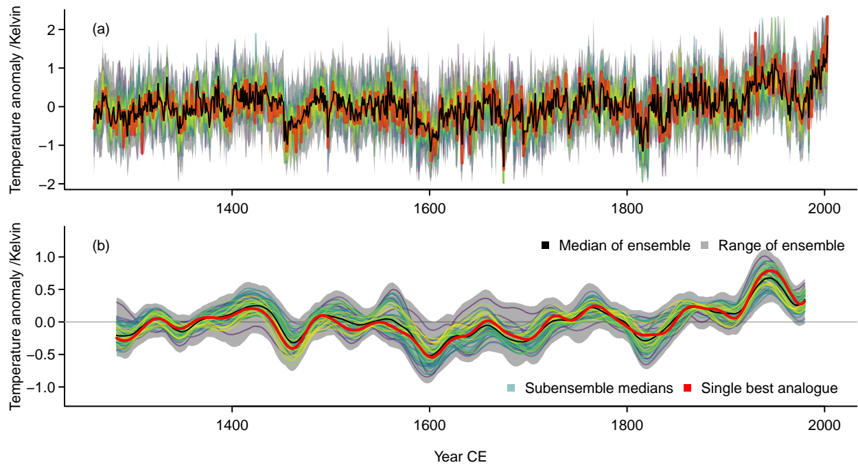
Figure 11. Ensemble of subsampled reconstructions: (a) Interannual data, (b) data smoothed with 47-point Hamming filter. Both panels show in grey the full range of 6500 reconstructions based on 4 proxies and only half of the simulated fields, in black the median of all 6500 reconstructions, and in red the single best analogue reconstruction based on the full data. Further colored lines are medians of the 65 subensembles using different sets of 4 proxies. Panel (b) adds a zero line as visual assistance.
