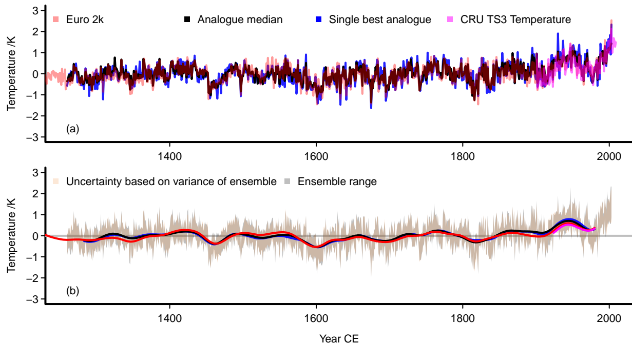
Figure 7. The analogue reconstruction for the 39 best analogues: (a): the interannual rescaled temperature reconstruction median in black; the blue line is the single best-analogue reconstruction; the red line is the Euro 2k-reconstruction; magenta is the CRU temperature adjusted to the mean of the reconstruction-median over the CRU period. (b): the unsmoothed uncertainty, estimates in light grey are the ensemble range, and the brown envelope gives a two standard deviation interval based on the variance of the 39 samples; note that both uncertainty estimates are hardly distinguishable on this scale, the panel adds the series from (a) but for 47-point Hamming filtered data. Panel (b) adds a zero line as visual assistance.
