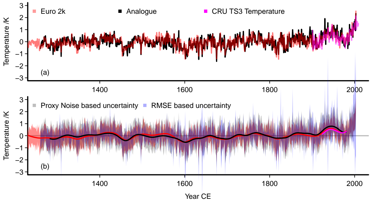
Figure 2. The best-analogue reconstruction relative to its full period mean: (a) the interannual temperature reconstruction in black, the red line is the area mean Euro 2k-reconstruction, magenta is the observational CRU temperature adjusted to the mean of the reconstruction over its time-range. The analogue reconstruction is rescaled by the variability from one of the simulations. (b) : as (a) but for 47-point Hamming filtered data; we further add the uncertainty for estimates for the interannual data: red is the unsmoothed Euro 2k-uncertainty, the grey envelope is a 2 standard-deviation uncertainty based on the correlation between the proxies and the observations at the proxy locations, the blue envelope is a 2 standard-deviation uncertainty based on a MSE-estimate. Panel (b) adds a zero line as visual assistance.
