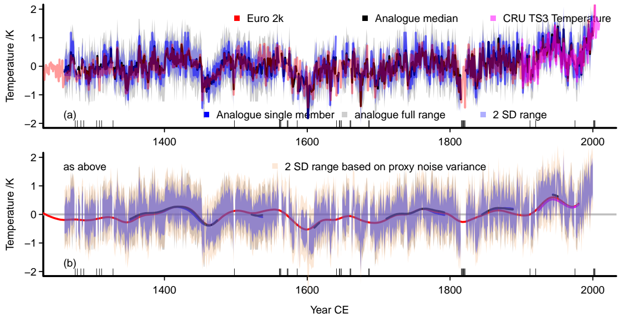
Figure 8. Analogue reconstruction based on an 1SD_{noi} uncertainty of the proxies. (a): Interannual data: red, the Euro 2k-reconstruction; black, the analogue median; blue line, a single analogue member, blue shading, two standard deviation uncertainty range around the analogue median based on variability of the analogues, grey shading, the full range of analogues; marks at horizontal axis mark unsuccessful analogue searches. (b): As (a) for 47-point Hamming filtered data, but we add a two standard deviation uncertainty based on the square root of the proxy noise variances in brown as also shown in Figure 2. Panel (b) adds a zero line as visual assistance.
