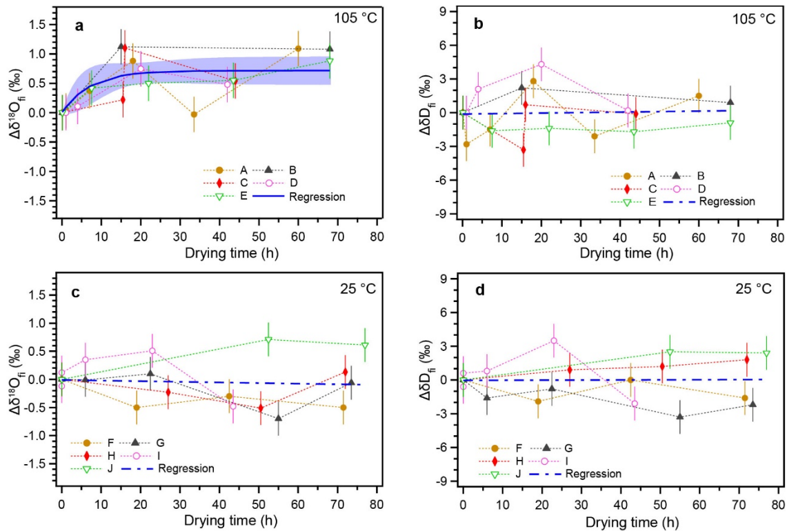
Figure 2: Changes in isotopic compositions of inclusion water with increasing drying time.
