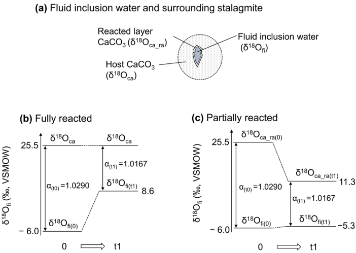
Figure 5: Schematic illustration of isotopic re-equilibration between inclusion water and stalagmite.
