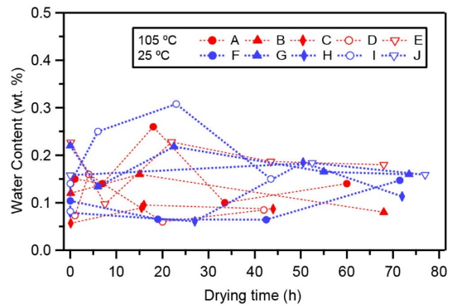
Figure 3: Changes in water content with increasing drying time.
