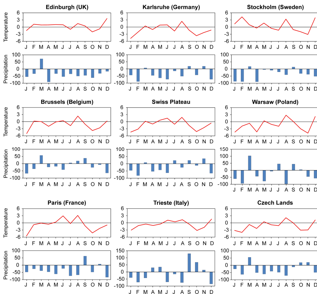
Figure 4. Annual variation of air temperature and precipitation in 1842 for selected European meteorological stations and regions. Temperatures are expressed as deviations from the 1961–1990 reference period, precipitation totals as percentages of corresponding 30-year means
