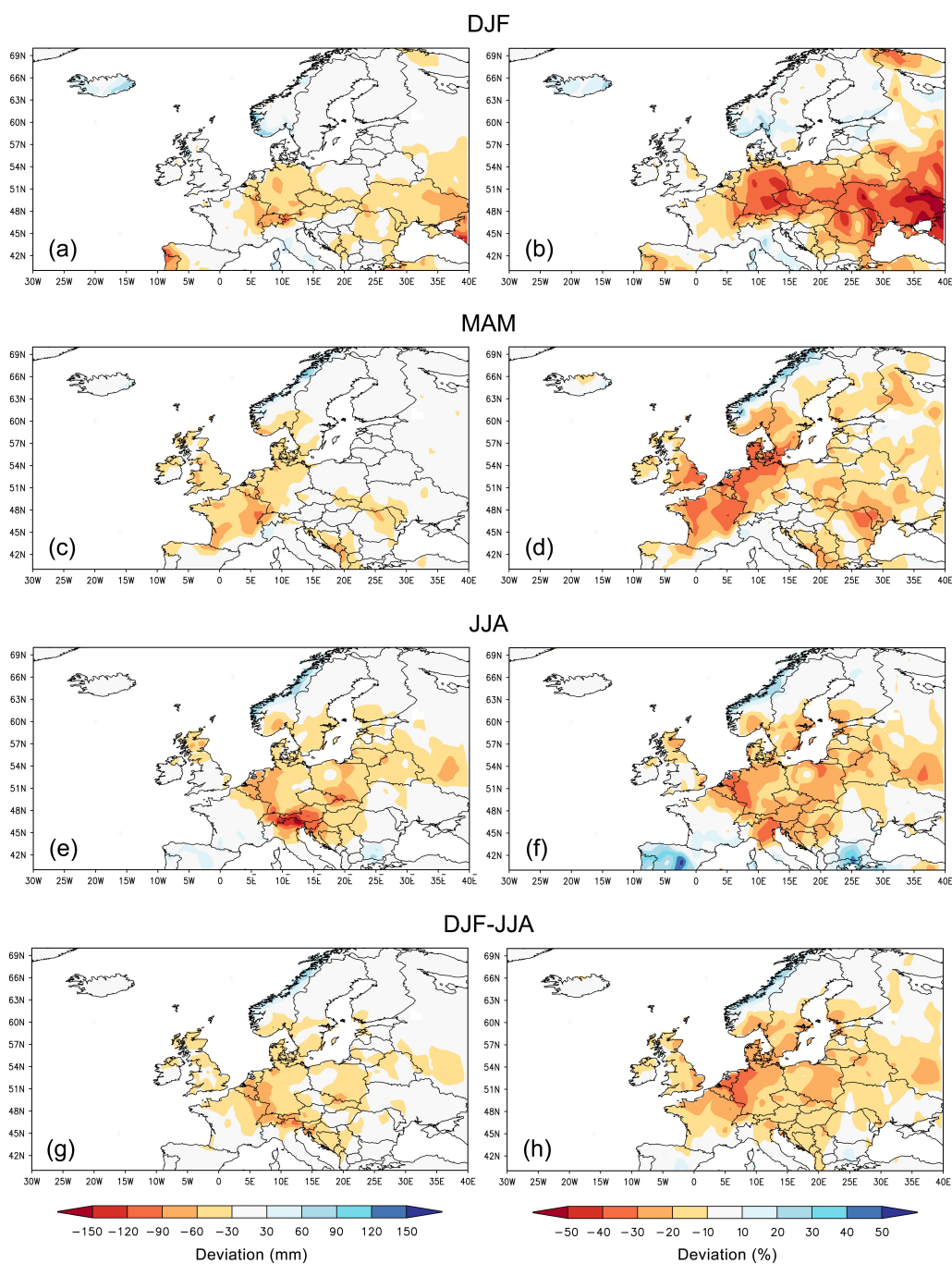
Figure 2. Precipitation patterns of DJF (a), MAM (c), JJA (e) and DJF-JJA (g) and their expression as percentages of the corresponding parts of the seasonal means in the 1961–1990 reference period (b, d, f, h) over the European lands (data from Pauling et al., 2006)
