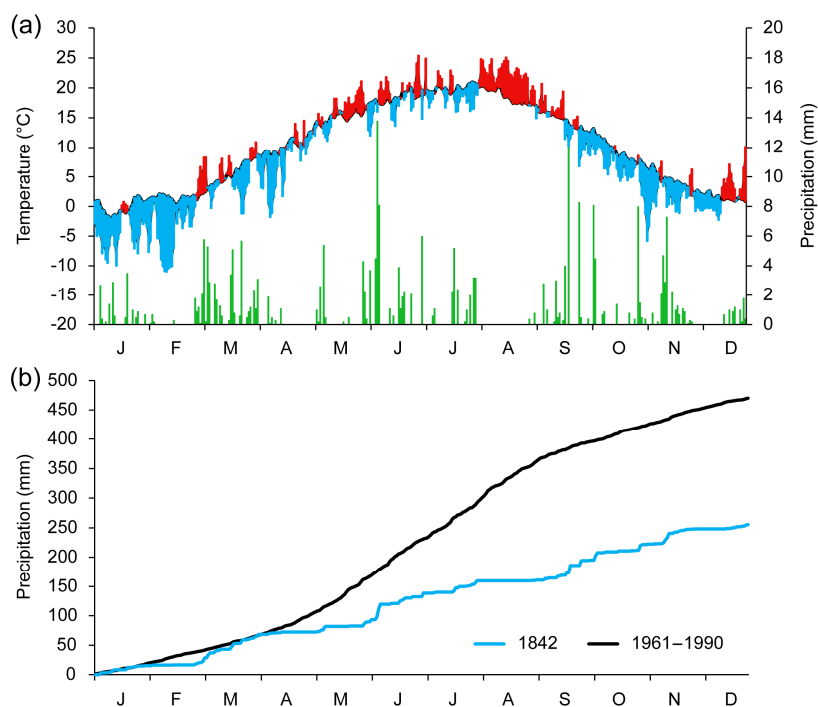
5 Figure 3. Temperature and precipitation for 1842 at the Prague-Klementinum station: (a) annual variation of daily mean temperatures (compared with the 1961–1990 mean variation) and daily precipitation totals for 1842; (b) cumulative daily precipitation totals for 1842 in comparison with the 1961–1990 reference period
