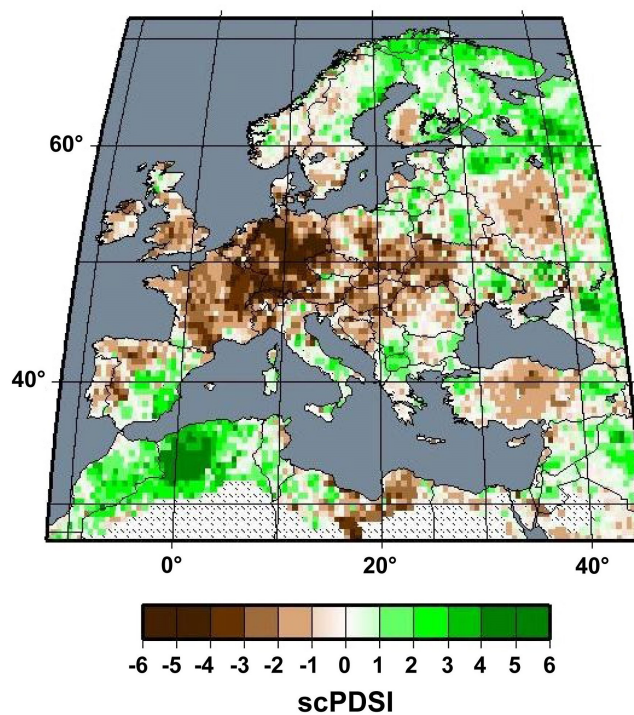
Figure 9. Values of summer scPDSI for 1842 in the European area as derived from tree-rings in OWDA (Cook et al., 2015)
