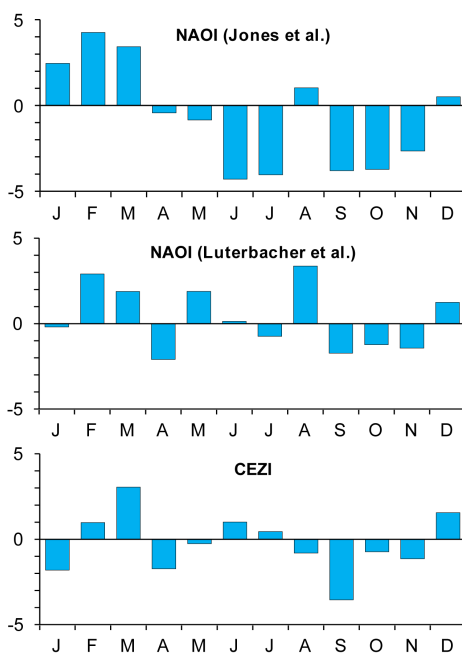
Figure 7. Annual variation of mean monthly NAOI (Jones et al., 1997; Luterbacher et al., 1999) and CEZI (Jacobeit et al., 2001) in 1842
