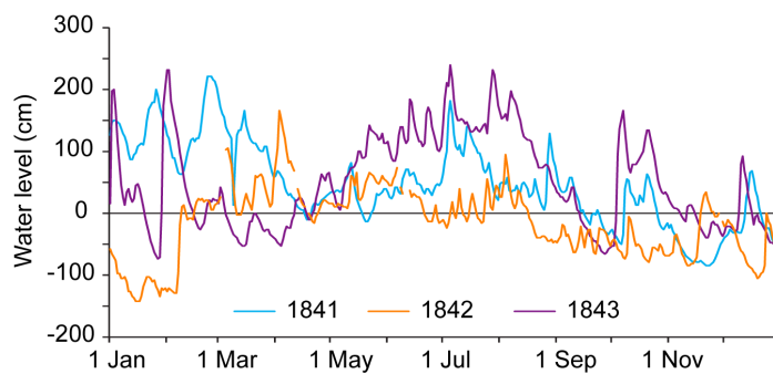
Figure 8. Annual fluctuations in daily water levels of the Danube at Vienna in the profile of the Great Danube Bridge during the years 1841, 1842 and 1843 (data extracted from Wiener Zeitung )
