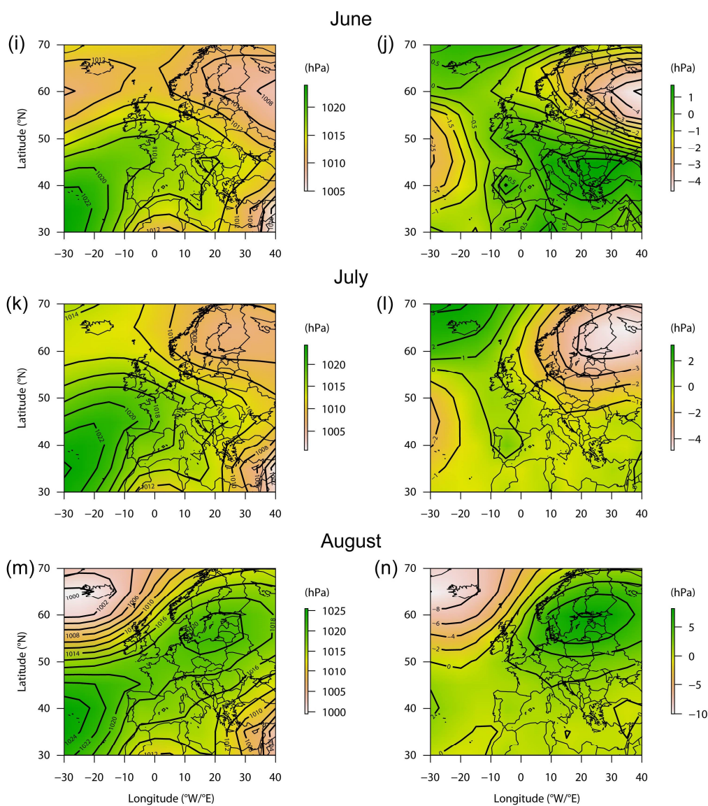
Figure 6. Mean sea-level pressure and deviations with respect to the reference 1961–1990 period means in the European-Atlantic area for the months of January (a,b), February (c,d), April (e,f), 5 May (g,h), June (i,j), July (k,l) and August (m,n) 1842
