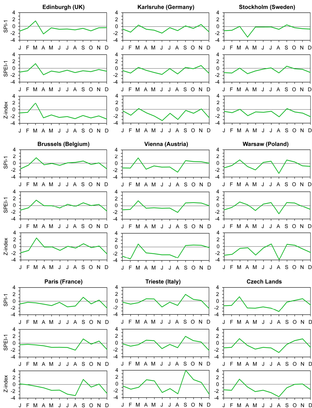
Figure 5. Annual variation of SPI-1, SPEI-1 and Z-index for selected European stations and regions in 1842
