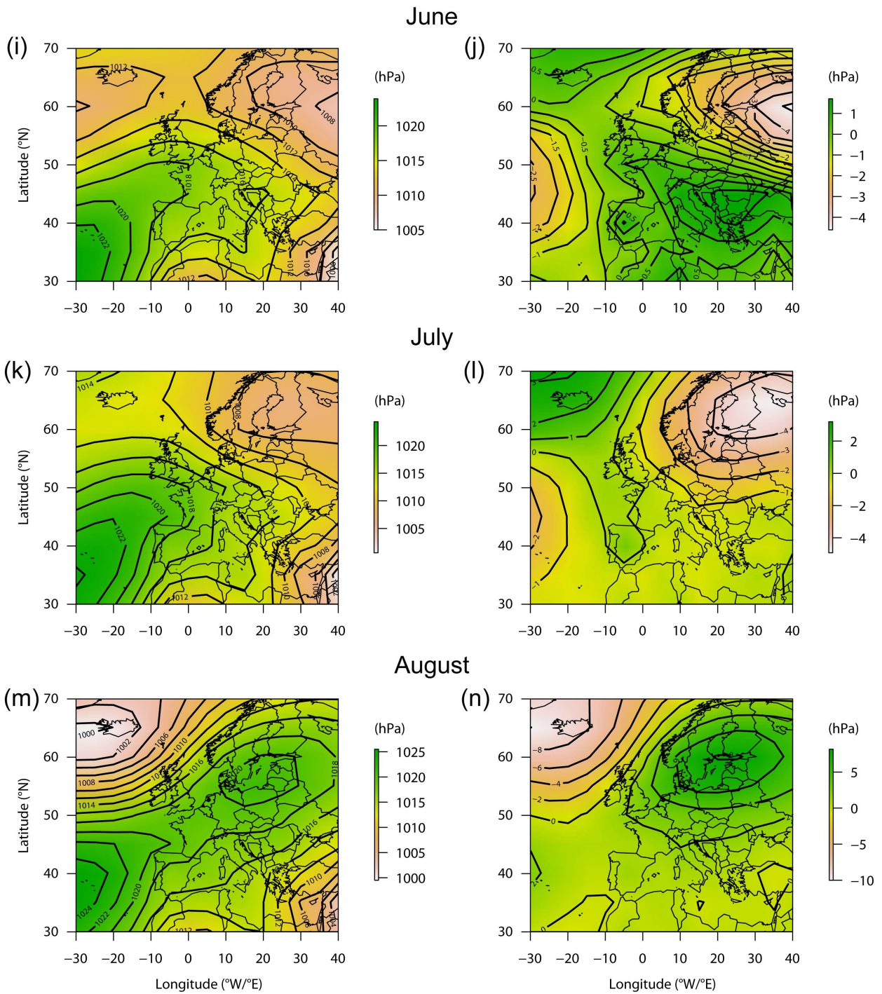
Figure 7. Mean sea-level pressure and deviations with respect to the reference 1961–1990 period means in the European-Atlantic area for the months of January (a,b), February (c,d), April (e,f), 5 May (g,h), June (i,j), July (k,l) and August (m,n) 1842
