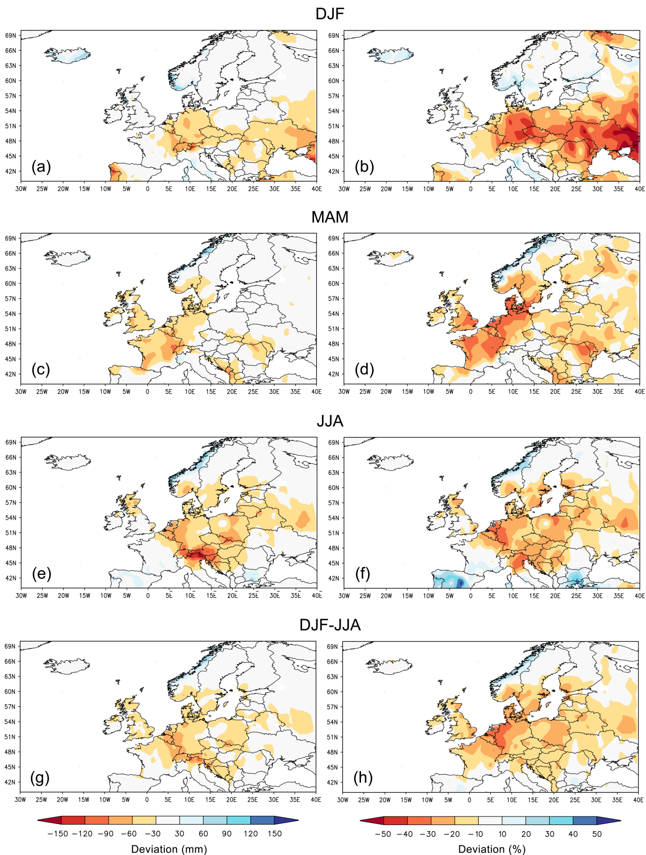
Figure 3. Precipitation patterns of DJF (a), MAM (c), JJA (e) and DJF-JJA (g) and their expression as percentages of the corresponding parts of the seasonal means in the 1961–1990 reference period (b, d, f, h) over the European lands (data from Pauling et al., 2006)
