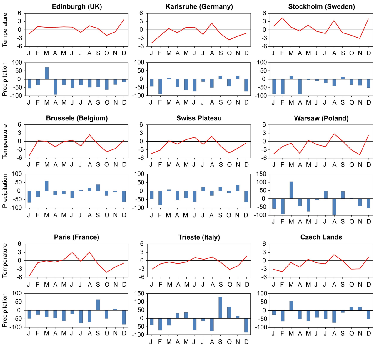
Figure 5. Annual variation of air temperature and precipitation in 1842 for selected European meteorological stations and regions. Temperatures are expressed as deviations from the 1961–1990 reference period, precipitation totals as percentages of corresponding 30-year means
