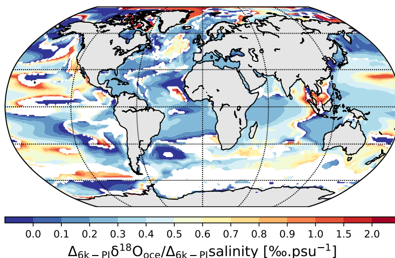
Figure 13. Spatial distribution of calculated temporal 6k–PI \delta^{18}\text{O}_{\text{oce}} –salinity gradients for oceanic grid cells where the 6k–PI absolute change in salinity is at least 0.02 psu.
