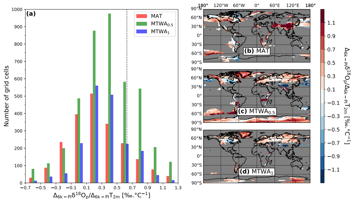
Figure 10. (a) Histogram of the calculated temporal 6k-PI \delta^{18}\text{O}_p-T gradients for all grid cells where (i) simulated mean temperature for both PI and 6k is lower than 20^\circ\text{C} and (ii) absolute change in temperature between the 6k and PI control simulations is at least 0.5^\circ\text{C} (MAT, \text{WTMA}_{0.5} ) or 1^\circ\text{C} ( \text{WTMA}_1 ). The dotted line shows the simulated mean spatial PI \delta^{18}\text{O}_p-T gradient of 0.63\text{‰}\cdot^\circ\text{C}^{-1} . The gradients are calculated in three different ways: with the annual mean \delta^{18}\text{O}_p and temperature values where |\Delta_{6k-PI}\text{MAT}| \geq 0.5^\circ\text{C} (MAT, red bars), with the mean \delta^{18}\text{O}_p and temperature values of the warmest month where |\Delta_{6k-PI}\text{WTMA}| \geq 0.5^\circ\text{C} ( \text{WTMA}_{0.5} , green bars), with the mean \delta^{18}\text{O}_p and temperature values of the warmest month where |\Delta_{6k-PI}\text{WTMA}| \geq 1^\circ\text{C} ( \text{WTMA}_1 , blue bars). Their spatial distribution is shown in (b), (c) and (d) respectively.
