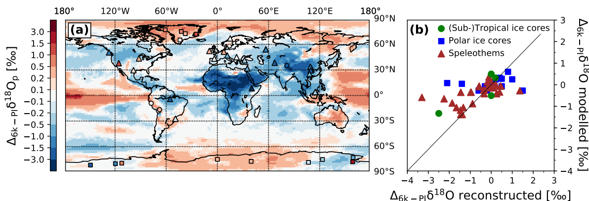
Figure 6. (a) Simulated global pattern of annual mean \delta^{18}\text{O}_p changes in precipitation between the mid-Holocene and PI climate and comparison with reconstructed \delta^{18}\text{O} changes in polar (squares) and (sub-)tropical (dots) ice cores and in calcite speleothems (triangles). (b) Reconstructed \delta^{18}\text{O} changes from ice cores and speleothems vs. simulated 6k–PI \delta^{18}\text{O} anomalies at the same location. The observed \delta^{18}\text{O} anomalies in polar and (sub-)tropical ice core records (blue squares and green dots respectively) are compared to the simulated 6k–PI \delta^{18}\text{O}_p changes in precipitation. The observed \Delta_{6k-PI}\delta^{18}\text{O} in speleothems (brown triangles) are compared to simulated \delta^{18}\text{O}_c changes in calcite (see text).
