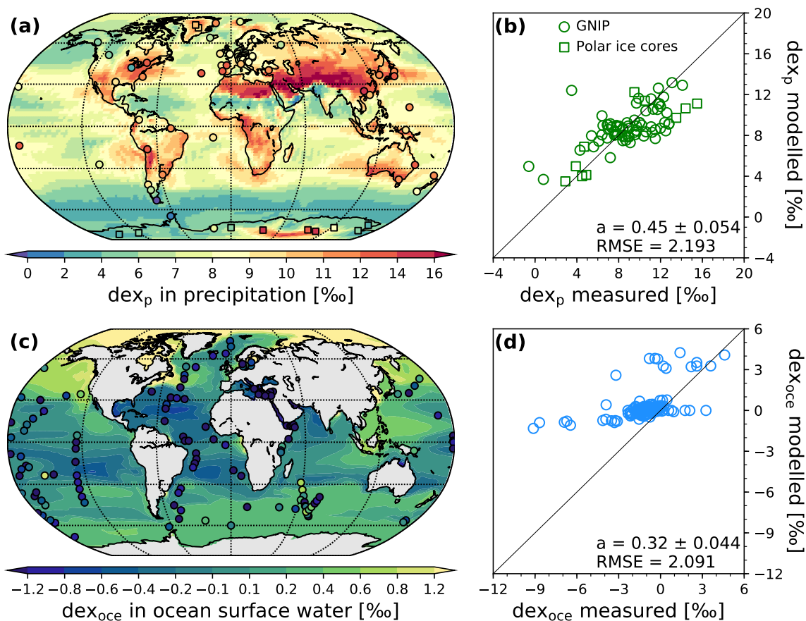
Figure 4. Global distribution of simulated and observed annual mean dex values in precipitation (a) and ocean surface waters (c). Scatter plots of modeled vs. observed annual mean deuterium excess values in precipitation (b) and ocean surface waters (d) are shown. The gradients and RMSE of the linear regression fits are given in the legend.
