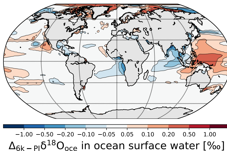
Figure 7. Modeled annual mean \delta^{18}\text{O}_{\text{occ}} changes in ocean surface water between the mid-Holocene and PI climate.
