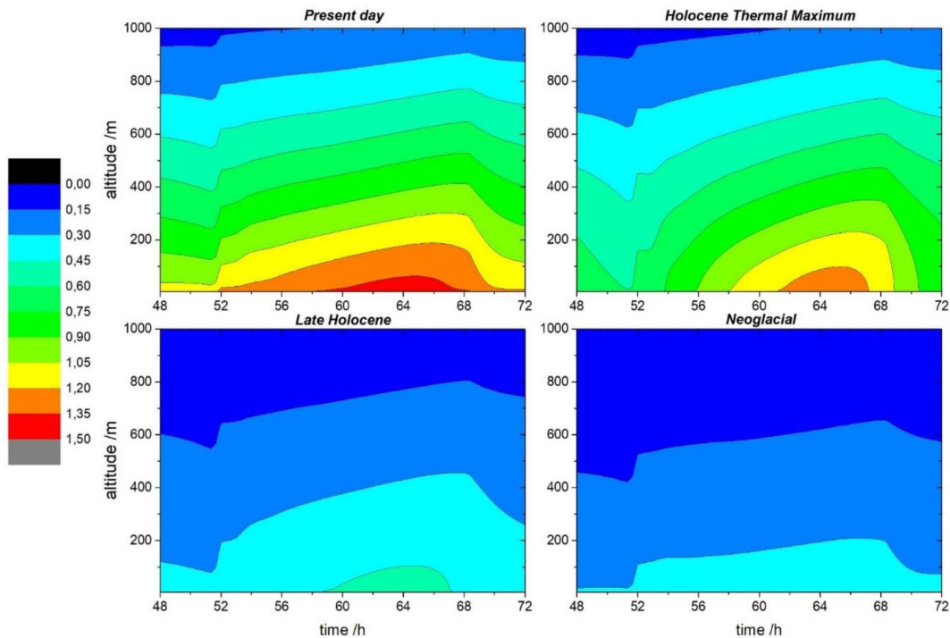
Fig. 1. Figure S3. Diurnal variation of reactive iodine modelled by THAMO in different scenarios of [O 3 ] and VSLs emissions fluxes
