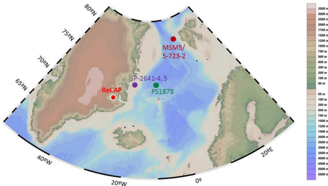
Fig. 2. Fig. 1: Location of the ReCAP ice core (red) and other marine paleoceanographic archives in the Nordic Seas discussed in the text.
