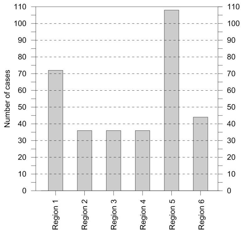
11 12 Fig. 3. Number of years with droughts in six geographical regions of Poland (including information 13 related to the whole country) 1451–1800. See Table 2 or Fig. 4 for names of regions.
