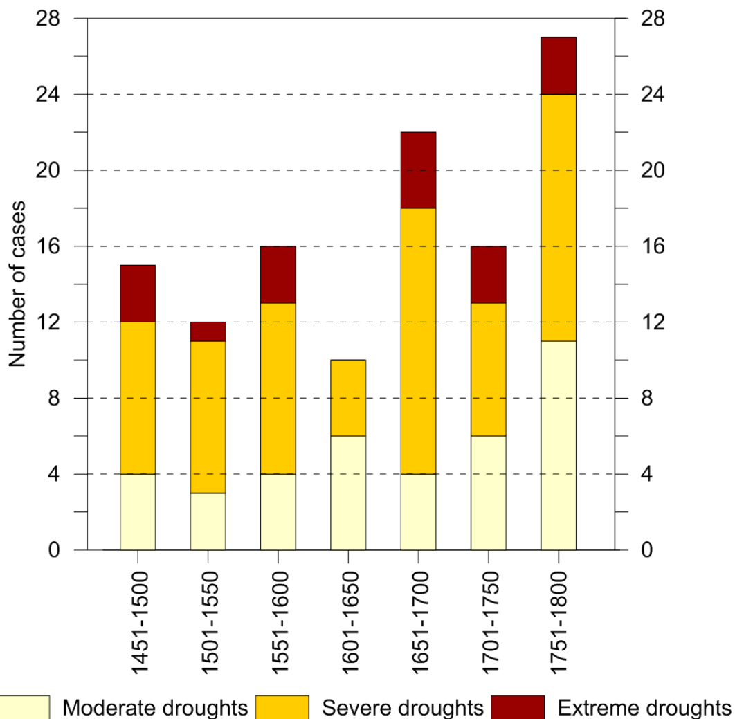
6 Fig. 5. Frequency of occurrence of three categories of droughts in Poland in 50-year periods, 1451– 7 1800
