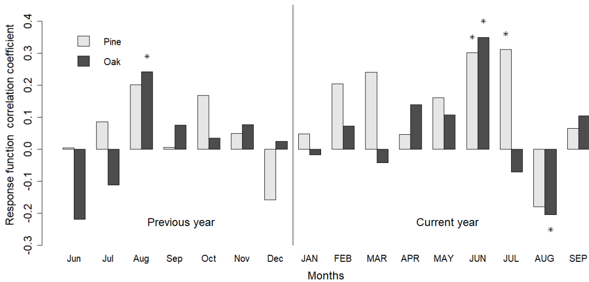
3 Fig. 2. Climate growth relationships between tree rings in pine (grey bars) and oak (black bars) 4 and monthly totals of precipitation. Key: Asterisks indicate statistically significant correlation 5 coefficients at the level of 0.05. Climate data were taken from Toruń Meteorological Station.
