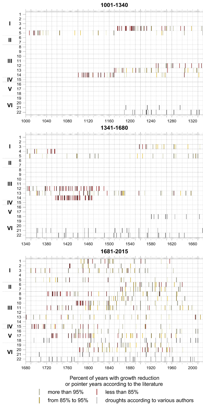
2 Fig. 6. Pointer years in Poland, 1001–2015
