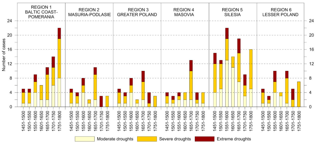
8 9 Fig. 4. Frequency of occurrence of three categories of droughts in six distinguished 10 geographical regions in Poland in 50-year periods, 1451–1800
