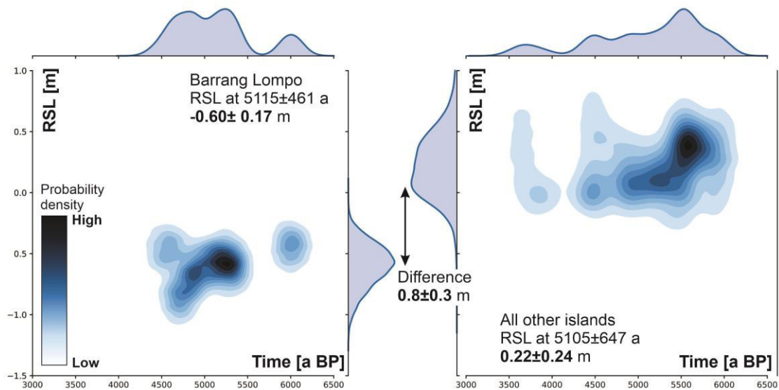
Figure 9: Joint plot showing bivariate (central plot) and univariate (marginal axes) distribution of RSL data points at Barrang Lompo (left) and all the other islands surveyed in this study and in Mann et al. (2016) (right). Darker blue areas in the central plots indicate a higher density of RSL point therefore darker colors indicate a higher probability of RSL at the given time. The Jupyter notebook used to create this graph is available as SM2.
