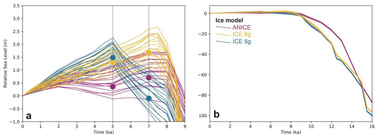
Figure 5: Results of the 54 GIA model runs for an island located in the center of the Spermonde Archipelago, a) last 9 ka. Dots indicate the points at which the maps in Figure 6 have been extracted. b) last 16 ka, representing the full time extent of the
