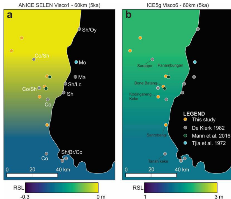
Figure 7: Location of the RSL data presented in this study, Mann et al. (2016), De Klerk (1982) and Tjia et al. (1972) compared with RSL as predicted by GIA models. Land areas are filled in black. Here we show the models predicting, respectively, the lowest (a) and highest (b) RSL in the Spermonde Archipelago. Labels in a) represent the type of indicator reported by De Klerk (1982) and Tjia et al. (1972). Island names in b) refer to the islands mentioned in the discussion. Legend: Sh – shell accumulations; Oy – Oysters (no further details available); Mo – mollusks fixed on Eocene bedrock; Ma – Mangrove swamp; Lc – Loamy clays; Br – Beachrock; Co – Corals (in situ?). In b) we report the names of the islands discussed in the main text.
