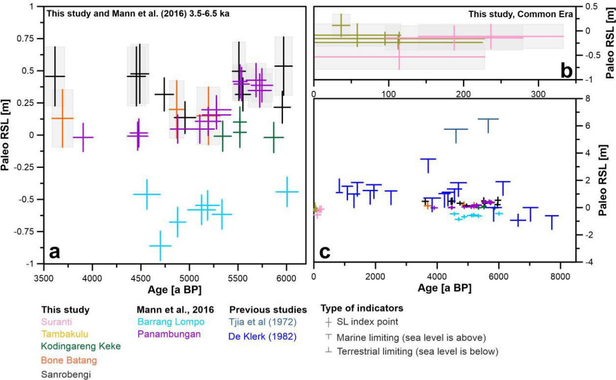
Figure 3: Representation of data reported in Table 2 and Table 3. a) RSL index points dating ~6.5 to ~3.5 ka and b) Common Era microatolls surveyed in this study. Gray bands in a) and b) represent the microatolls that were recognized as eroded in the field, and to which the erosion correction explained in the text has been applied. Panel c) shows the newly surveyed data in the context of previous studies.
