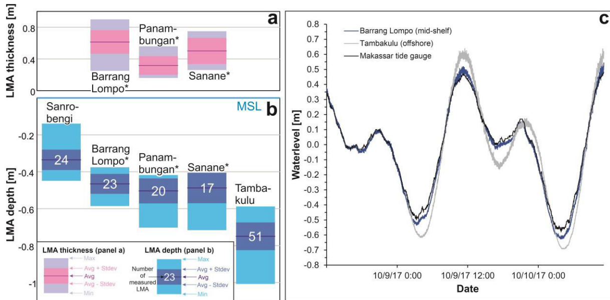
Figure 4: a) Thickness of Living Microatolls (LMA) measured by Mann et al., 2016 in the Spermonde Archipelago. The average of the three islands reported is 0.48 \pm 0.19 m. b) Measured depth of LMA in this study (Sanrobengi and Tambakulu islands) and in Mann et al., 2016. * in a) and b) indicates the islands surveyed by Mann et al., 2016. In a) and b) the islands are ordered from the closest to the shore on the left side to the further away from the shore on the right side. c) Comparison between water levels measured at Barrang Lompo (located on the mid-shelf), Tambakulu (located offshore towards the edge of the shelf) and data recorded by the national tide gauge at Makassar harbor. Note that, in a and b), 'zero' refers to mean sea level, while in b) 'zero' refers to the average water level over the measurement period (here 10/8/2017 to 10/10/2017).
