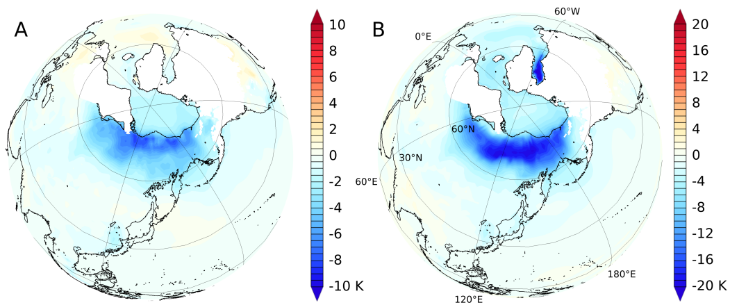
Figure 7. JJA LGM temperature anomalies showing the impact of introducing vegetation-climate feedbacks. Results are shown as LGM-PI anomalies for CAM4 (A; LGM_CAM4_Veg – LGM_CAM4_noVeg) and CAM5 (B; LGM_CAM5_Veg – LGM_CAM5_noVeg). Regions covered by continental ice sheets during the LGM have been masked out. The LGM coastlines are given in black. Note the different scaling used for the two panels.
