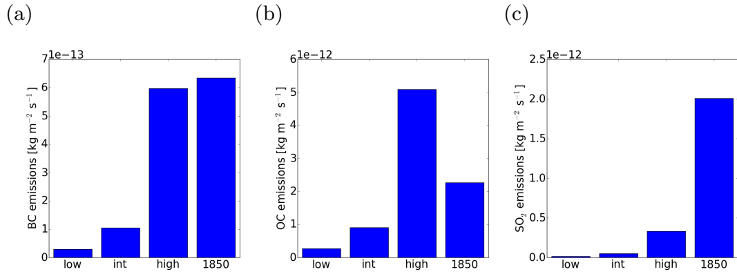
Figure 5. The annual mean anthropogenic aerosol emissions of (a) BC, (b) OC, and (c) \text{SO}_2 in AD 100 averaged over the study domain ( 10^\circ W to 50^\circ E, 20^\circ N to 60^\circ N) for the low emission scenario (low), the intermediate emission scenario (int), and the high emission scenario (high). Also shown are the anthropogenic aerosol emissions from the ACCMIP inventory for the year AD 1850 averaged over the same region.
