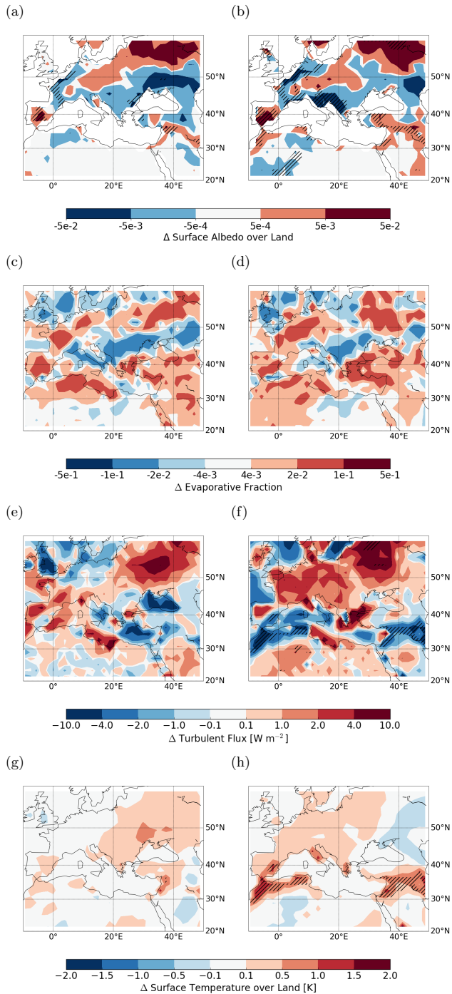
The impact of anthropogenic land-cover change on climate using HYDE11 (left) and KK11 (right). Shown are changes in surface albedo over land (a,b), evaporative fraction (c,d), turbulent flux (e,f), and land surface temperature (g,h). Statistically significant changes (5% significance level; N = 20 ) are hatched.
