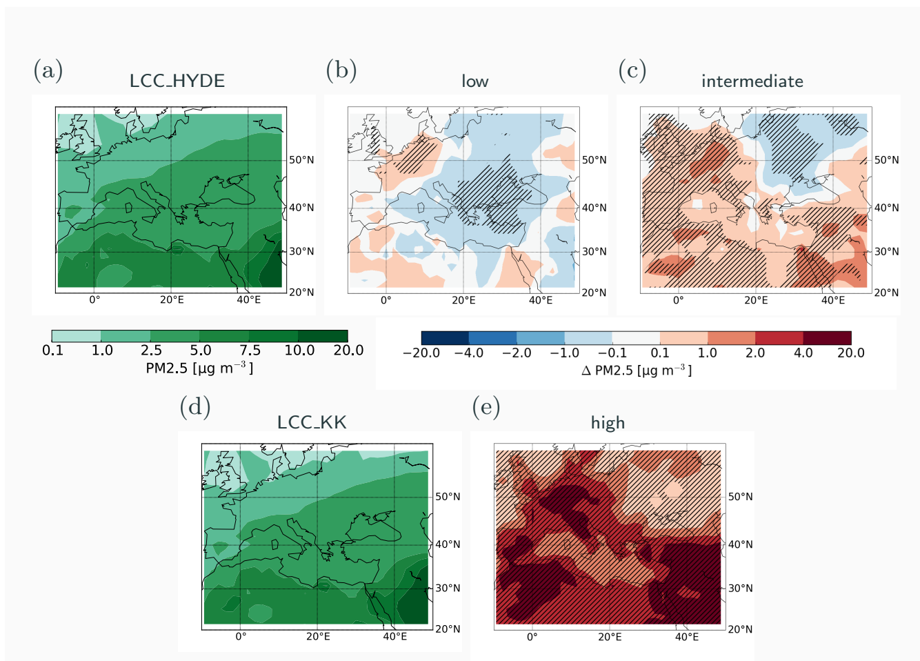
Figure 8. The background surface PM2.5 concentrations (a: LCC_HYDE; d: LCC_KK) and the changes in PM2.5 surface concentrations due to anthropogenic aerosol emissions for the low (b; LCC_HYDE_low), the intermediate (c; LCC_HYDE_int), and the high (e; LCC_KK_high) emission scenarios. Statistically significant changes (5% significance level; N = 20 ) are hatched.
