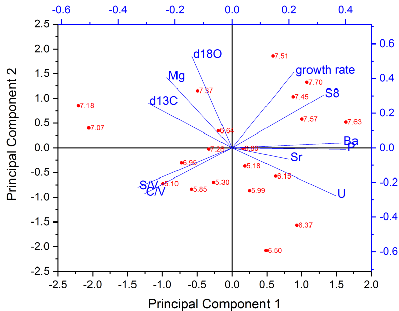
Figure 1. Principal component analysis for the middle part of the stalagmite.
