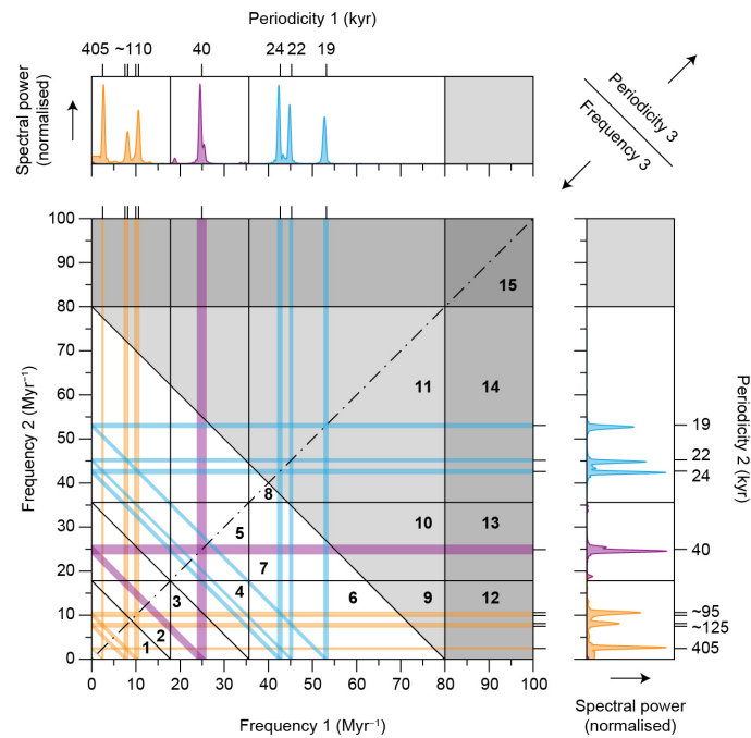
Figure 3. Bispectral zonation scheme. Bispectra of climate cycles can be subdivided into 15 zones that reflect unique combinations of three frequency bandwidths. Orange, purple, and blue lines represent the main astronomical frequencies of the eccentricity, obliquity and precession cycles, respectively (this colour coding is consistent throughout the paper). The grey shaded areas represent suborbital periodicities. Difference frequencies f_1 and f_2 are plotted along the horizontal and vertical axes, respectively. Sum frequencies f_3 (i.e., f_1 + f_2 ) are depicted as diagonal lines in the bispectrum. See also Table A1 for a list of bispectral zones, and Table A2 for a list of triad types among the main astronomical frequencies in the bispectrum.
