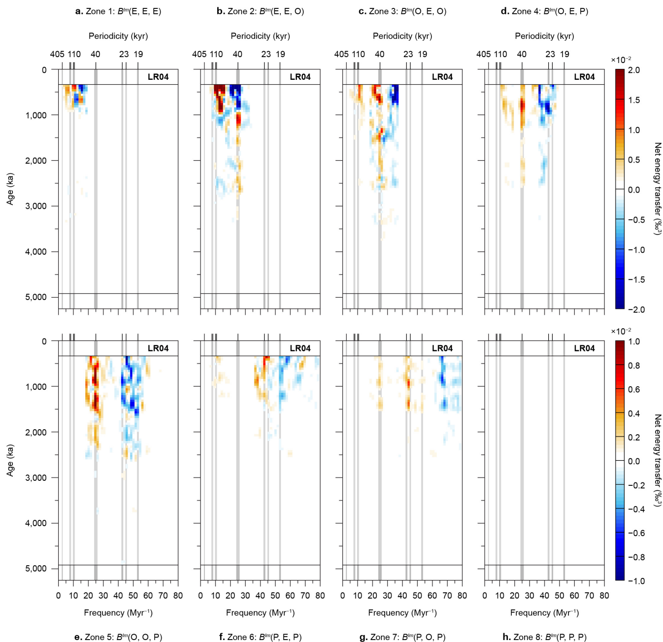
Figure 8. Disentangling “black box” climate. Conservative net energy transfers during the Pliocene and Pleistocene over specific zones in the imaginary part of the bispectrum (see Methods). Computational settings as in Figure 5b. (a) Zone 1. (b) Zone 2. (c) Zone 3. (d) Zone 4. (e) Zone 5. (f) Zone 6. (g) Zone 7. (h) Zone 8. See also Figure 3 and Table A1.
