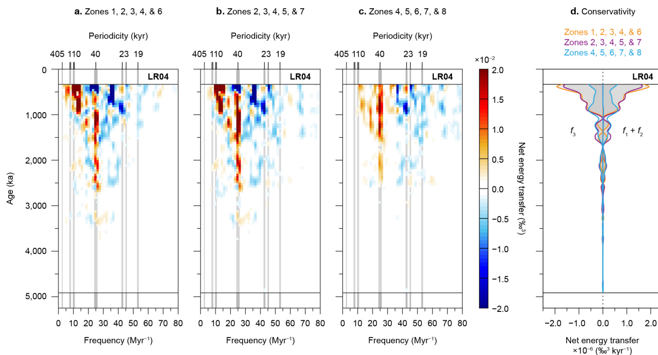
Figure 10. Summed zonal integrations of the imaginary part of Pliocene and Pleistocene bispectra. Net energy transfers are computed by (a) summing Zones 1, 2, 3, 4, and 6 for triad interactions corresponding to the “eccentricity” bandwidth, (b) summing Zones 2, 3, 4, 5, and 7 for triad interactions corresponding to the “obliquity” bandwidth, and (c) summing Zones 4, 5, 6, 7, and 8 for triad interactions corresponding to the “precession” bandwidth. Panel (d) shows the corresponding summed zonal conservativities with eccentricity in orange, obliquity in purple, and precession in blue.
