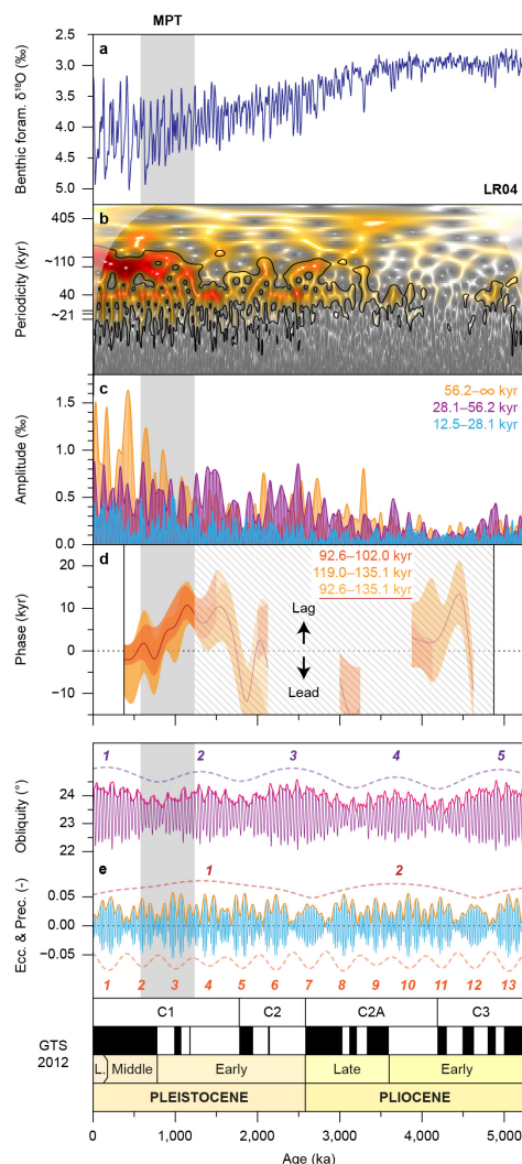
Figure 1. Sinusoidal properties of Pliocene and Pleistocene climate cycles (after (Lisiecki and Raymo, 2005; Lisiecki, 2010)). (a) Resampled LR04 benthic foraminiferal \delta^{18}\text{O} stack. (b) Wavelet analysis of the LR04 stack after detrending. (c) Absolute amplitude modulations and filters of the \sim 110 -kyr, 40 kyr, and \sim 21 -kyr cycles. (d) Phase evolution of the \sim 110 -kyr cycles with respect to eccentricity (Laskar et al., 2011a; Laskar et al., 2011b), computed over a 750 kyr sliding window. Blackman-Tukey phase estimates are only shown when coherent (Paillard et al., 1996). We focus the phase interpretation on the time interval with high amplitude \sim 110 -kyr cycles (transparent area). Phase relationship of \delta^{18}\text{O} to obliquity is not shown because it is assumed during the astronomical tuning process. Phase to precession is not shown because globally averaged \delta^{18}\text{O} records have no single response to either NH or SH precession forcing. (e) Obliquity, eccentricity and precession solutions. The 1.2-Myr obliquity, and 2.4-Myr and 405-kyr eccentricity cycles numbers are given. Black and white bars correspond to normal and reversed magnetochrons of the 2012 geologic time scale (Hilgen et al., 2012).
