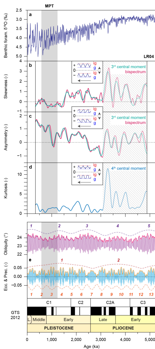
Figure 2. Nonsinusoidal properties of Pliocene and Pleistocene climate cycles (after (Lisiecki and Raymo, 2007)). (a) As in Figure 1. (b) Evolution of glacial-interglacial cycle skewness, (c) asymmetry, and (d) kurtosis (i.e., normalised third and fourth central moments). Computed over a 668 kyr sliding window, using standard (teal and blue lines) and bispectral (pink lines) methods. Cycle kurtosis is computed with the standard method only, because no trispectra were computed. Inset boxes show corresponding cycle shapes. The arrow shows the direction of time, g = glacial, ig = interglacial. We focus the geometry interpretation on the time interval with the greater amplitude variability in the record (transparent area). (e) As in Figure 1.
