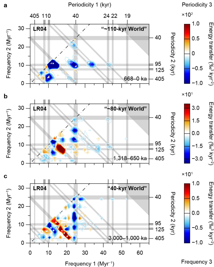
Figure 4. Bispectra of Pliocene and Pleistocene climate cycles. (a) Imaginary part of a bispectrum of the Middle and Late Pleistocene “~110-kyr world”. Age range = 668 ka to 0 ka. Resampling resolution = 1 kyr -1 . Window length = 668 kyr. Block length = 668 kyr. Number of blocks = 1. Number of merged frequencies = 1. Frequency resolution = 1.50 Myr -1 . Degrees of freedom = 2. Min value = -598 ‰ 3 kyr -2 . Max value = 51 ‰ 3 kyr -2 . (b) Imaginary part of a bispectrum of the mid-Pleistocene transition “~80-kyr world”. Age range = 1,318 ka to 650 ka. Resampling resolution = 1 kyr -1 . Window length = 668 kyr. Block length = 668 kyr. Number of blocks = 1. Number of merged frequencies = 1. Frequency resolution = 1.50 Myr -1 . Degrees of freedom = 2. Min value = -57 ‰ 3 kyr -2 . Max value = 73 ‰ 3 kyr -2 . (c) Imaginary part of a bispectrum of the Pliocene and Early Pleistocene “40-kyr world”. Age range = 3,000 ka to 1,000 ka. Resampling resolution = 1 kyr -1 . Window length = 2,000 kyr. Block length = 2,000 kyr. Number of blocks = 1. Number of merged frequencies = 3. Frequency resolution = 1.50 Myr -1 . Degrees of freedom = 6. Min value = -21 ‰ 3 kyr -2 . Max value = 23 ‰ 3 kyr -2 . Note the different scaling of the z-axes between panel (a), (b), and (c). These bispectra are computed on the LR04 stack (see Methods) (Lisiecki and Raymo, 2005).
