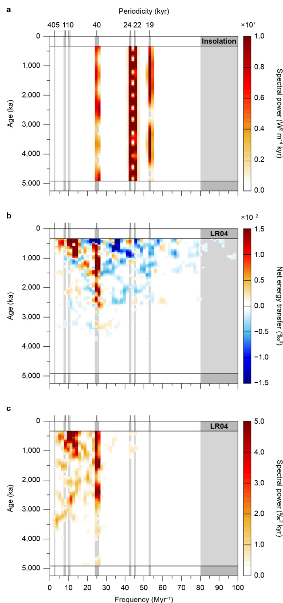
Figure 5. Input → “black box” climate → output. (a) Power spectral density of mean summer insolation (June 21 to September 21) at 65°N (Paillard et al., 1996; Laskar et al., 2004). (b) Conservative net energy transfers during the Pliocene and Pleistocene, computed by integrating over the entire imaginary part of the bispectrum (see Methods). Input data is the resampled LR04 stack (Lisiecki and Raymo, 2005). (c) Power spectral density of the LR04 stack (Lisiecki and Raymo, 2005). For all three panels, the window length is 668 data points (668 kyr), and the step-size between partially overlapping windows is 50 data points (50 kyr). We used no blocks and did not merge frequencies. These settings yield a frequency resolution of 1.50 Myr -1 , and 2 degrees of freedom.
