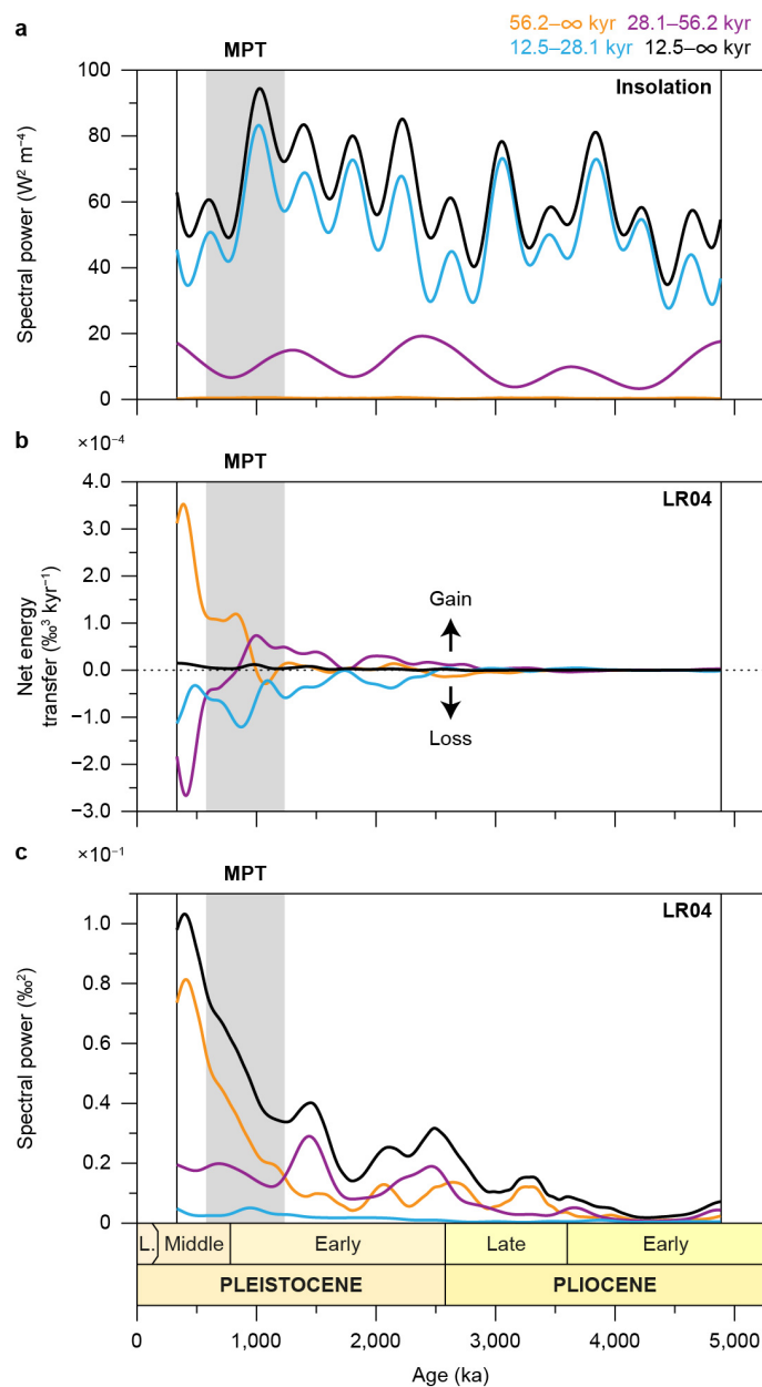
Figure 7. Integration of the spectra and bispectra per astronomical bandwidth (top right). (a) Totally and zonally integrated spectra of mean summer insolation (June 21 to September 21) at 65^\circ N . (b) Totally and zonally integrated bispectra of the LR04 stack. (c) Totally and zonally integrated spectra of the LR04 stack. Computational settings as in Figure 5.
