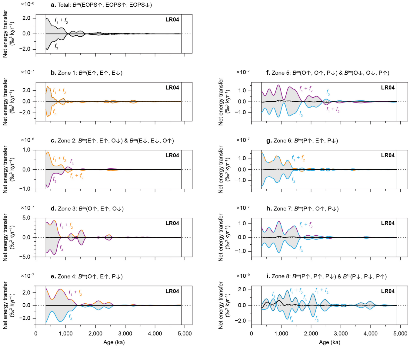
Figure 9. Conservativity of energy in triad interactions located in the imaginary part of Pliocene and Pleistocene bispectra. Conservativity of (a) the entire bispectrum (Fig. 5b), and (b) Zone 1, (c) Zone 2, (d) Zone 3, (e) Zone 4, (f) Zone 5, (g) Zone 6, (h) Zone 7, and (i) Zone 8, of the bispectrum (Fig. 8). Energy gains or losses of f_1 and f_2 (dashed lines) are computed using Eq. 8, those of f_3 (single coloured lines) following Eq. 7, and their difference (black lines) by Eq. 6.
