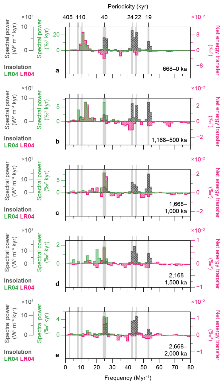
Figure 6. Qualitative linkage of power spectra of insolation to those of climate, via energy exchanges among climate cycles. (a) 334 ka. (b) 834 ka. (c) 1334 ka. (d) 1834 ka. (e) 2334 ka. Computational settings as in Figure 5. Note that the scaling between the spectra and energy exchanges is arbitrary. Energy exchanges of the LR04 stack can be scaled to the power spectrum of the LR04 by using multiplication factors of 430, 250, 360, 230, and 250 for panels (a) to (e), respectively.
