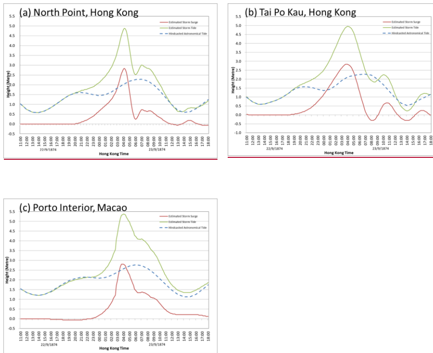
Figure 7. Time series of the hindcasted astronomical tide and estimated storm tide above Hong Kong Chart Datum and the estimated storm surge at (a) North Point and (b) Tai Po Kau in Hong Kong, and the hindcasted astronomical tide and estimated storm tide above Macao Chart Datum and the estimated storm surge at (c) Porto Interior in Macao from 11 a.m. on 22 September to 6 p.m. on 23 September 1874. The estimated storm tide is the sum of the estimated storm surge and the astronomical tide.
