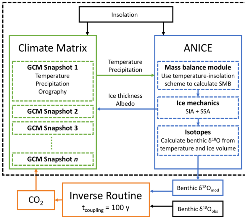
15 Figure 3: A conceptual visualisation of the inverse forward modelling approach. The model is forced externally by a benthic δ 18 O record and an insolation reconstruction (black boxes). The inverse routine calculates pCO 2 based on the difference between observed and modelled δ 18 O. This value is forwarded to the climate matrix, which interpolates between the GCM snapshots based on the prescribed pCO 2 value and the modelled state of the cryosphere (ice thickness and albedo).
