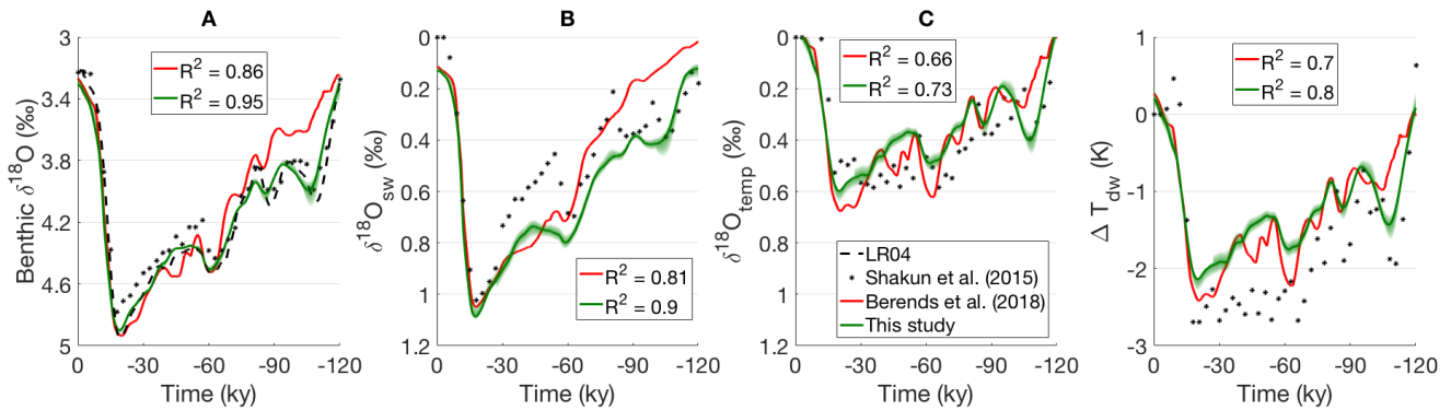
15 Figure 6: Benthic δ 18 O for the LGC simulation using the inverse-method forced matrix model, compared to data from LR04 (A; Lisiecki and Raymo, 2005) and from Shakun et al. (2015) for both the contribution from the δ 18 O of seawater (B) and that from deep water temperature (C), as well as the resulting deep water temperature itself (D). Also shown are the results from Berends et al. (2018). Solid green line shows the benchmark run, green shaded area shows the maximum uncertainty range from the sensitivity experiment. Since the new model set-up is forced with the LR04 stack, rather than with the EPICA CO 2 record used by Berends et al. (2018), the increased correlation coefficients are not a strong result. 20
