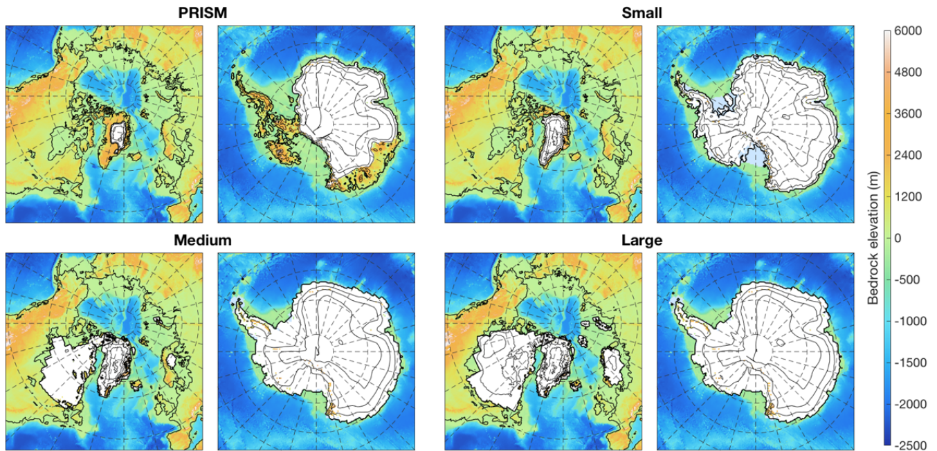
Figure 2: The four ice-sheet configurations used by Dolan et al. (2015) as boundary conditions for their HadCM3 simulations. “PRISM” is the PRISM3 ice sheet from Dowsett et al. (2010), “Small” is present day, “Medium” is the ICE-5G reconstruction (Peltier, 2004) at 8 ky ago and “Large” is ICE-5G at 11 ky ago.
