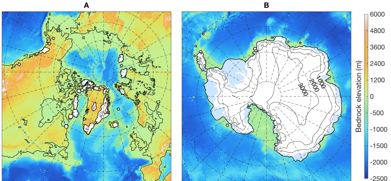
Figure 11: The ice-sheets during KM5c (3.205 My ago), as simulated with the inverse-method forced matrix model. Contour lines for the Northern Hemisphere (A) show ice thickness, contour lines for Antarctica (B) show surface elevation. Antarctic ice shelves
