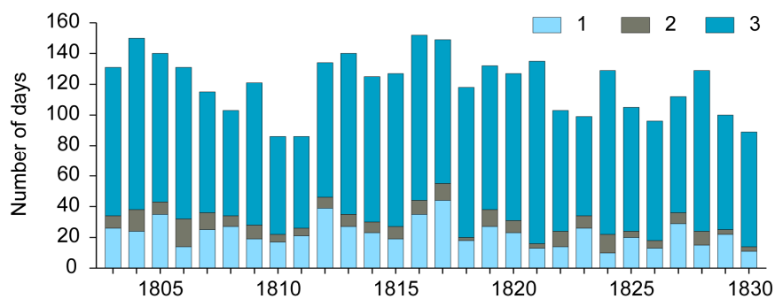
Figure 5. Fluctuations in the annual number of precipitation days (1 – solid, 2 – mixed, 3 – liquid) at Buchlovce during 1803–1830 derived from the weather diary kept by Šimon Hausner.
