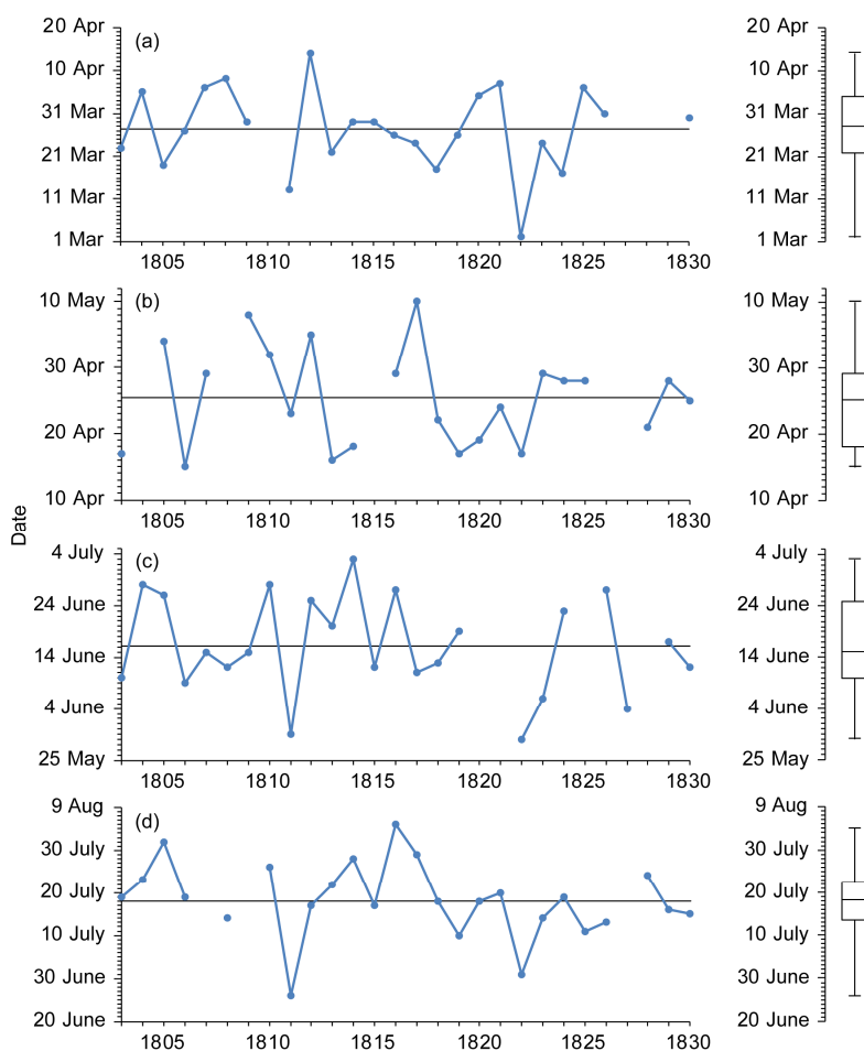
Figure 8. Fluctuations (left) and box-plots (right) of the beginnings of selected phenophases and agricultural work at Buchlovice during 1803–1830 derived from the weather diary kept by Šimon Hausner: (a) spring sowing of cereals; (b) blossoming of cherry trees; (c) blossoming of grapevine; (d) grain harvest.
