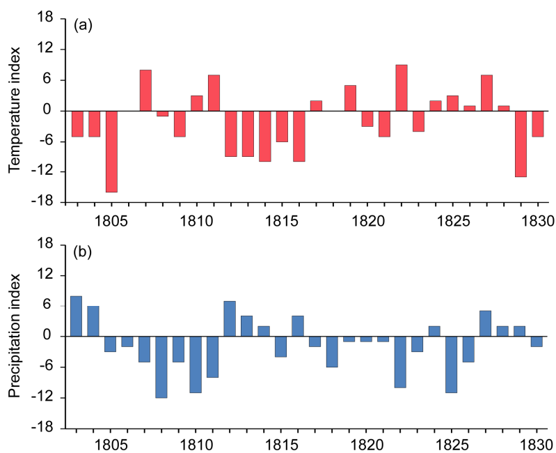
Figure 4. Fluctuations in annual temperature (a) and precipitation (b) indices at Buchlovice during 1803–1830, as derived from the weather diary kept by Šimon Hausner.
