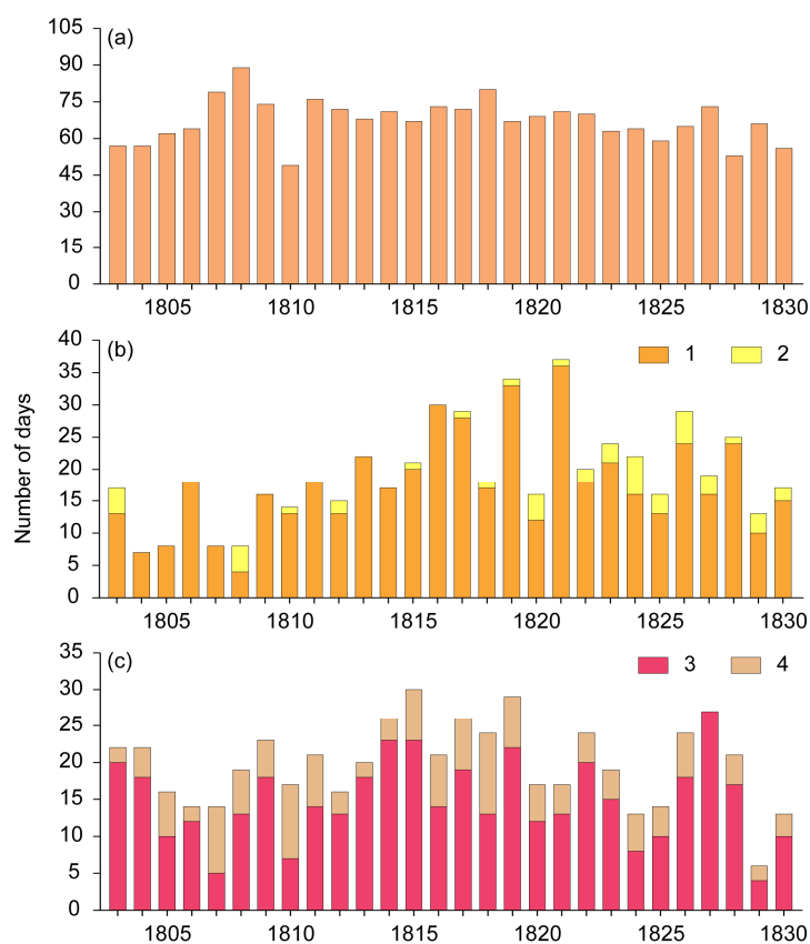
Figure 7. Fluctuations in the annual number of days with selected phenomena at Buchlovice during 1803–1830 derived from the weather diary kept by Šimon Hausner: (a) strong wind; (b) fog (1 – fog, 2 – foggy); (c) thunderstorm (3 – at Buchlovice, 4 – distant thunderstorm).
