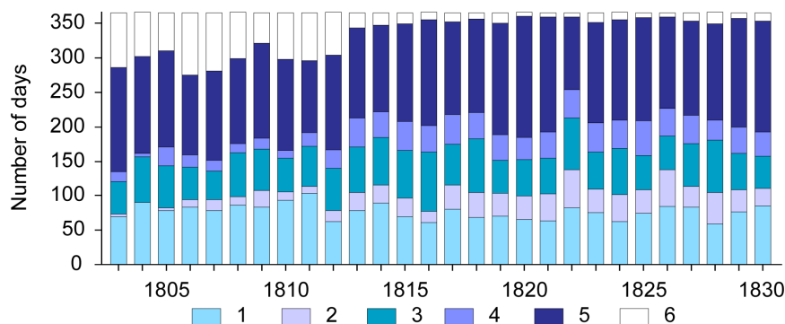
Figure 6. Fluctuations in annual cloudiness at Buchlovice during 1803–1830, derived from the weather diary kept by Šimon Hausner: 1) clear sky, 2) clear sky in one part of the day and half-covered sky in the other part, 3) half-covered sky, 4) half-covered sky in one part of the day and overcast in the other part, 5) overcast, 6) missing days or no information related to cloudiness.
