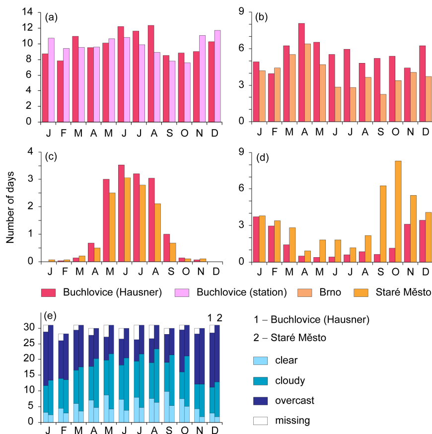
Figure 13. Comparison of annual variation of selected climatological characteristics at Buchlovice interpreted from Hausner's records for 1803–1830 and at three selected meteorological stations in 1961–1990: (a) number of precipitation days (with totals \geq 0.1 mm for the Buchlovice rain-gauge station); (b) number of days with strong winds (with wind force \geq 7^\circ\text{B} , i.e. wind speed \geq 10.8 m s ^{-1} for Brno); (c) number of days with thunderstorm; (d) number of days with fog; (e) number of days with various degrees of cloudiness: clear days (0–2/10 of cloud cover at Staré Město), cloudy days (2.1–7.9/10 of cloud cover at Staré Město, sum of categories 2, 3 and 4 at Buchlovice – see Fig. 6) and overcast days (8–10/10 of cloud cover at Staré Město).
