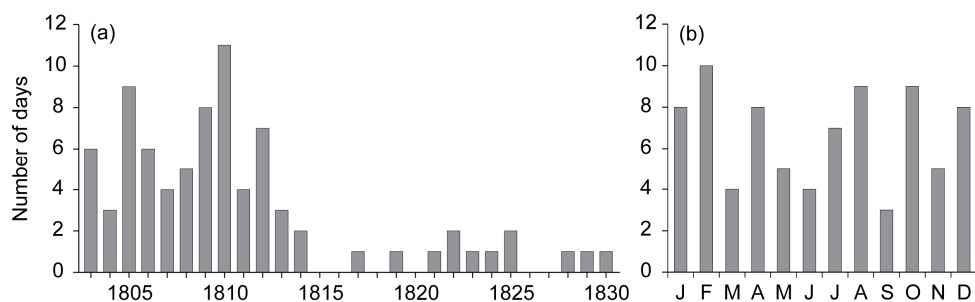
Figure 3. Days missing from daily weather records kept by Šimon Hausner at Buchlovice during 1803–1830 (a) and their annual variation (b).
