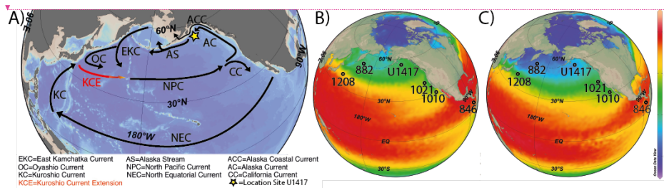
Figure 1: Map of modern ocean circulation and SSTs. a) Modern North Pacific Ocean circulation, b) September c) and December 1955-2013 SST average centred in the North Pacific Ocean (NOAA WOA13, Locamini et al. , 2013) and core sites discussed in this study. Map made using Ocean Data View (Schlitzer, 2018).
