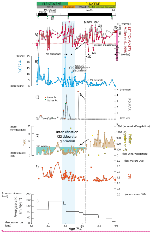
Figure 2: Site U1417 across the Pliocene-Pleistocene transition. a) red line: SST from U^{k_{37}} index according to Müller et al. (1998) calibration; grey line: SST from U^{k_{37}} index according to Prah et al. (1988) calibration. Black squares are samples where alkenones were not detected. Dashed red line: Modern averaged decades (1955-2012) annual statistical mean SST=6.4 °C at 0 m water depth (NOAA WOD13, Boyer et al. , 2013) at Site U1417, similar to the modern annual average SST=7 °C at GAK1 station during the 1970-2018 time intervals for the 0-100 m water column depth (Weingartner et al. 2016) in the Gulf of Alaska; Red star on y-axis: value of our youngest sample analysed at Site U1417 (U1417D 1H-1W 44-48; 0.016 Ma; SST=10.6 °C with Müller et al. (1998) calibration; SST=11.8 °C with Prah et al. , 1988 calibration); Pink rectangle on y axis: modern averaged decades (1955-2012) statistical mean SST during winter and summer at Site U1417 and 0 m water depth (NOAA WOD13, Boyer et al. , 2013) SST=0-11.3 °C; b) abundance of the cold and freshwater
