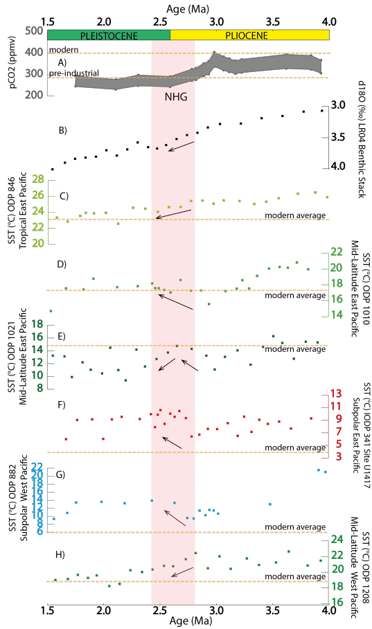
Figure 3: Pliocene-Pleistocene SST across the North Pacific. a) Alkenone \text{pCO}_2 upper and lower end (ppmv) estimates at Site ODP 999A (Seki et al. , 2010); b) \delta^{18}\text{O} (‰) LR04 Benthic Stack (Lisiecki and Raymo, 2005); Alkenone SST ( ^{\circ}\text{C} ) from c) ODP Site 846 (Herbert et al. , 2017), d) Site 1010 (Herbert et al. , 2018), e) Site 1021 (Herbert et al. , 2018), f) IODP 341 Exp. Site U1417 (Sánchez-Montes et al. , 2019), g) ODP Site 882 (Martínez-García et al. , 2010) and h) ODP Site 1208 (Herbert et al. , 2018). Orange horizontal lines indicate reference levels of pre-industrial times and/or modern values for each of the records or sites (SSTs from NOAA WOD13, Boyer et al. , 2013). Arrows indicate position of M2 and KM2 periods and cooling or warming trends across the Pacific Ocean. The KM2 event is located within the MPWP. The MG1-G1 warming precedes the M2 event. b) to h) climate data are 100 kyr smoothed records, and the x axis have been determined through the calculation of the mean for each interval.
