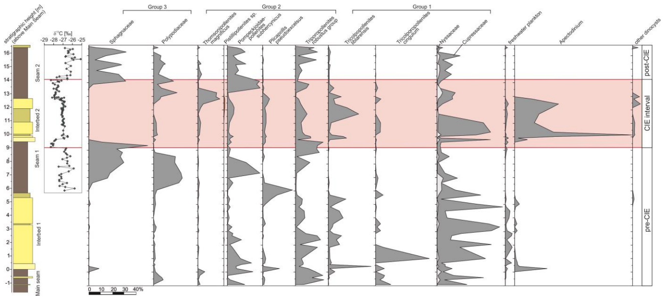
Figure 5: Simplified pollen diagram, comprising the top of the Main Seam up to the top of Seam 2, showing frequency and palynological abundance changes between pre-, peak- and post-CIE intervals. The carbon isotope data is shown for comparison. Due to the different thicknesses of the sections (cf. Fig. 2), it has been tied to top and base of Seam 1 and top and base of Seam 2. Red bar indicate the carbon isotope excursion. The palynological record is characterized by three palynological groups: (1) elements with frequency maxima in the clastic interbeds (representing the hinterland), (2) interbed-lignite seam transitional elements and back mangrove equivalents, and (3) elements dominating the lignite seams.
