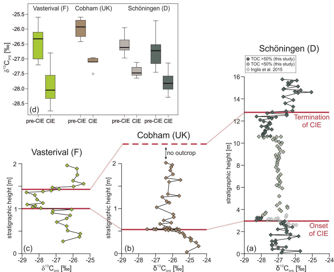
Figure 3: Comparison of mid-latitude wetland \delta^{13}C_{TOC} records surrounding the paleo-North Sea (cf. Fig. 1): (a) Schöningen, Germany (this study (green symbols), Inglis et al. (2015) (grey symbols)), (b) Cobham, UK (Collinson et al., 2003), (c) Vasterival, France (Storme et al., 2012). Note the different stratigraphic thicknesses due to different sediment accumulation and preservation conditions in the individual depositional environments. (d) Carbon isotopic differences at the onset of the CIE.
