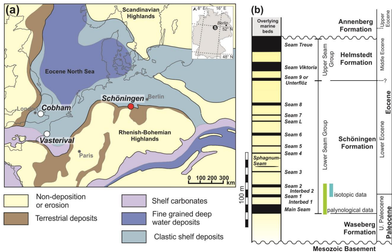
Figure 1: (a) Palaeogeographic map of northwestern Europe during the early Eocene (adapted from Ziegler, 1990) showing the locations of the Schöningen open cast mine (D), Cobham (UK) and Vasterival (F). (b) Schematic stratigraphy of the Schöningen area (adapted from Brandes et al., 2012).
