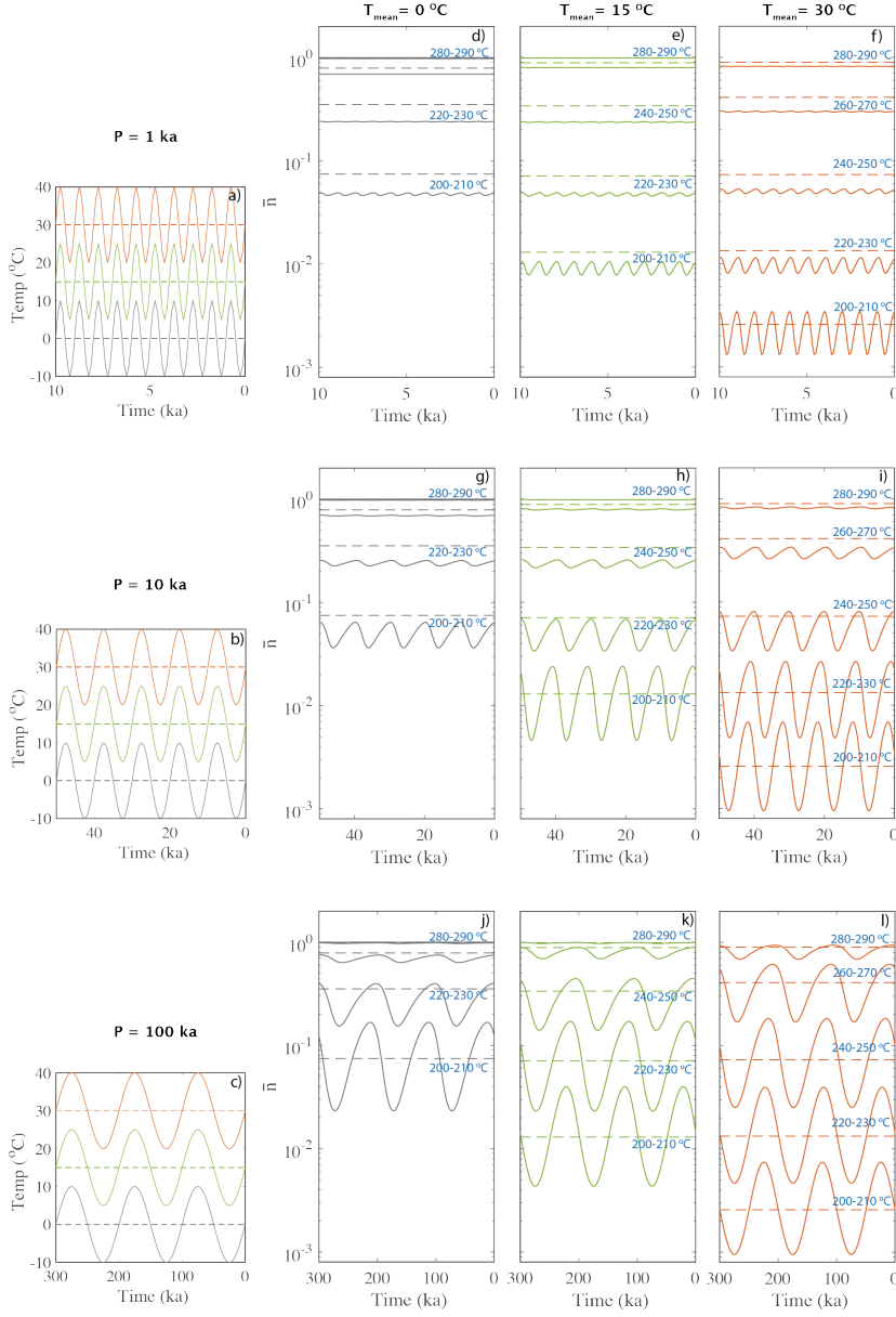
Figure 4: Variation of trapped charge population ( \bar{n} ) for different sinusoidal thermal histories. a, b, and c represents the prescribed thermal histories with same mean amplitude (10 °C) and three different mean temperatures (0, 15 and 30 °C) but for different periods, 1, 10 and 100 ka respectively. The dashed lines are the isotherm (mean temperature of oscillation). Fig. d-f, g-i, and j-l are the the response of \bar{n} for the corresponding thermal field. The solid lines are for oscillating fields and dashed lines are for isothermal fields. The temperature of the representative thermometers (or TL temperature) are shown inside in blue.
