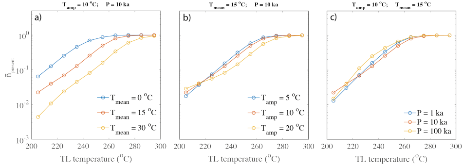
Figure 5: Present day trapped charge populations ( \bar{n}_{present} ) of different TL signals (or thermometers) with a) mean temperature variation (amplitude and period are fixed), b) amplitude variation (mean temperature and period are fixed), and c) period variation (mean temperature and amplitudes are fixed).
