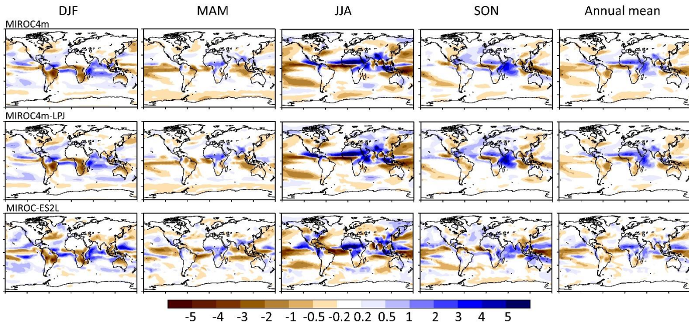
595 Figure 9: Annual and seasonal precipitation change is shown as the 127ka-PI (mm/day).
