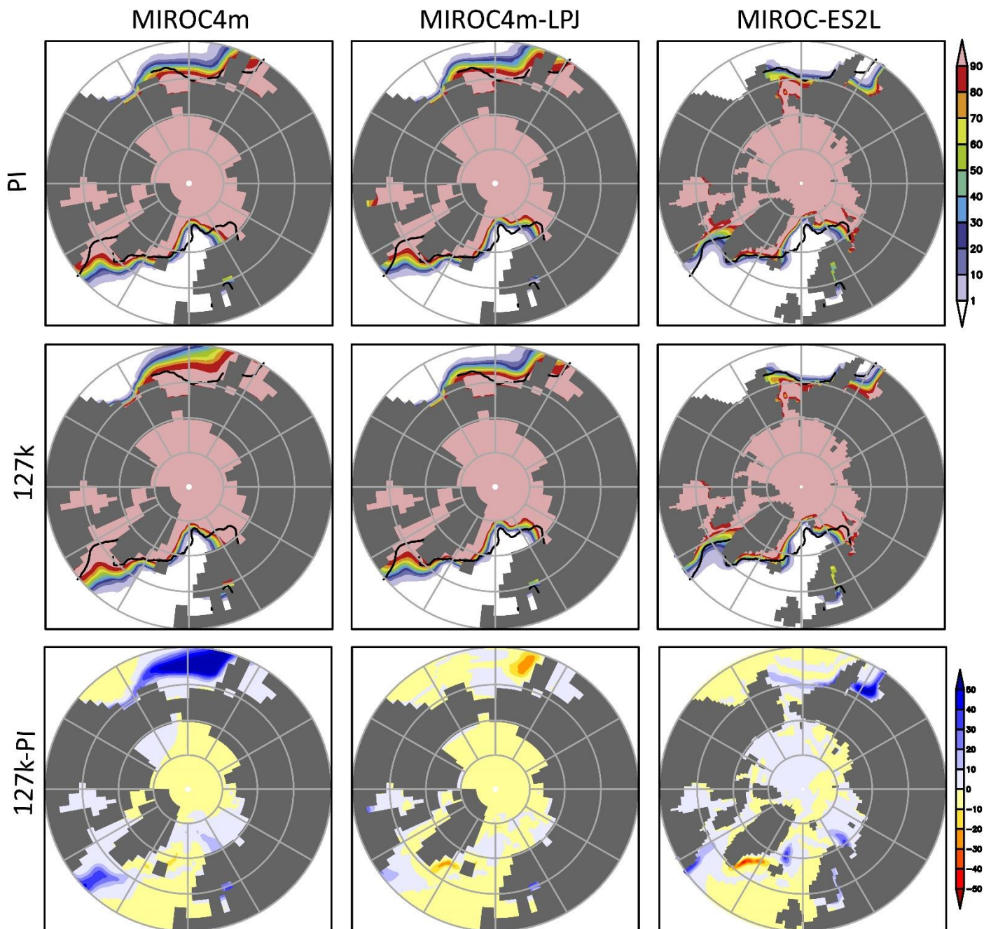
600 Figure 10: NH March sea ice concentration (%) in PI, 127k and difference between 127k and PI are shown for three models. Thick lines indicate a concentration of 15% in the climatology (the HadISST data averaged over 1961–1990).
