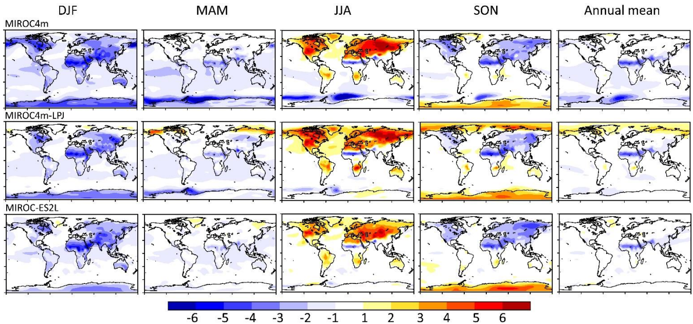
575 Figure 4: Seasonal and annual surface air temperature difference (K) between 127k and PI in three models. The present-day calendar is applied to both PI and 127k.
