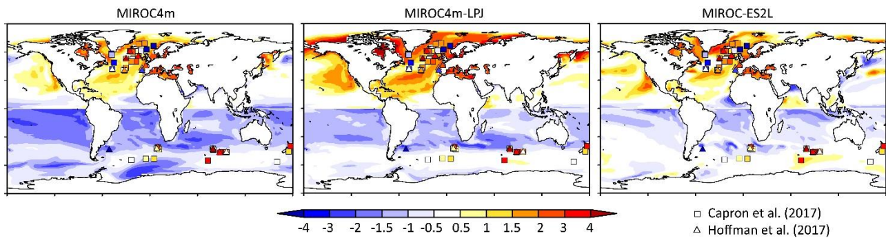
Figure 8: Summer (JJA in NH, DJF in SH) sea surface temperature change (K) in 127k from PI is compared with reconstruction by Capron et al. (2017) and Hoffman et al. (2017).
