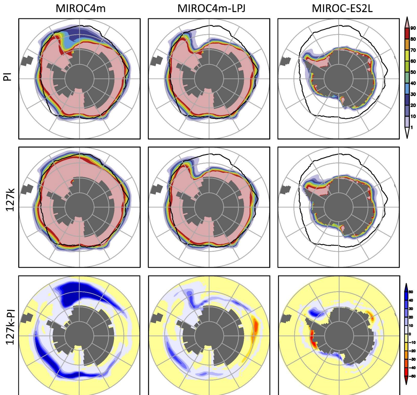
Figure 13: As same as Figure 10 but SH September sea ice concentration (%).
