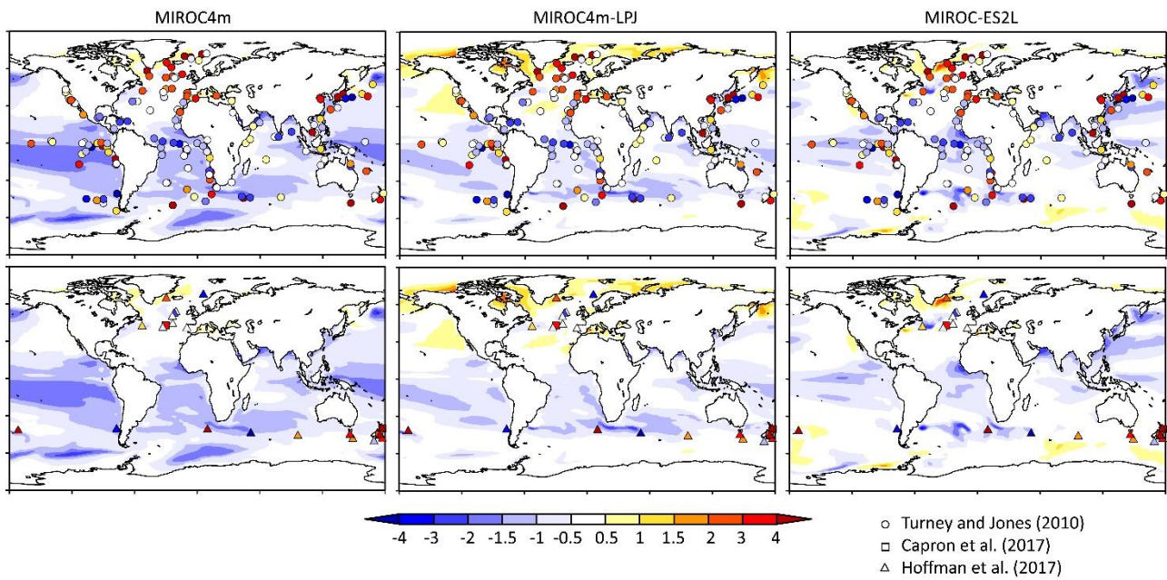
Figure 7: Annual sea surface temperature change (K) in 127ka from PI is compared with reconstruction by Turney and Jones (2010), Capron et al. (2017) and Hoffman et al. (2017).
