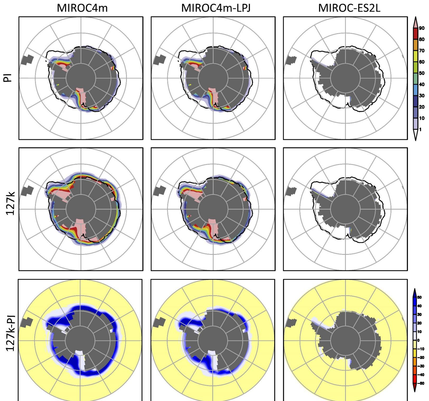
Figure 12: As same as Figure 10 but SH March sea ice concentration (%).
