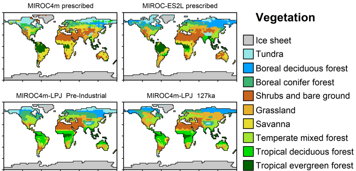
570 Figure 3: Vegetation distribution as fixed boundary condition (MIROC4m and MIROC-ES2L) and resultant most dominant vegetation types in MIROC4m-LPJ experiments in PI and 127k.
