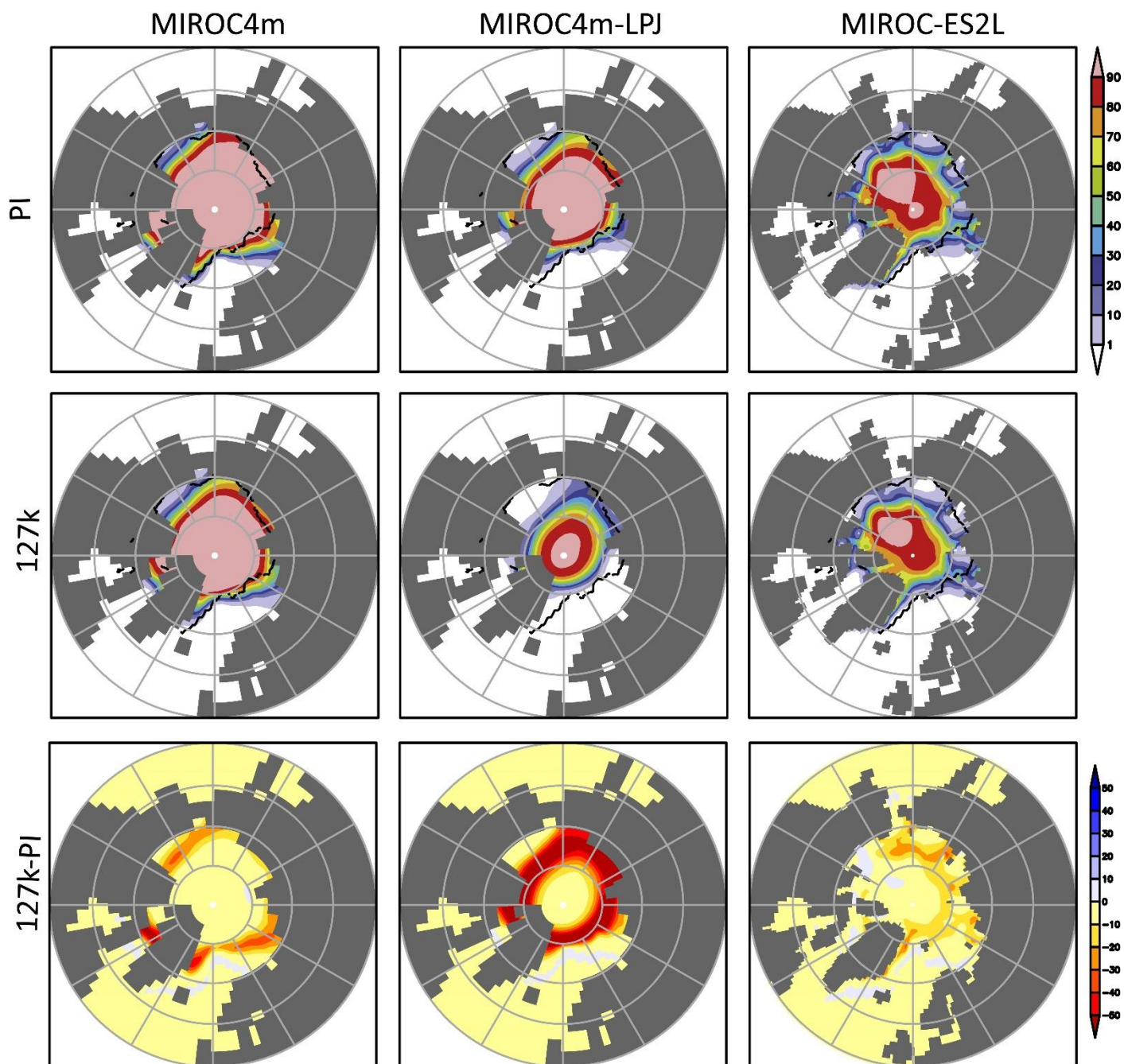
Figure 11: As same as Figure 10 but NH September sea ice concentration (%)
