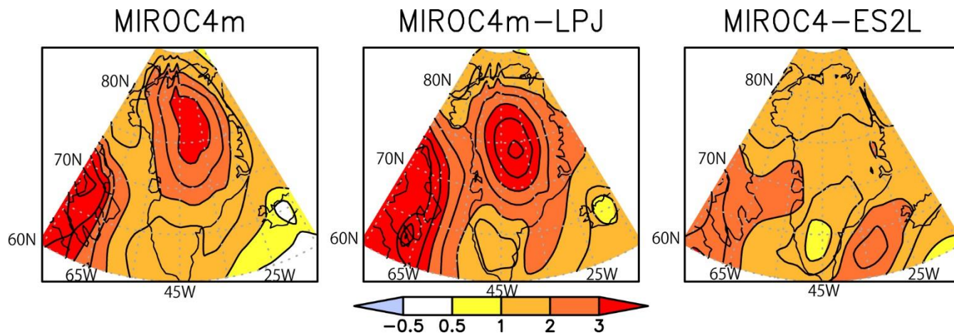
580 Figure 5: May-June-July-August averaged temperature difference (K) between 127k and PI in three models. The present-day calendar is applied to both PI and 127k.
