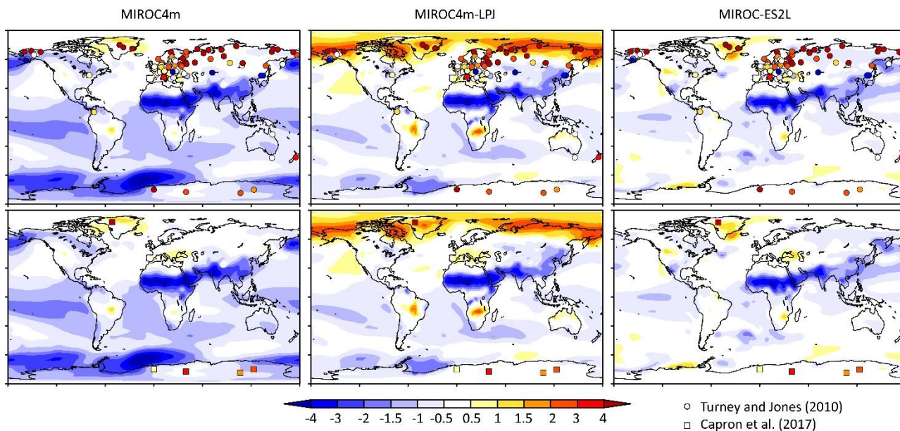
580 Figure 5: May-June-July-August averaged temperature difference (K) between 127k and PI in three models. The present-day calendar is applied to both PI and 127k.
