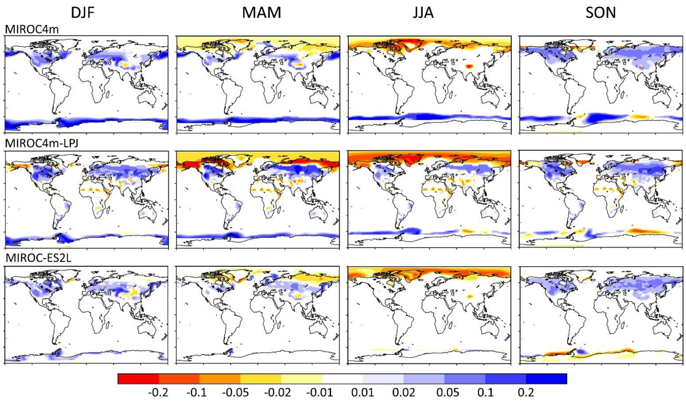
Figure 15: Seasonal surface albedo difference between 127k and PI in three models.
