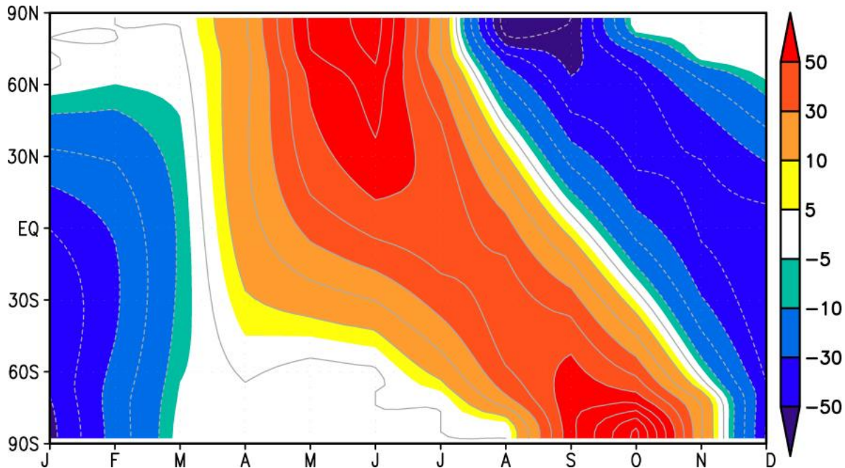
Figure 1: Latitude-month insolation anomaly between 127ka and present-day ( \text{W/m}^2 ). Modern calendar is assumed.
