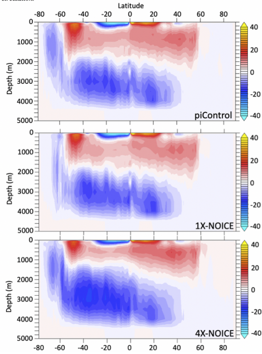
Global meridional stream function ( S_y ) for piControl, 1X-NOICE and 4X-NOICE simulations. Positive values (red) indicate a clockwise circulation and negative values (blue) an anticlockwise circulation.
