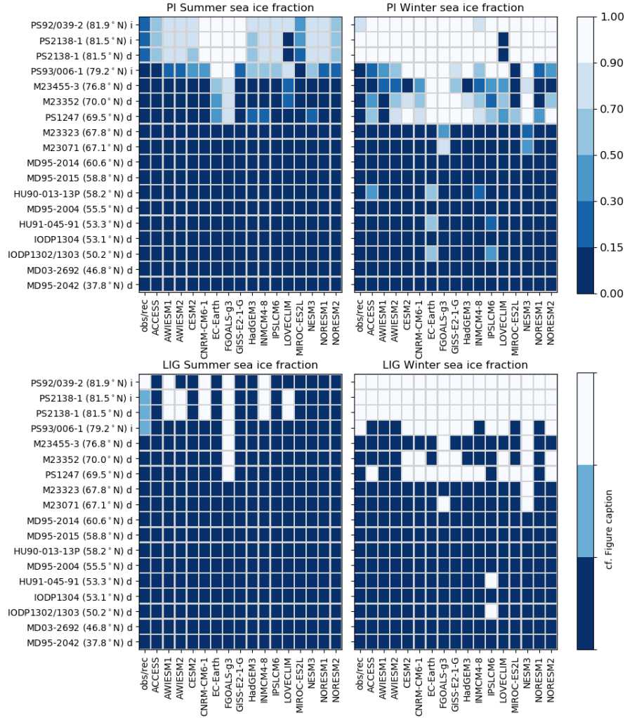
Figure 5. Model-data comparison as a function of latitude and record site for PI (top row) and LIG (bottom row). For each LIG data site, the NOAA_OI_v2 observations (PI) or reconstructions (LIG) are shown in the first column of each plot, and the model results in the columns to the right. For PI, both the model results and the data are shown in terms of sea ice fraction averaged over the month of minimum (l.h.s) or maximum (r.h.s) northern hemisphere sea ice area and the previous and following months. For the LIG, the qualitative assessments (eighth columns of Table 1 have been used, for records with good chronological control. The letter next to the name of the site stands for indicator used for the reconstruction: dinocysts ("d") or IP25/PIP25 ("i"). For summer conditions, dark blue shading is used for the "no sea ice" category, light blue shading for "summer probably ice free" conditions, and white shading for "summer sea ice concentration > 75%" and "Perennial sea ice". For winter, dark blue shading is used for "ice free all year round" conditions and white shading for "Seasonal sea-ice conditions" and "Perennial sea-ice". The model results are averaged like for PI, and shown following the colour scale to the r.h.s. of the plots.
