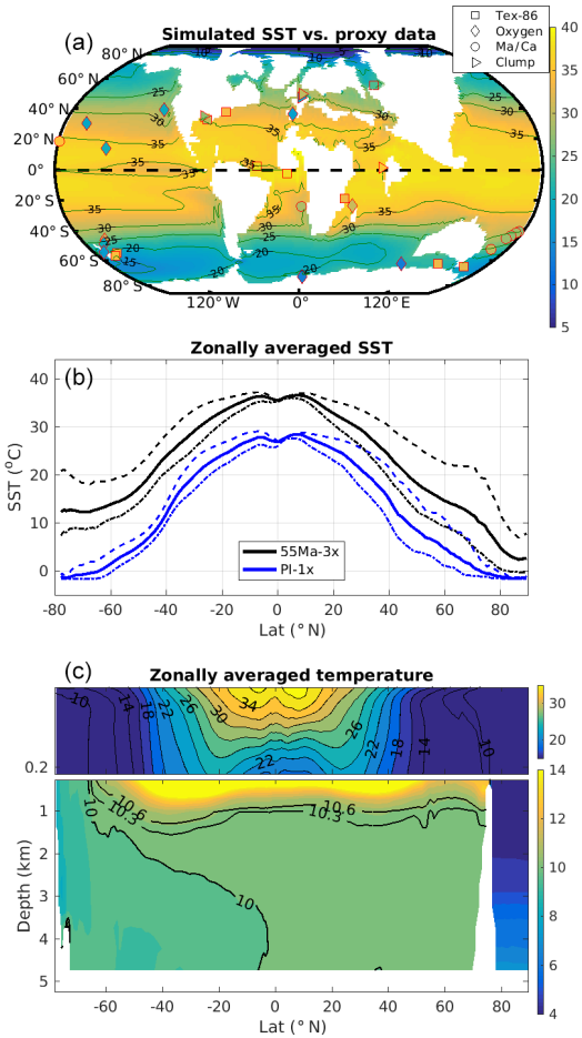
Figure 2. (a) Annual mean SST (°C) in the 55 Ma-3x simulation and point-to-point comparisons with proxy-based SST estimates from the DeepMIP dataset for the early Eocene (Hollis et al., 2019). The different symbols represent different proxies. (b) Simulated zonally averaged annual mean SST (°C, solid lines) in the 55 Ma-3x (black) and PI-1x (blue) simulations. The dashed and dotted lines indicate the means for summer and winter, respectively. (c) Zonally averaged ocean temperature in the 55 Ma-3x simulation, with a zoom of the upper 200 m (contour interval: 2 and 0.3 °C for the upper and lower parts of panel c, respectively).
