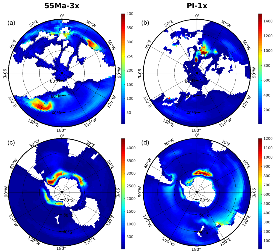
Figure 4. Winter (i.e., March in the Northern Hemisphere – a , b ; and September in the Southern Hemisphere – c , d ) mixed layer depth (m) in the 55 Ma-3x ( a , c ) and PI-1x ( b , d ) simulations. Note the very different color bars among plots. Mixed layer depth is defined by the potential density difference of 0.3 \text{ kg m}^{-3} with reference to the surface.
