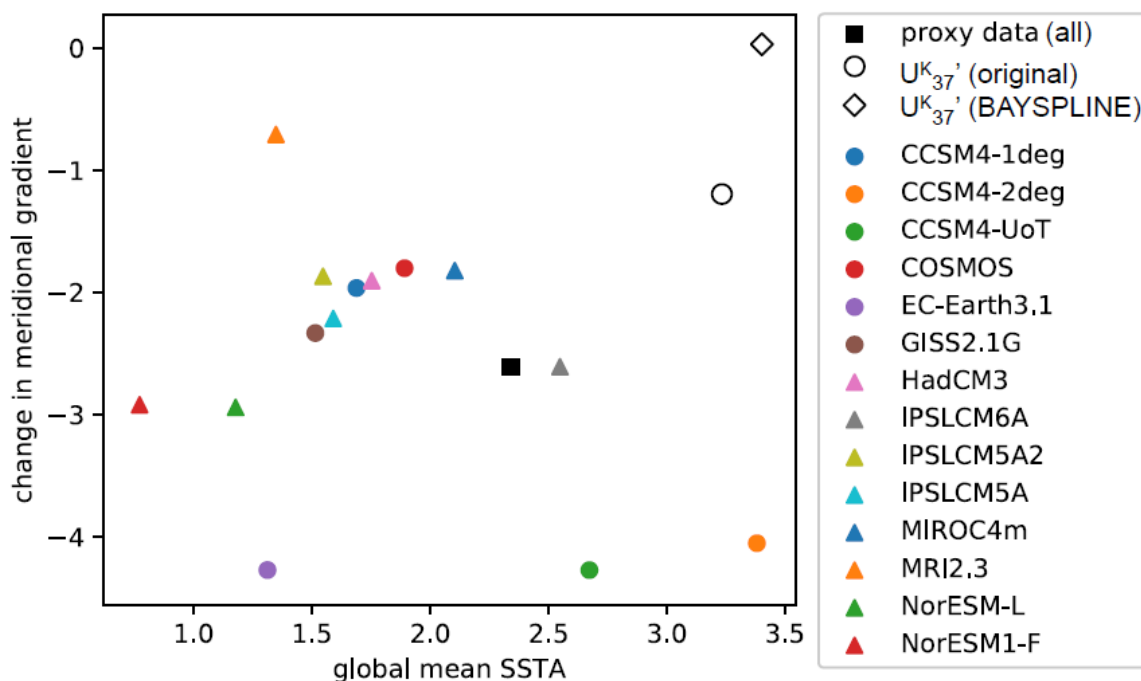
Figure 3: Comparison of KM5c SST data relative to pre-industrial (NOAA-ERSST5) for global mean SST anomalies (SSTA) and the change in meridional SST gradient, constructed using proxy data and the suite of PlioMIP2 models. The meridional SST gradient is calculated as 30°S-30°N minus 60°N-75°N, so that a more negative change in the gradient reflects a larger warming anomaly at high latitudes relative to low latitudes. Proxy data calculations were made using either all proxy data (UK 37' and Mg/Ca using their original calibrations), or using only UK 37' data. No Mg/Ca data is available >60°N so we were unable to calculate Mg/Ca-only gradients (Figure 3). The impact of changing the low- and high-latitude bands is explored in Table 1.
