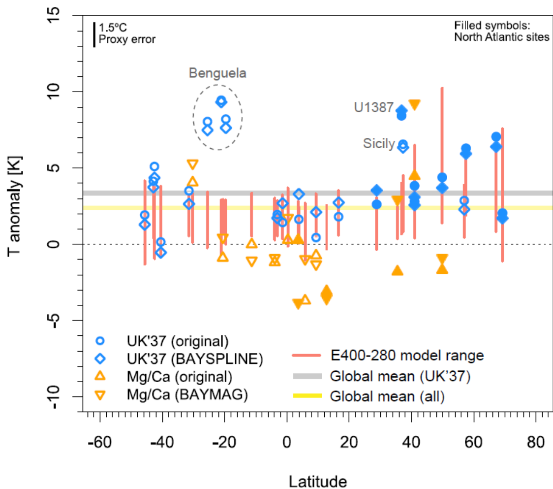
725 Figure 4: reconstructed and modelled SST anomalies plotted by latitude. SST reconstructions using the original published data and two Bayesian approaches (BAYSPLINE, BAYMAG) are shown. Vertical red lines show the range of modelled annual SSTs from all PlioMIP2 experiments (Haywood et al., submitted) calculated at the grid boxes containing each site.
