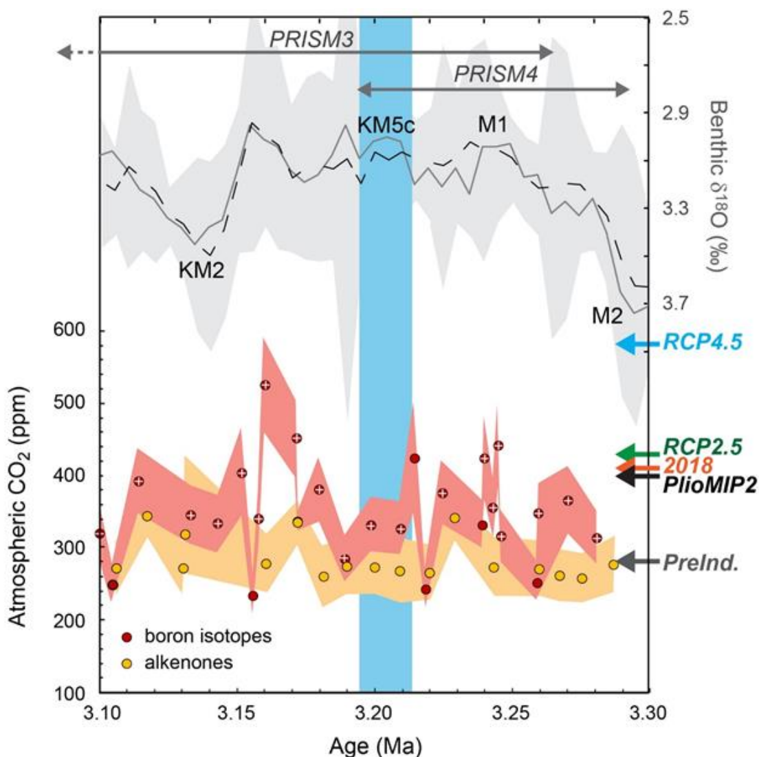
695 Figure 1: the KM5c interglacial during the late Pliocene (3.195-3.215 Ma). Upper panel: benthic oxygen isotope stack (solid line: LR04 (Lisiecki and Raymo, 2005); dashed line and grey shading: Prob-stack mean and 95% confidence interval, respectively, (Ahn et al., 2017)). Selected Marine Isotope Stages (KM2 through M2) are highlighted. The KM5c interval of focus here is indicated by the shaded blue bar. Previous Pliocene synthesis intervals are also shown: PRISM3 (3.025–3.264 Ma) and PRISM4 (isotope stages KM5c-M2; (Dowsett et al., 2016)); (c) reconstructed atmospheric CO 2 concentrations (Foster et al., 2017). Points show mean reported data (except white crosses: median values from Martinez-Boti et al., 2015), shading shows reported upper and lower estimates. Past and projected atmospheric CO 2 concentrations highlighted by arrows: PlioMIP2 simulations are run with CO 2 at 400 ppmv (Haywood et al., submitted) close to the annual mean in 2018 (NOAA), Pre-Industrial values from ice cores (Loulerge et al., 2008) and projected representative concentration pathways (RCP) for 2100 CE (IPCC, 2013). 700
