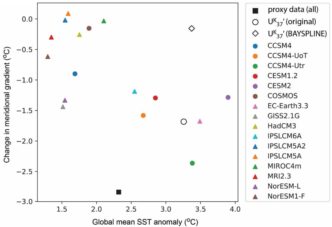
Figure S5: impact of changing high/low latitude bands on meridional SST gradient calculations. The high-latitude box is expanded from >60^\circ\text{N/S} (Figure 3) to include sites between 45\text{--}60^\circ\text{N/S} , and the low-latitude box is restricted to 15^\circ\text{S--}15^\circ\text{N} . This adds a further 4 sites to the original 2 included in the high-latitude box, and removes the possible influence of the Benguela upwelling sites from the low-latitude SST calculations, given data-model mismatch (Figure 4). Although there is minimal change in the proxy data meridional T gradient anomaly ( 2.8^\circ\text{C} here compared to 2.6^\circ\text{C} in Figure 3), the data no longer agree with the PlioMIP2 models.
