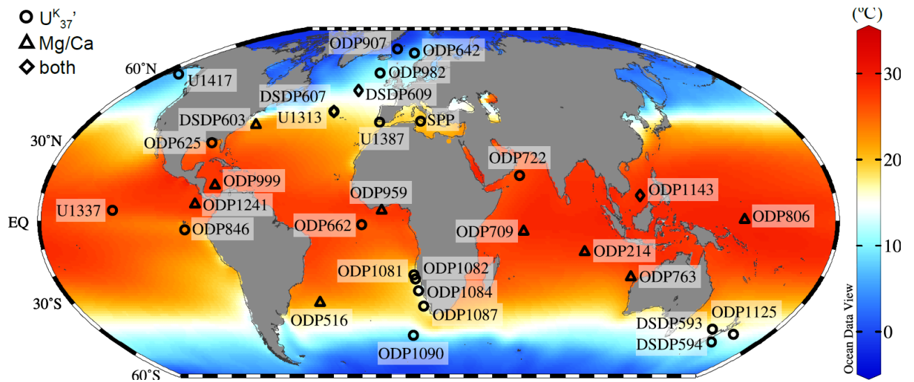
Figure 2: Locations of sites used in the synthesis, overlay on mean annual SST data from the World Ocean Atlas 2018 (Locarnini et al., 2018) . A full list of the data sources and proxies applied per site are available in Table S3 (U K 37 ) and Table S4 (Mg/Ca), and can be accessed at https://pliovar.github.io/km5c.html . The combined PlioVAR proxy data and its sources are also archived at Pangaea: https://doi.pangaea.de/10.1594/PANGAEA.911847 .
