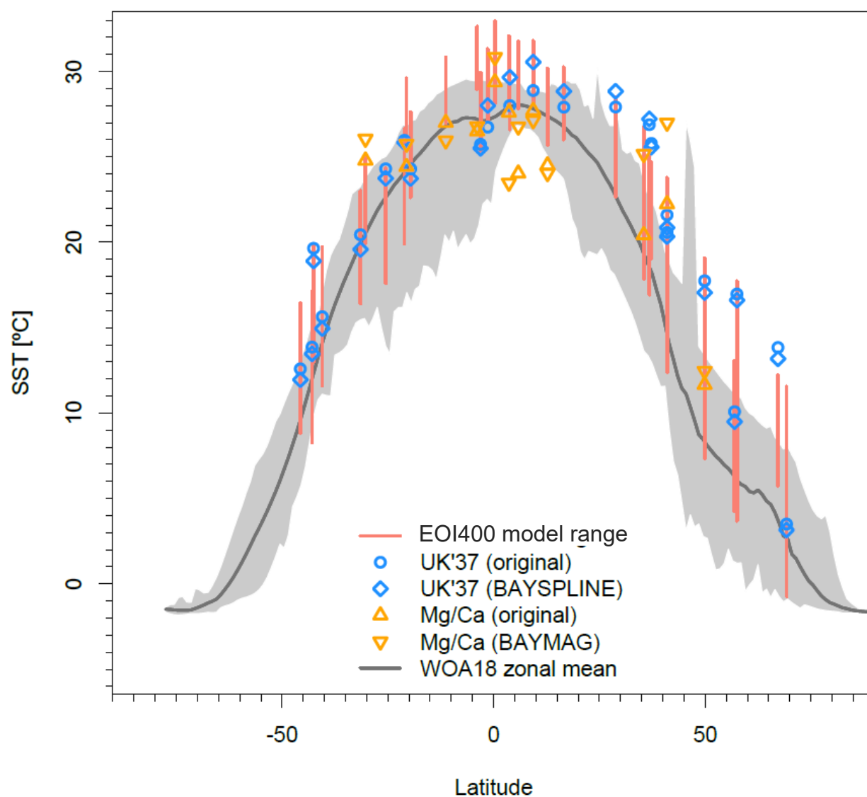
Figure S6: Absolute SSTs for each site, for modern (World Ocean Atlas, 2018 (Boyer et al., 2018)) and for KM5c (proxy data and models as for Figure 4). Grey shading represents the range of SSTs recorded at each latitude for WOA18 (the zonal mean is shown by the solid black line).
