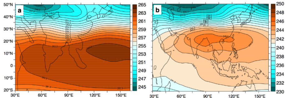
Fig. 2. Figure 8: Air Temperature at 300hPa
