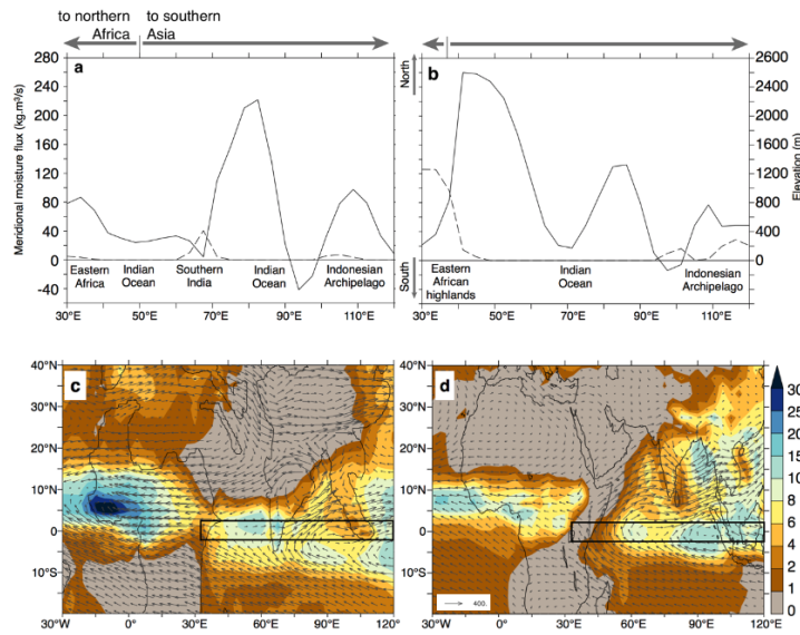
Fig. 1. Figure 5: integrated moisture flux crossing the equator
