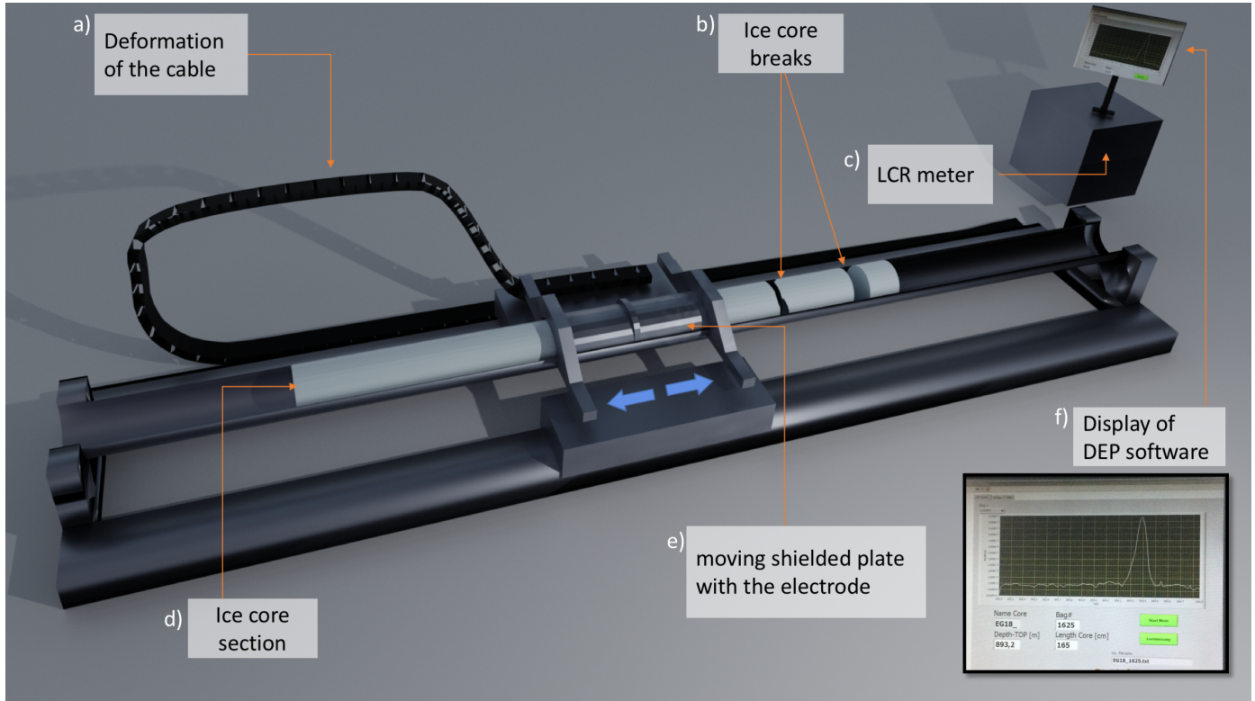
Figure 4. Schematic of the DEP instrument.
