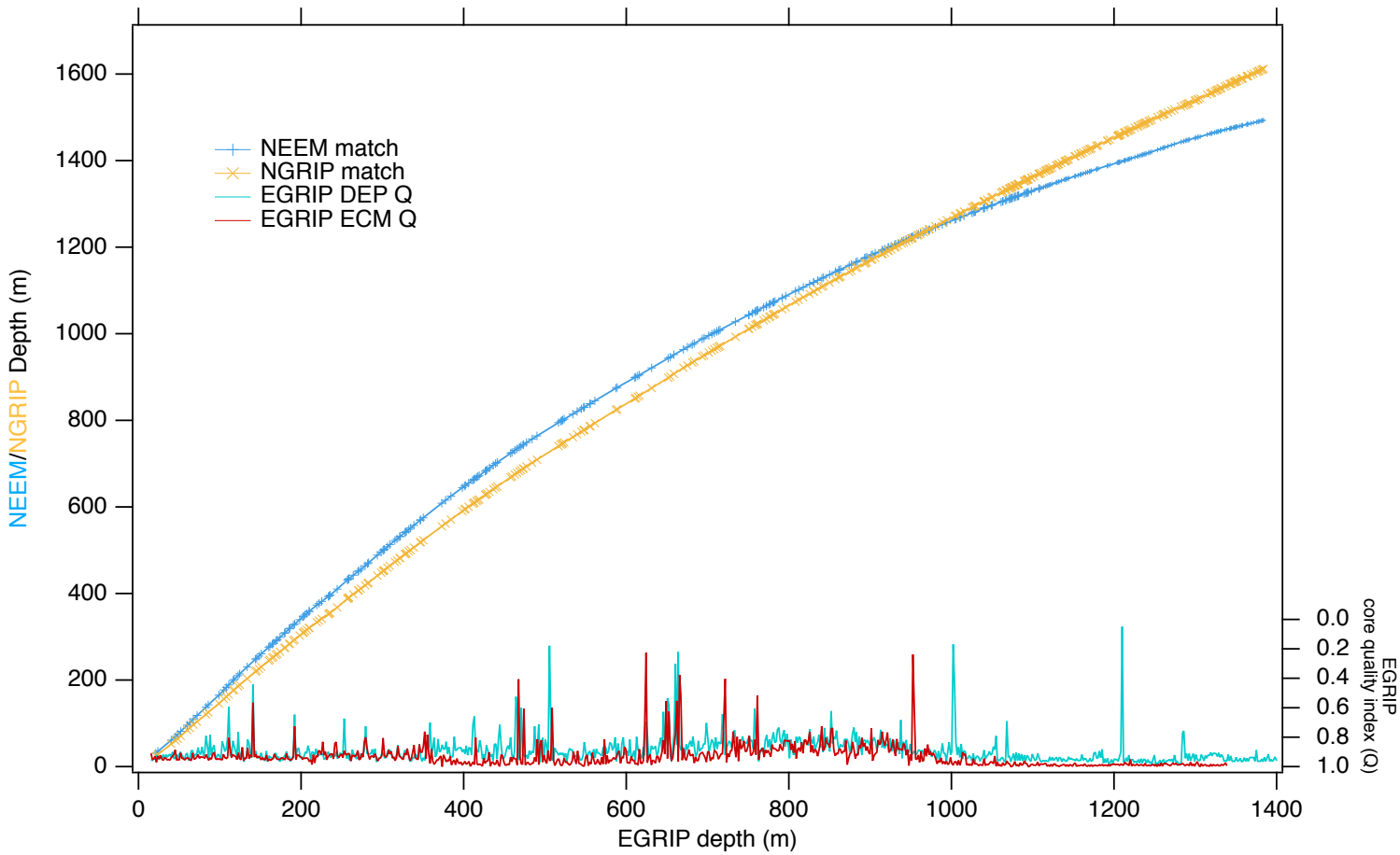
Figure 3. Match points between EGRIP, NEEM (blue) and NGRIP (yellow) ice cores based on the DEP and ECM data sets. The core quality index Q as derived from the validated DEP (blue) and ECM (red) data, respectively.
